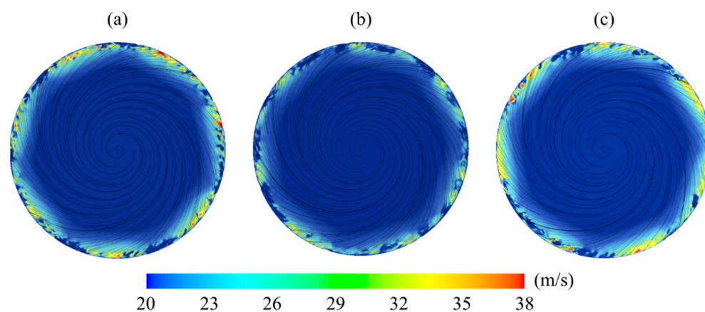
Figure 9. Instantaneous velocity magnitudes |v_R| visualized in Plane 1: (a) Case 1, (b) Case 2, and (c) Case 3.
