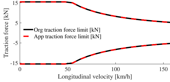
Figure 11: Original and approximated traction force limits of the EM.
