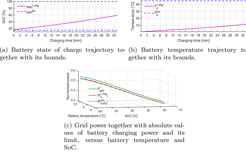
Figure 11: Case 2; optimal trajectories associated with the vehicle's intermediate charging mode at s = 240 km.
