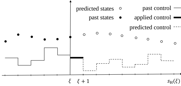
Figure 3.2: Concept of a model predictive controller in discrete domain, where \xi is current instance and s_H is prediction horizon length.
