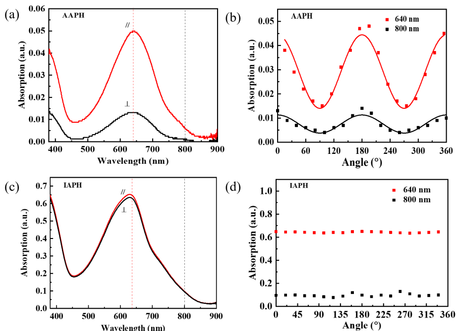
FIG. 2. Polarized UV–Vis absorption spectra of the (a) AAPH and (c) IAPH films. Symbols of // and \perp correspond to the polymer chain orientation parallel and perpendicular to the polarization direction of the incident light. The dependence of the absorption intensity on the \theta for the (b) AAPH and (d) IAPH films at 640 and 800 nm with the fitting lines based on Malus's law.
