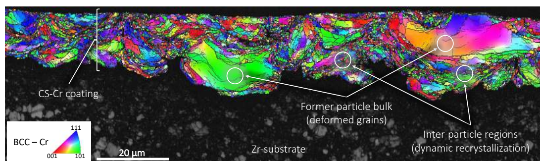
Figure 6-9: EBSD map of CS-Cr coated Zr-cladding (cross-section). Band contrast map is used for the Zr-substrate, IPF colours are plotted for the Cr coating.
