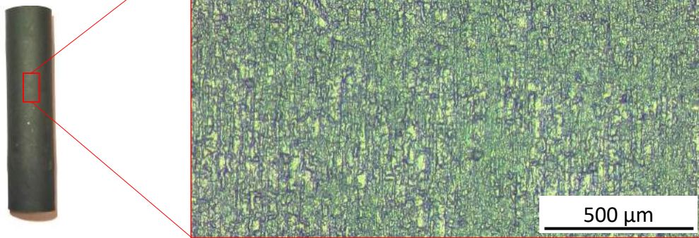
Figure 5-6: Cr coated Zr-cladding oxidised at 1200 °C for 5 min in air.
