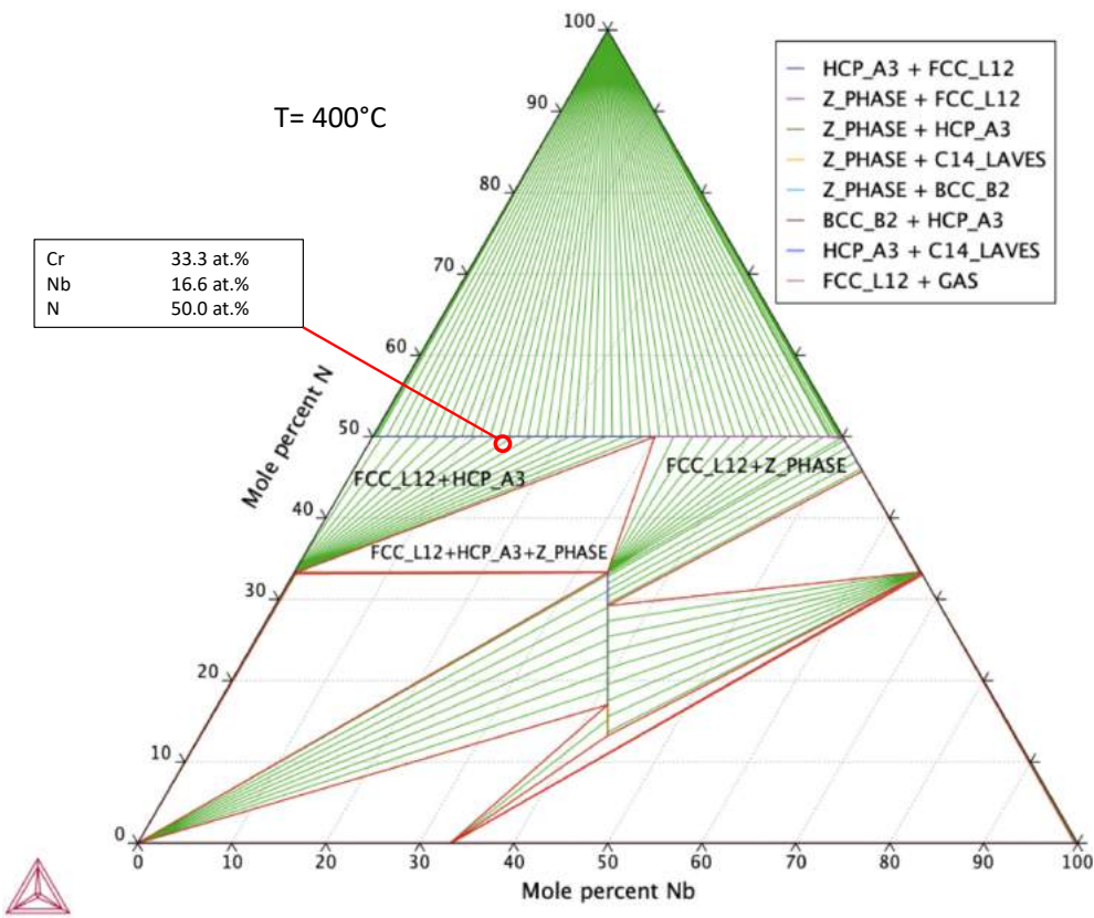
Figure 6-3:Cr-Nb-N ternary phase diagram calculated using ThermoCalc.
