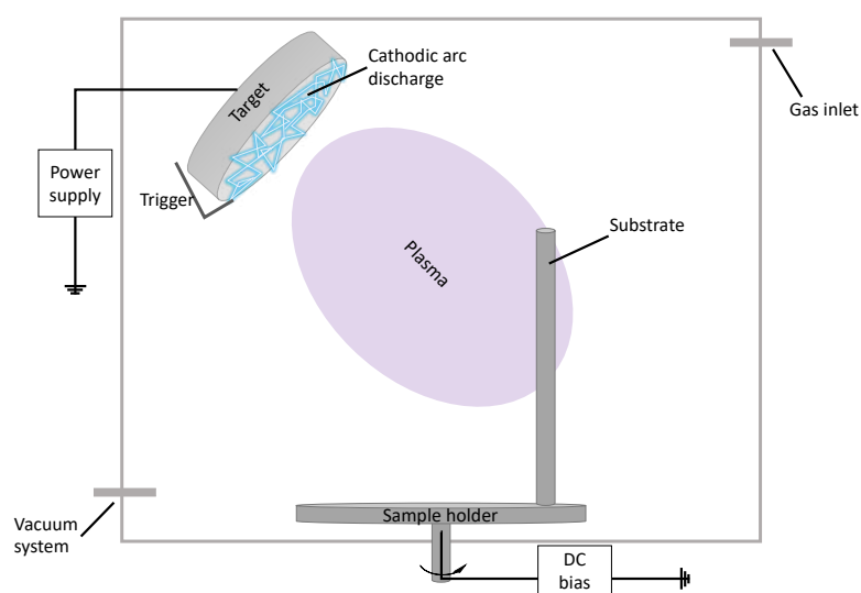
Figure 4-1: Schematic drawing of a cathodic arc evaporation PVD system
