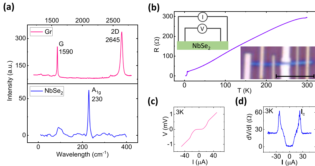
FIG. 2. Materials characteristics of \text{NbSe}_2 and graphene. (a) Raman spectrum of single-layer CVD graphene (top panel) and exfoliated multilayer \text{NbSe}_2 (bottom panel) using 638 nm LASER. (b) Temperature dependence of the longitudinal resistance of multilayer \text{NbSe}_2 flake, where superconducting critical temperature ( T_c ) around 6.8 K is evident. Insets are the four-terminal measurement geometry (top) and device picture (bottom) along with a scale bar of 5 \mu\text{m} . (c) and (d) The four-probe IV measurements and corresponding differential resistance as a function of the bias current in the multilayer \text{NbSe}_2 flake at 3 K.
