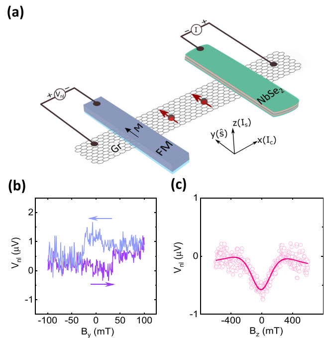
FIG. 3. Charge-spin conversion in \text{NbSe}_2 at room temperature. (a) Schematic illustration of non-local measurement geometry to detect the charge-spin conversion effect in \text{NbSe}_2 by injecting spin current into the graphene spin channel. (b) and (c) The spin-switch and Hanle spin precession measurements for spin injection from \text{NbSe}_2 with B_y and B_z sweeps, respectively. For spin-switch experiments, the up and down magnetic sweep directions are indicated by arrows. The Hanle data are fitted using Eq. (S1). A linear background is subtracted from the data.
