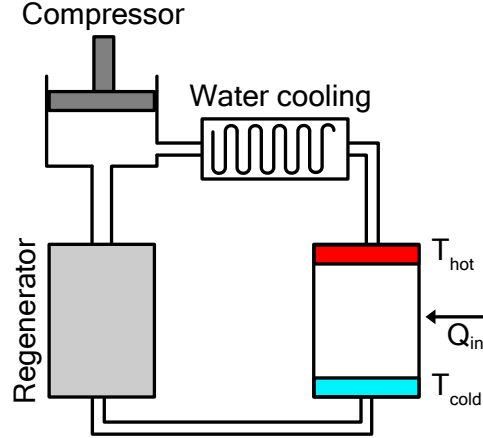
Figure 3.15: Schematic representation of a pulse tube cooler.
