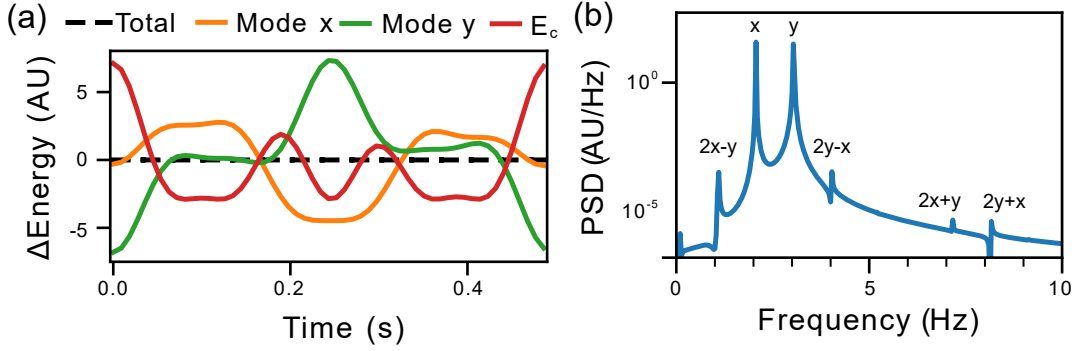
Figure 2.8: (a) Energies of a system with two coupled oscillators with frequencies of 2 Hz (x) and 3 Hz (y). The total energy, that is, the sum of the energy of the modes plus the coupling energy ( E_c ) remains constant, while the energies of the two modes and the energy of the mode coupling vary in time. (b) Power spectrum of the motion of the two oscillators showing a small shift from the uncoupled resonance frequencies (Eq. (2.52)) and additional peaks originating from frequency mixing, i.e. linear combinations of the frequencies of the two modes (Eq. (2.53)).
