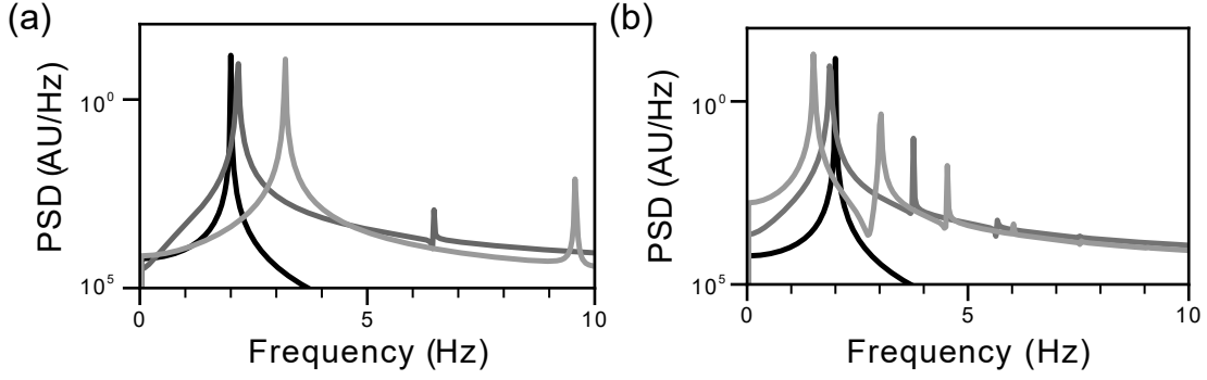
Figure 2.7: Power spectra of the displacement of a 2 Hz oscillator with (a) a quartic (Duffing) and (b) a cubic nonlinearity. Lighter lines indicate larger \alpha and \beta . Note that the fundamental frequency is shifted due to frequency pulling (Eq. (2.44)).
