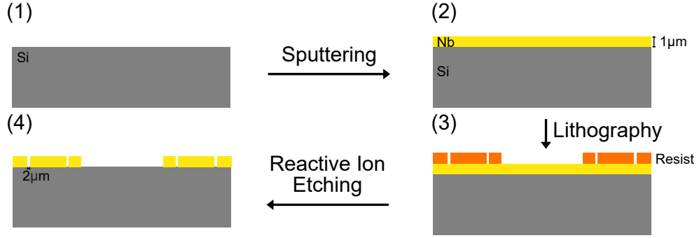
Figure 3.8: Process flow for the fabrication of planar traps. The superconducting coils of the two-chip traps are fabricated in the same way.
