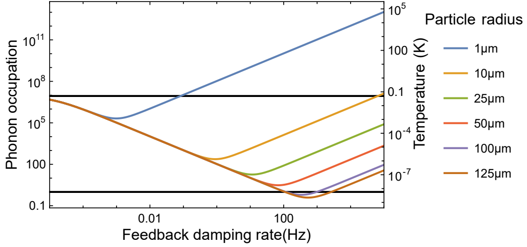
Figure 4.19: Effect of the particle size on the phonon occupation vs feedback cooling rate.
