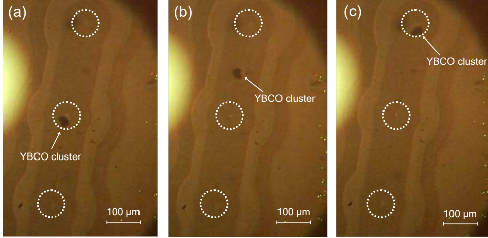
Figure 4.1: Microscope pictures of a planar trap with a YBCO cluster in one of the trap sites (circles). When the trap is on, and we shake the sample with a piezoelectric transducer, the particles slide from one trapping site to another, but they do not levitate. The trapping sites are the areas within the dashed lines.
