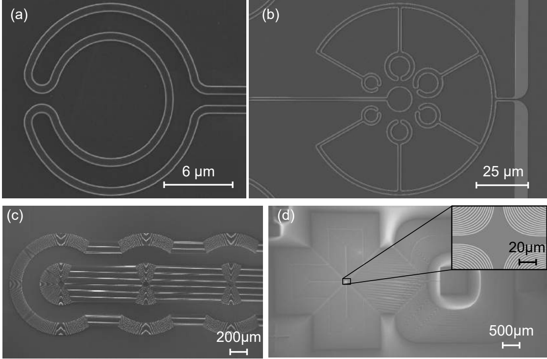
Figure 3.7: SEM pictures of several generations of planar traps in chronological order. The cross-like trap structure in (d) has 500 windings in total.
