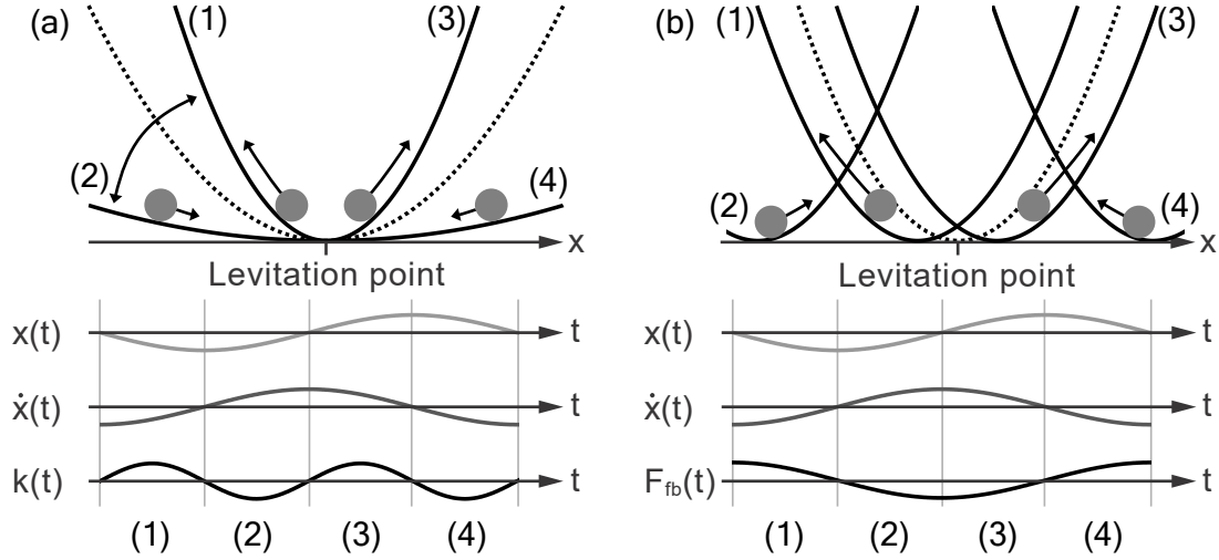
Figure 3.22: Schematic representations of (a) parametric and (b) direct feedback cooling of a levitated particle for a single oscillation cycle. Figures adapted from [118]. The figures show how the potential landscape of the particle in the trap changes over time. The oscillation cycle is divided into four parts, the particle moving away and toward the levitation point from the left (1,2) and from the right (3,4). The dashed line shows the potential well when there is no feedback.
