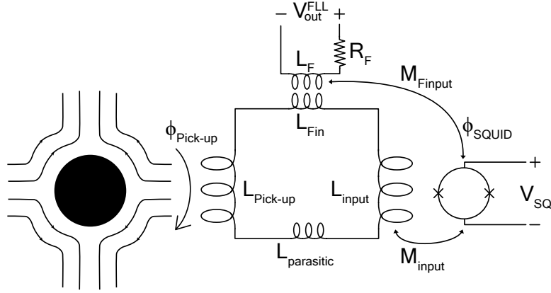
Figure 3.21: Circuit equivalent of the electronics used for the SQUID detection of the levitated particle.
