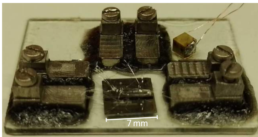
Figure 4.21: Picture of a glass sample holder with Niobium contact pads and titanium screws with a wire-bonded two-chip trap. The cube on the top right is a piezoelectric transducer used to shake the sample if the magnetic force is insufficient to lift the particle.
