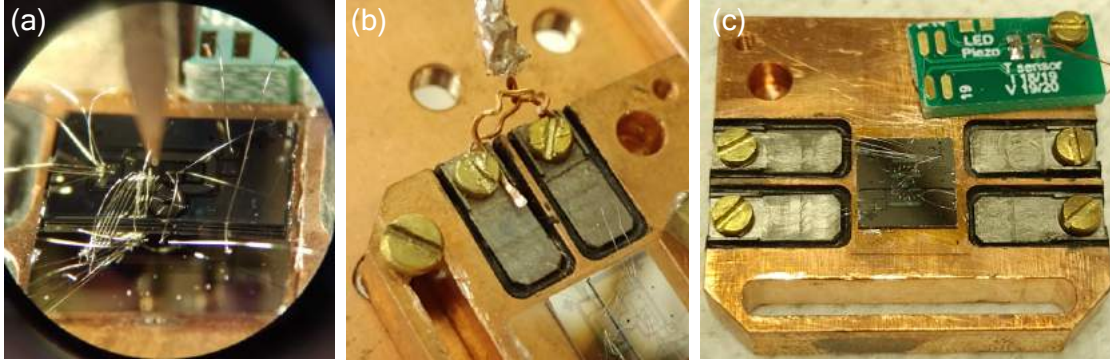
Figure 3.13: Optical microscope pictures of an assembled two-chip trap with the wire bonds between the two chips and the sample holder. (b) Picture of the connections between a two-chip trap and a twisted pair of superconducting wires used to provide electrical current to the coils in the trap. (c) Picture of the copper sample holder with a wire-bonded two-chip trap.
