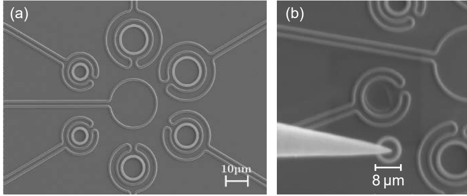
Figure 3.5: SEM pictures of (a) niobium rings fabricated within planar magnetic traps and (b) the same rings being picked and placed with a micromanipulator inside the SEM.
