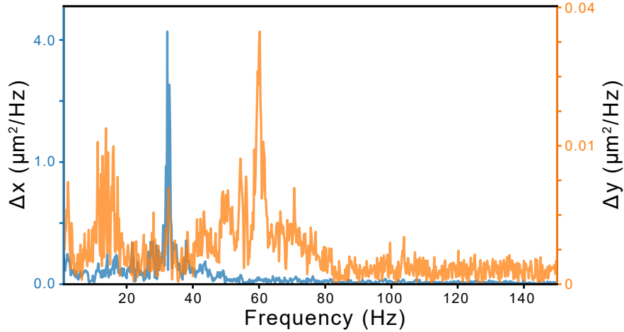
Figure 4.3: Power spectra of the x and y motion of the particle in blue and orange, respectively.
