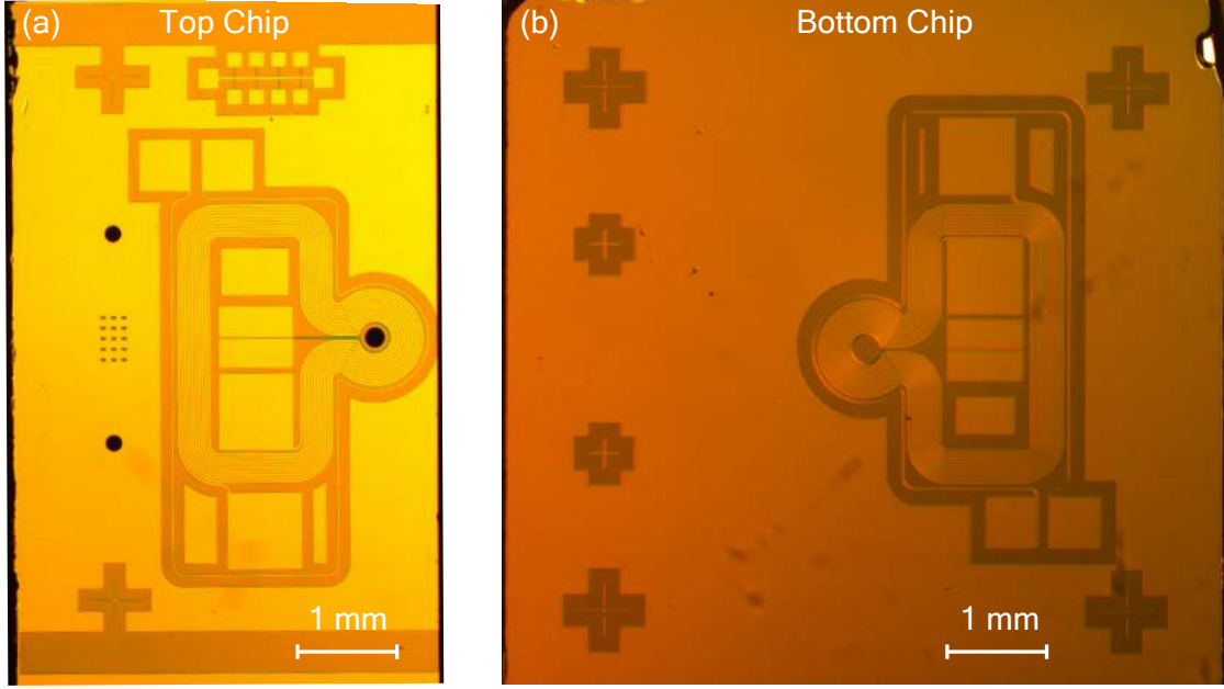
Figure 3.10: Top view of (a) the top chip and (b) the bottom chip of a two-chip trap.
