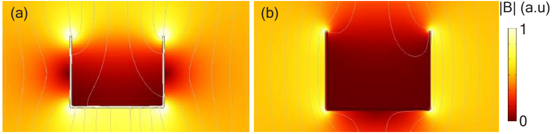
Figure 3.18: Cross-sections of FEM simulations of the magnetic field distribution around (a) a mu-metal basket and (b) a superconducting basket under a vertical homogeneous magnetic field.
