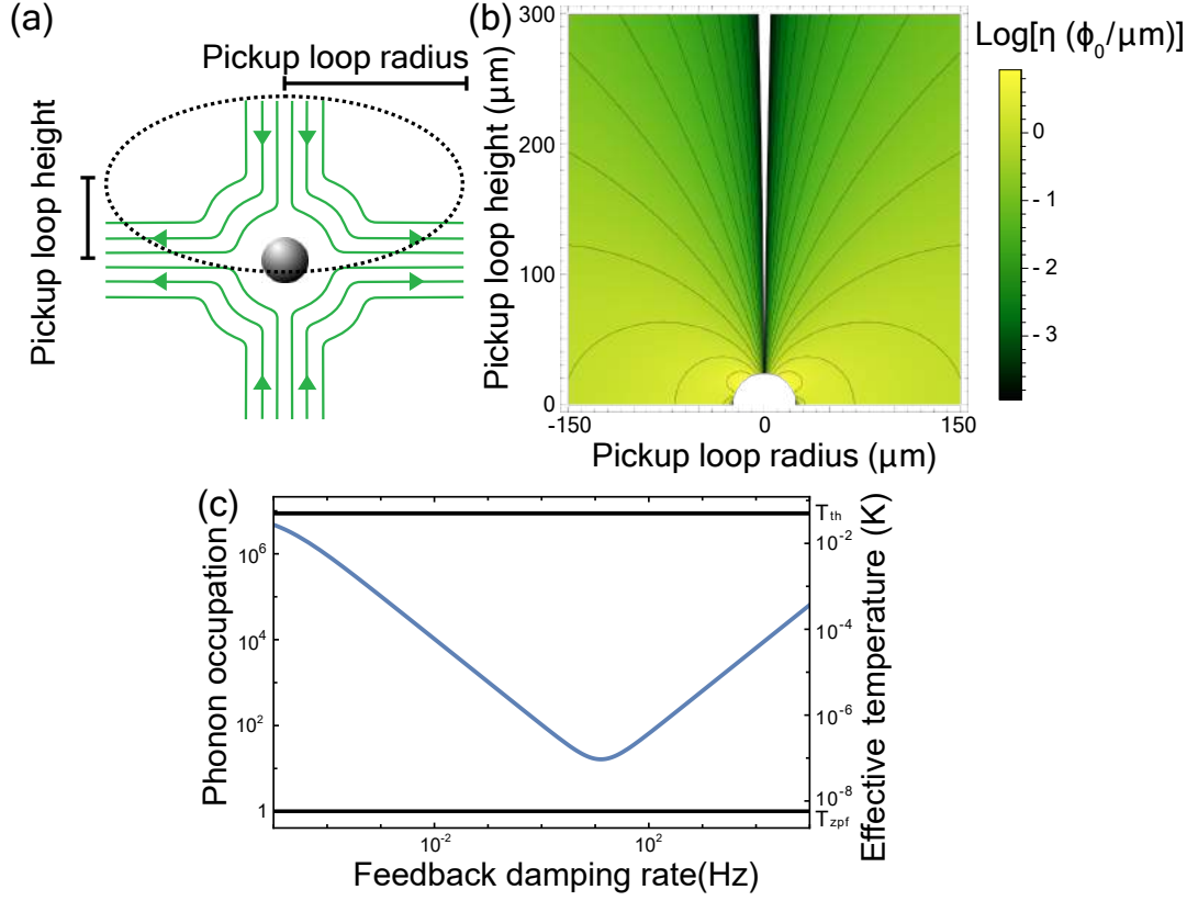
Figure 4.18: (a) Schematic representation of a levitated superconducting particle in a quadrupole field, with a pick-up coil concentric with the particle and the field. (b) Surface plot of the pickup efficiency \eta for different pick-up loop radii and vertical separation with the particle. (c) Phonon occupation vs feedback rate using a pick-up coil with 100 windings, with a pitch of 1 \mu\text{m} and an inner radius of 50 \mu\text{m} , to cool down a levitated particle with Q=10^7 using a SQUID magnetometer with a sensitivity limited by its intrinsic noise and with the same input inductance as the pick-up loop.
