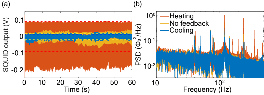
Figure 4.11: (a) Amplitude of the SQUID signal when the COM motion of the levitated particle in the z direction is heated, provided no feedback, and when it is cooled. (b) The corresponding power spectra of the time traces in (a), showing the difference in peak height and the frequency shifts, caused by nonlinearities of the magnetic trap and coupling between the modes.
