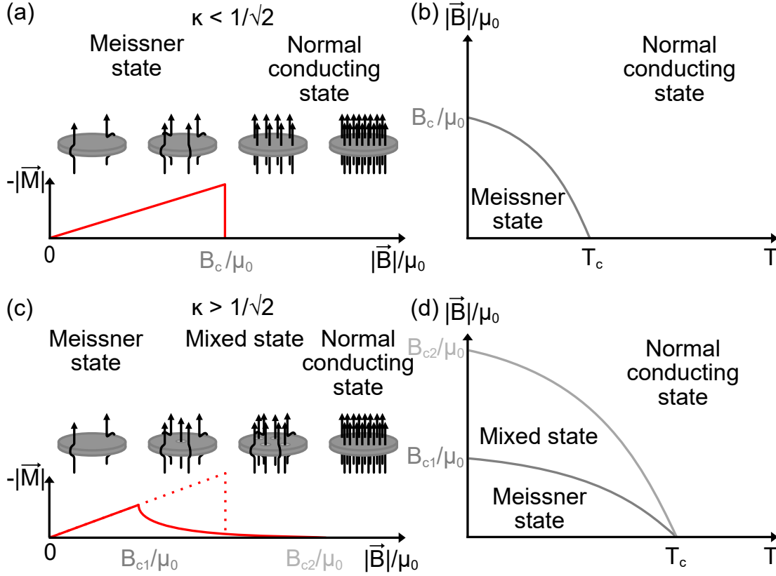
Figure 2.2: Type I and Type II superconductivity. (a)-(c) Magnetization curves and (b)-(d) phase diagrams of type I and type II superconductors, illustrating field expulsion, field penetration by flux vortices, and the temperature dependence of B_c , B_{c1} , and B_{c2} , respectively.
