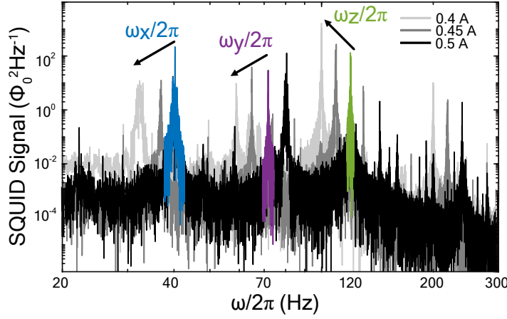
Figure 4.5: Spectra of three SQUID time traces for different currents running in the chip trap. The black curve shows the same power spectrum as Fig. 4.4(b) with the fundamental frequencies colored in the same way, and the lighter curves show the trap frequencies decreasing for descending trap currents.
