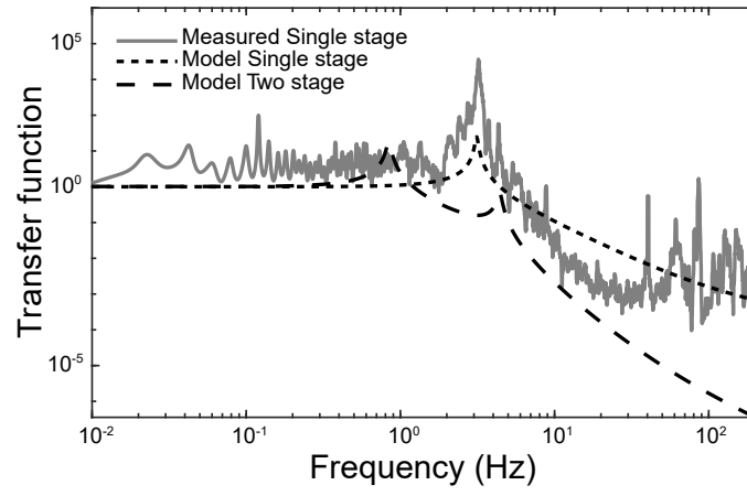
Figure 4.24: Transfer functions of the single-stage vibration isolation as measured and predicted by the model and of the two-stage system that will be employed in future experiments.
