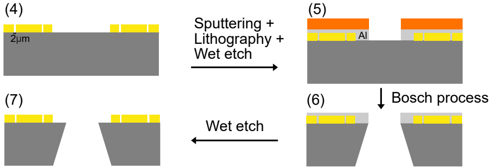
Figure 3.9: Process flow for the fabrication of the holes in the top chips of the magnetic two-chip traps. The fabrication starts from step (4) in Fig. 3.8.
