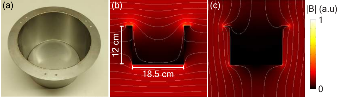
Figure 4.22: (a) Niobium cylinder with one end closed and one end open, meant to encase the whole sample stage. Magnetic field distributions around the cylinder when under (b) a horizontal and (c) a vertical magnetic field. The shielding factor is calculated 1 cm away from the bottom of the cylinder, where the sample would be.
