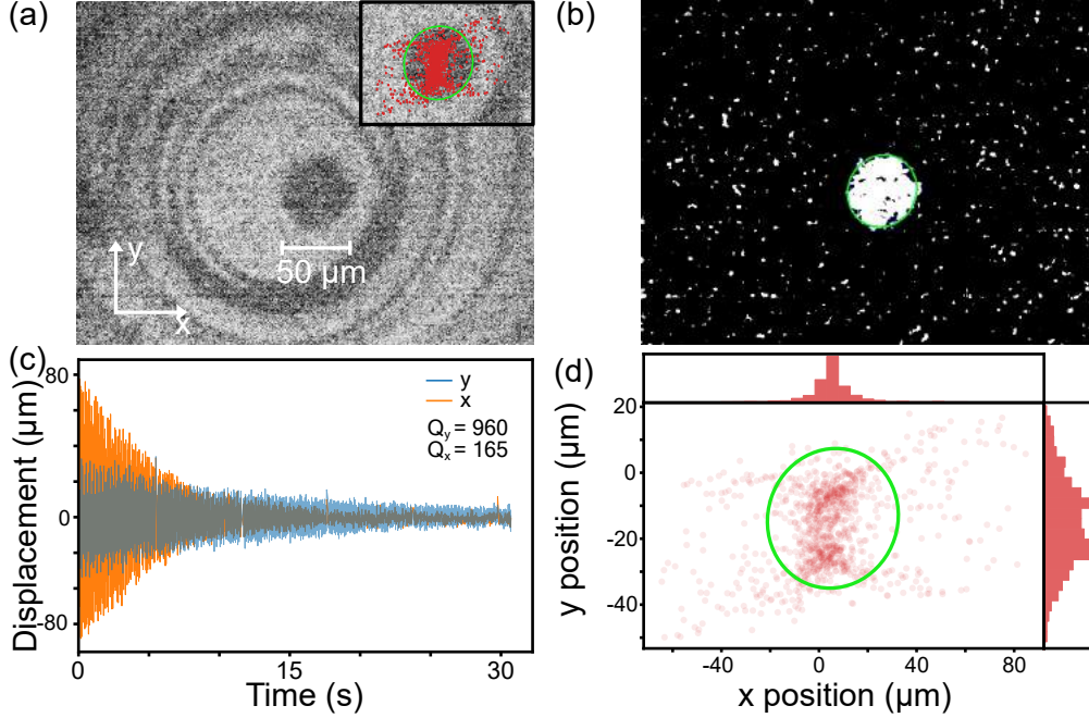
Figure 4.2: (a) Top view of the levitating particle (black circle) inside the magnetic trap. The concentric circles are the top and bottom coils and the hole in the top chip. The inset in the top right shows the fitted particle contour in green and the particle positions (red) measured over the duration of the video. (b) Particle contour (green) resulting from processing (a) with a particle tracking algorithm that fits an ellipse (green) to the perimeter of the particle. (c) Ringdown of the particle motion in the x and y directions. (d) Density plot of the measured particle positions in the trap, where the origin of the coordinate system is the center of the frame in (a) and the green contour is the one shown in (b).
