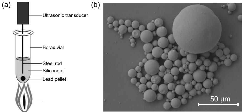
Figure 3.6: (a) Schematic representation of the ultrasonic cavitation setup used to produce lead microspheres (adapted from [108]) and (b) scanning electron microscope picture of the resulting lead microspheres.
