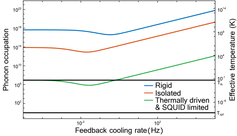
Figure 4.17: Phonon occupation and effective temperature of the z COM mode as a function of the feedback cooling rate for the experiment when attached to the fridge rigidly (blue), with vibration isolation (red) and in the hypothetical case of thermally driven COM motion and sensitivity limited by the SQUID noise floor (green). The solid black lines indicate an effective temperature of 50 mK (top) and the effective temperature of the motion when driven by zero-point fluctuations (bottom). The quality factors used for each case are 10^3 (blue), 10^5 (red), and 10^7 (green).
