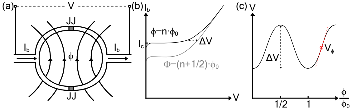
Figure 2.5: (a) Schematic representation of a DC-SQUID. (b) I-V curve of a DC-SQUID for one and half a magnetic flux quantum threading the loop. (c) V- \phi curve of a DC-SQUID with a current bias above the critical current of the SQUID.
