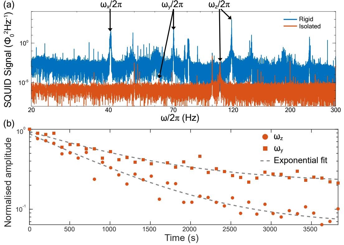
Figure 4.10: (a) Effect of vibration isolation in the SQUID signal, showing a decrease in the noise floor as well as in the particle motional amplitude when comparing a 24\text{ }\mu\text{m} radius sphere levitated on a setup rigidly attached to the mixing stage and a 31\text{ }\mu\text{m} radius sphere levitated on the vibration isolated stage, using the same magnetic trap. Note that the \omega_x peak is not found in the measurement with a vibration-isolated stage. (b) Ring-down measurements of the \omega_y and \omega_z peaks of the 31\text{ }\mu\text{m} radius sphere levitated on the vibration isolated stage.
