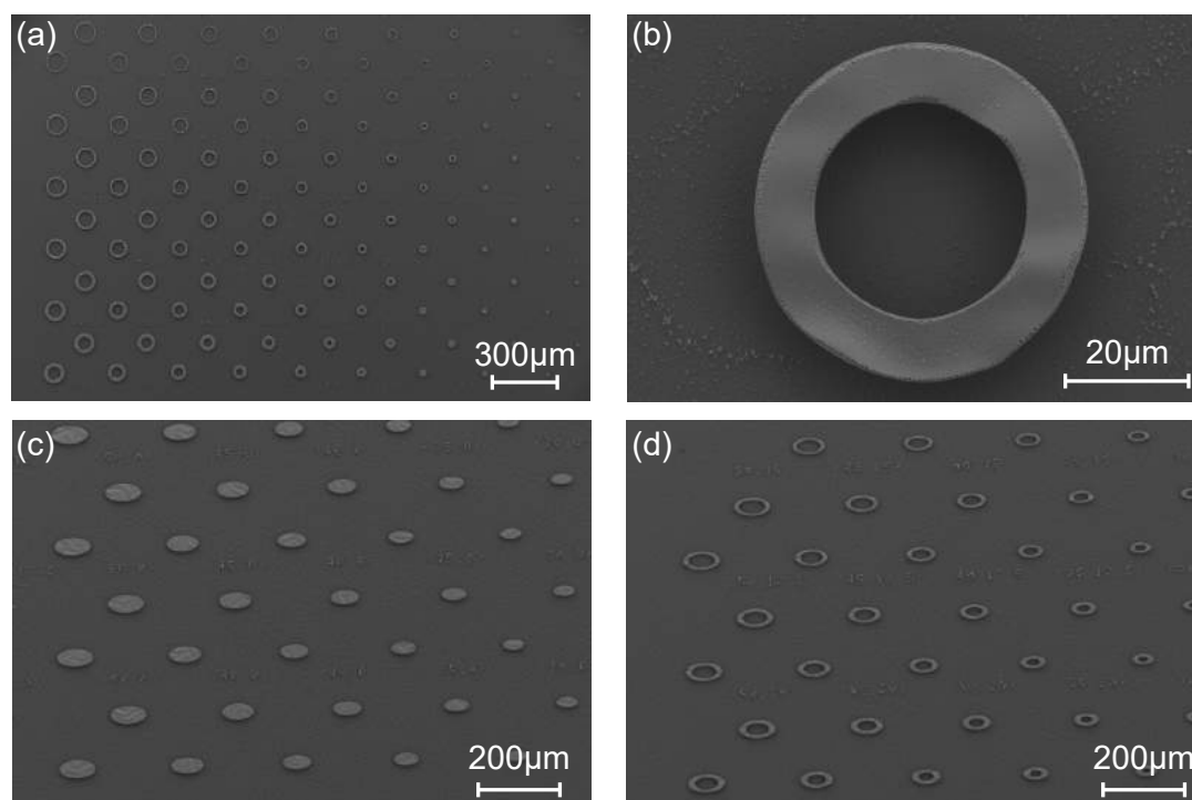
Figure 3.4: Scanning electron microscope (SEM) pictures of arrays of planar niobium particles of different sizes with the shape of (a) circular rings, (c) ellipses, and (d) elliptical rings. (b) Magnified view of a circular niobium ring. All the particles are 1 μm thick. All pictures have been taken using a top view detector, that is to say, pictures (c) and (d) do not show circular particles viewed at an angle, but actually elliptically shaped particles.
