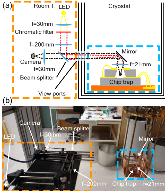
Figure 3.20: (a) Schematic of the optical detection setup, showing both the illumination and imaging paths of the light in red and black, respectively. Drawing not to scale. (b) Picture of the setup with the cryostat open.
