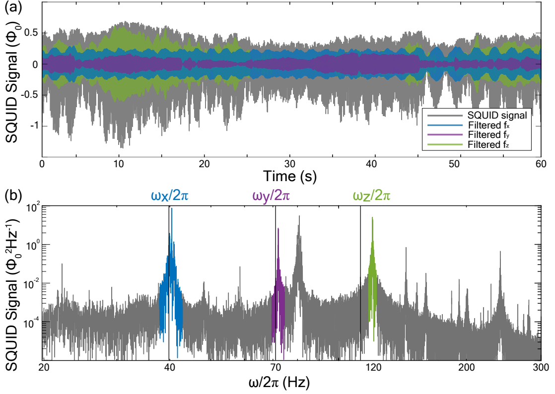
Figure 4.4: (a) Time trace of the SQUID magnetometer calibrated to flux quanta. The gray curve shows the output of the SQUID electronics, and the colored curves show the same data filtered around the particle trap frequencies. (b) Power spectrum of the curves in (a), where the vertical lines show the frequencies predicted by FEM simulations (taken from Paper C).
