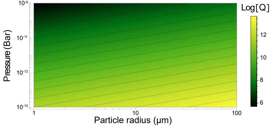
Figure 4.15: Quality factor due to gas collisions for a spherical particle at different pressures and particle radii.
