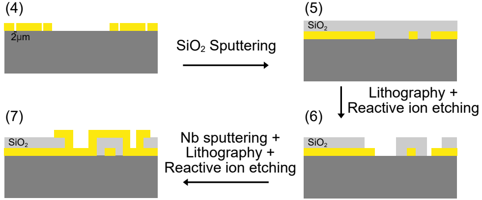
Figure 3.11: Process flow for the fabrication of vias on a planar coil. The process starts after step (4) in Fig. 3.8.
