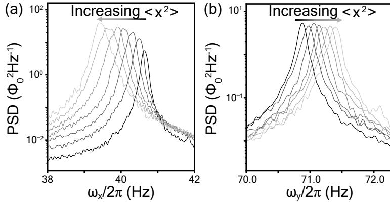
Figure 4.6: Frequency shift in (a) \omega_x and (b) \omega_y due to changes in the x-mode amplitude, exemplifying mode nonlinearities and mode coupling in the modes of the levitated particle, respectively (taken from Paper C).
