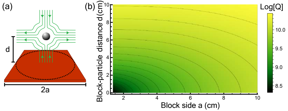
Figure 4.12: (a) Schematic representation of a particle levitated in a quadrupole field above a copper block, within which the oscillating magnetic flux is calculated. (b) Quality factor due to eddy current damping for a piece of copper with an increasingly large lateral dimension l and distance d for a given thickness h = 5 mm.
