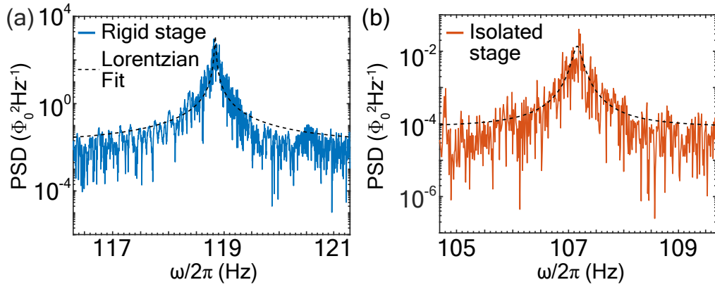
Figure 4.16: (a) SQUID signal of a 24 \mu\text{m} radius lead particle levitated on a sample stage that is rigidly fixed to the cryostat. (b) SQUID signal of a 31 \mu\text{m} radius lead particle levitated on a sample stage that is mechanically isolated from the cryostat by an elastic pendulum. The data is taken from Fig. 4.10(a).
