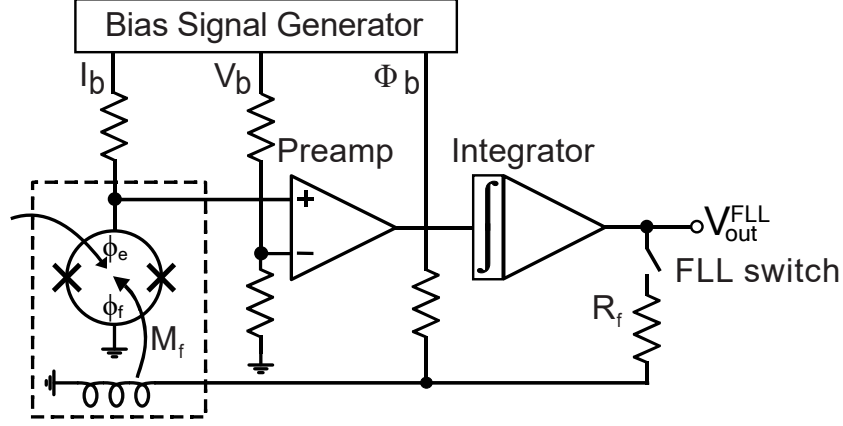
Figure 2.6: Circuit equivalent of the DC-SQUID control electronics, including the flux-locked loop (FLL) electronics. The elements inside the dashed line are cooled to cryogenic temperatures. Figure adapted from [93].
