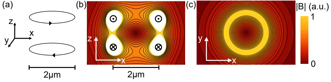
Figure 3.1: (a) Schematic representation of two current loops and (b,c) cut planes of their corresponding magnetic field distribution calculated with Eqs. (3.2) to (3.4).
