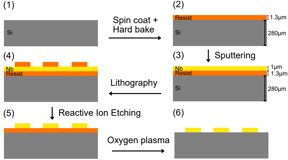
Figure 3.3: Process flow for the fabrication of planar niobium particles.
