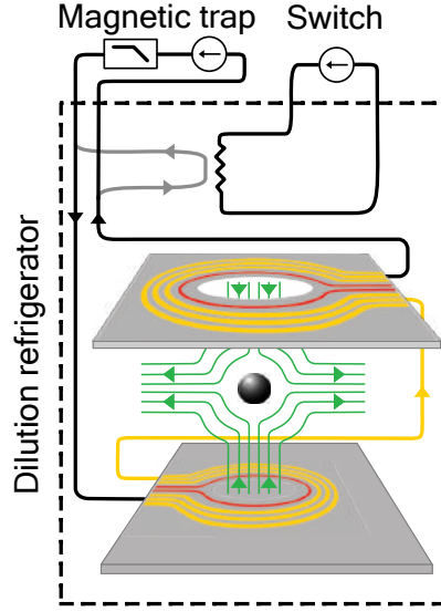
Figure 4.23: Schematic view of the persistent current switch, consisting of a resistor in thermal contact with the superconducting short (gray) in the high current line that feeds current to the magnetic trap, as implemented in our experimental setup. Current flows through the superconducting short only when it has been trapped by the persistent current switch.
