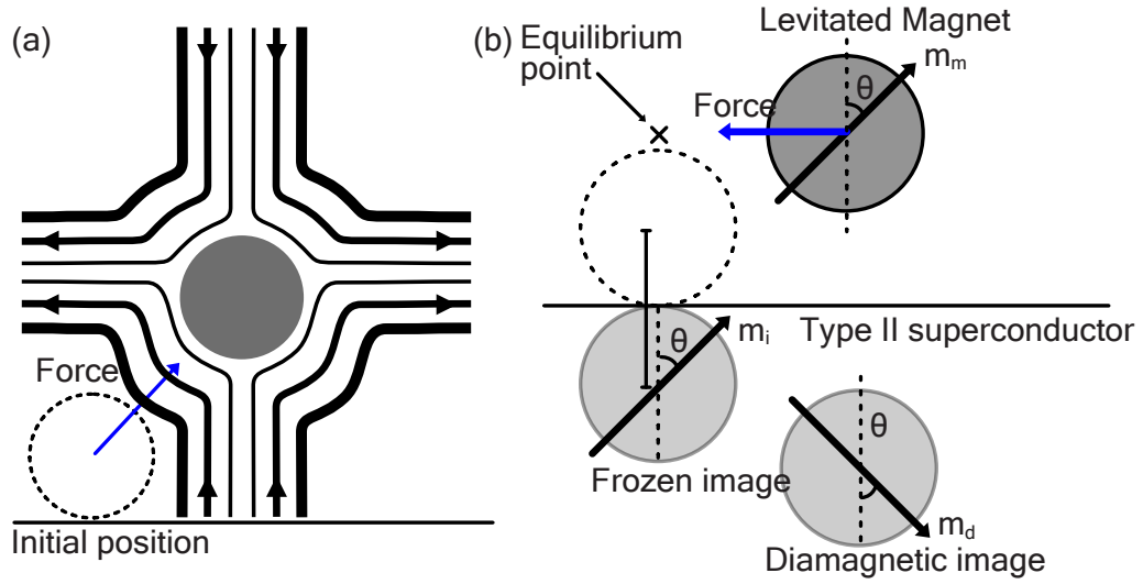
Figure 2.3: (a) A superconductor levitated with a quadrupole magnetic field using Meissner state repulsion. The superconductor is repelled by the high field regions (thicker lines) and is pushed into the center of the quadrupole field, where the magnetic field is minimum. Note that the particle is displaced downward from the quadrupole center due to the force of gravity. (b) Schematic of a magnet levitated on a type II superconductor. The superconductor produces two images of the levitated magnet. The frozen image is a consequence of flux trapping and the diamagnetic image is a consequence of Meissner state repulsion. The dashed line shows the initial resting position of the magnet.
