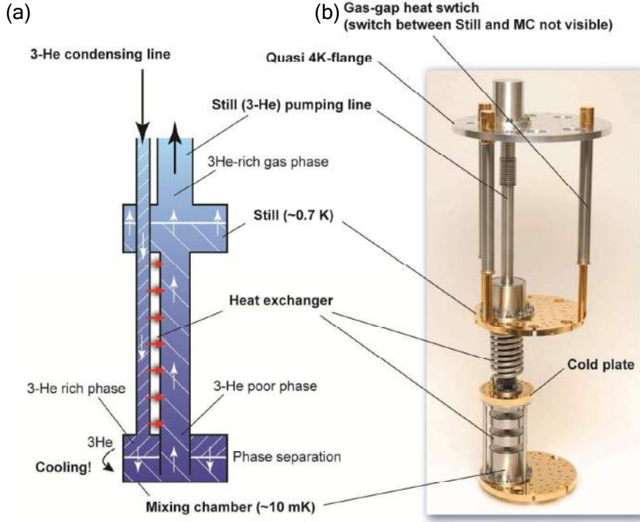
Figure 3.17: (a) Schematic view of a dilution unit and (b) a picture of a dilution unit of a Bluefors dilution refrigerator (figure from Bluefors User Manual).
