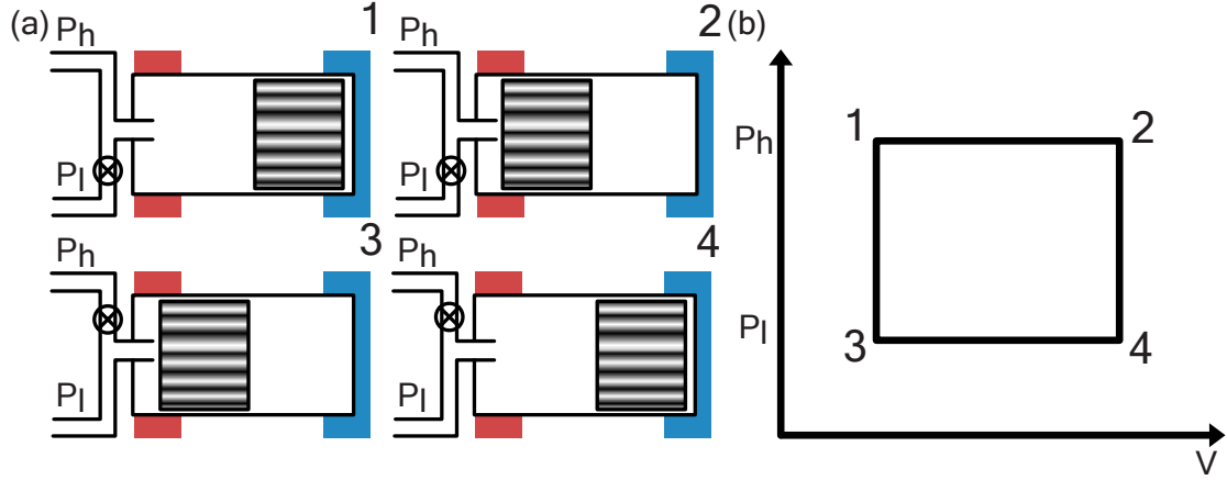
Figure 3.14: (a) Steps of the GM cycle illustrated in the GM cooler and (b) in a P-V diagram.
