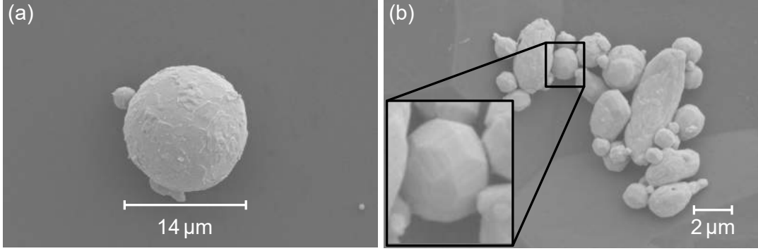
Figure 4.20: Scanning electron microscope pictures of lead microparticles (a) before and (b) after being heated at 300 °C in a nitrogen atmosphere. Note that the crystallographic facets are observable on the surface of the particles after heating, especially for the smaller particles (in the inset).
