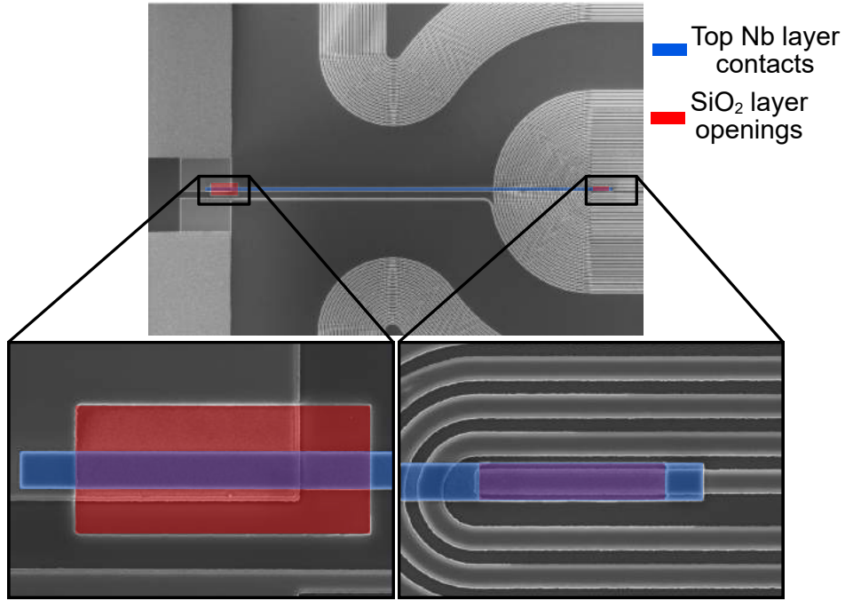
Figure 3.12: SEM pictures of a planar multiwinding coil. The entirety of the chip is covered in silicon dioxide, except the areas marked in red and blue. The red area indicates where the silicon dioxide has been etched away, and the blue area indicates the second layer of niobium, which has been patterned into a wire that connects the wire-bonding pad (big square on the left) and the contact inside the multiwinding coil (inset on the right). The insets show larger magnification pictures of the vias.
