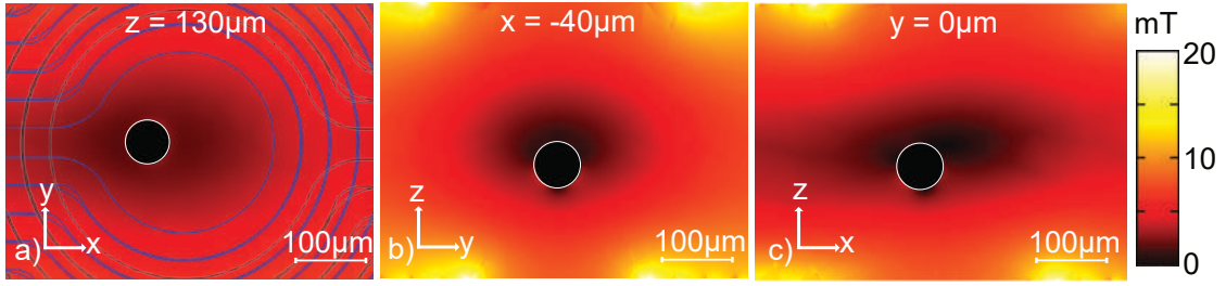
Figure 3.2: Cut planes of the magnetic field distribution of a superconducting sphere levitated inside a magnetic chip trap with 0.5 A running in the coils. The zero of the coordinate system is the center of the bottom coil.
