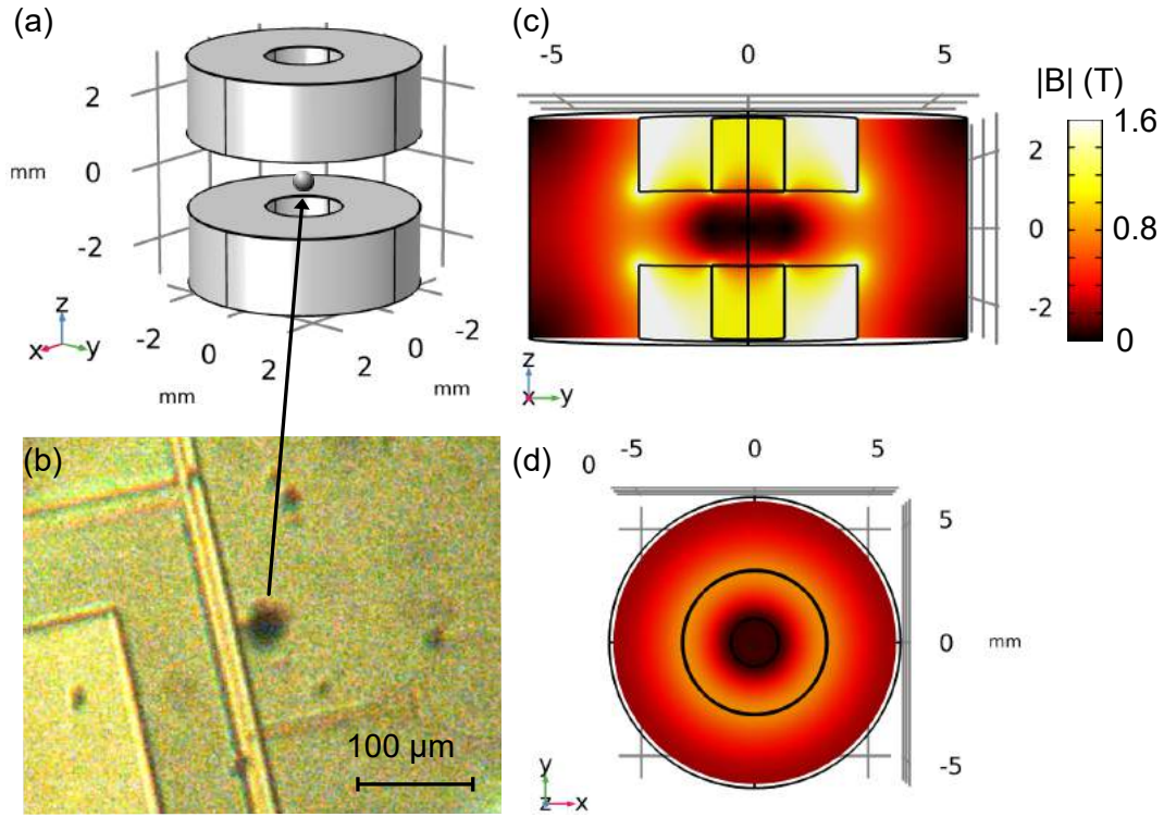
Figure 6.1: (a) Schematic representation of the magnet trap, showing two millimeter-sized ring magnets with opposing magnetization. (b) A YBCO cluster levitating inside a magnet trap, on top of a chip with niobium structures that acts only as a carrier for the particle. Magnetic field distributions of the (c) vertical and (d) horizontal cut planes at the levitation point between the magnets.
