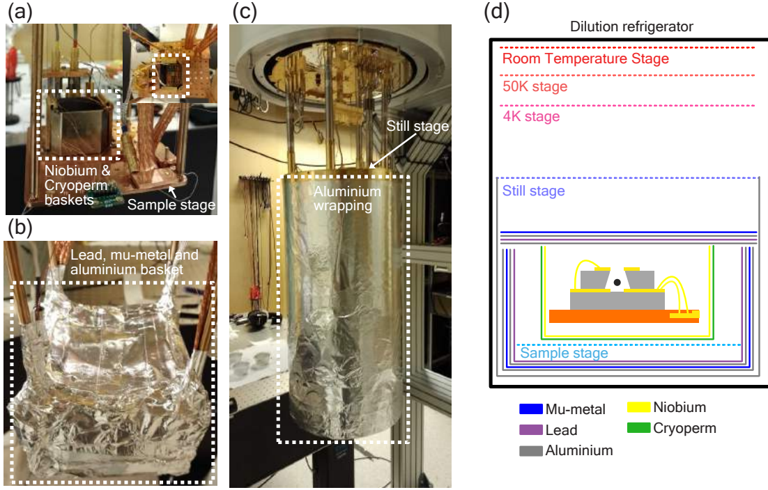
Figure 3.19: Magnetic shields shown from innermost to outermost, highlighted within the white dashed lines. (a) The innermost magnetic shield made of a Niobium basket inside a cryoperm basket on the sample stage of the dilution refrigerator. The inset on the top right shows a top view of the sample stage with a sample inside the magnetic shield basket. (b) Intermediate magnetic shield made of layers of lead, mu-metal, and aluminium that wraps around the entire sample stage. (c) Outermost magnetic shield made of aluminium foil wrapping the entire still can. (d) Schematic representation of all the magnetic shielding in the dilution refrigerator, not to scale.
