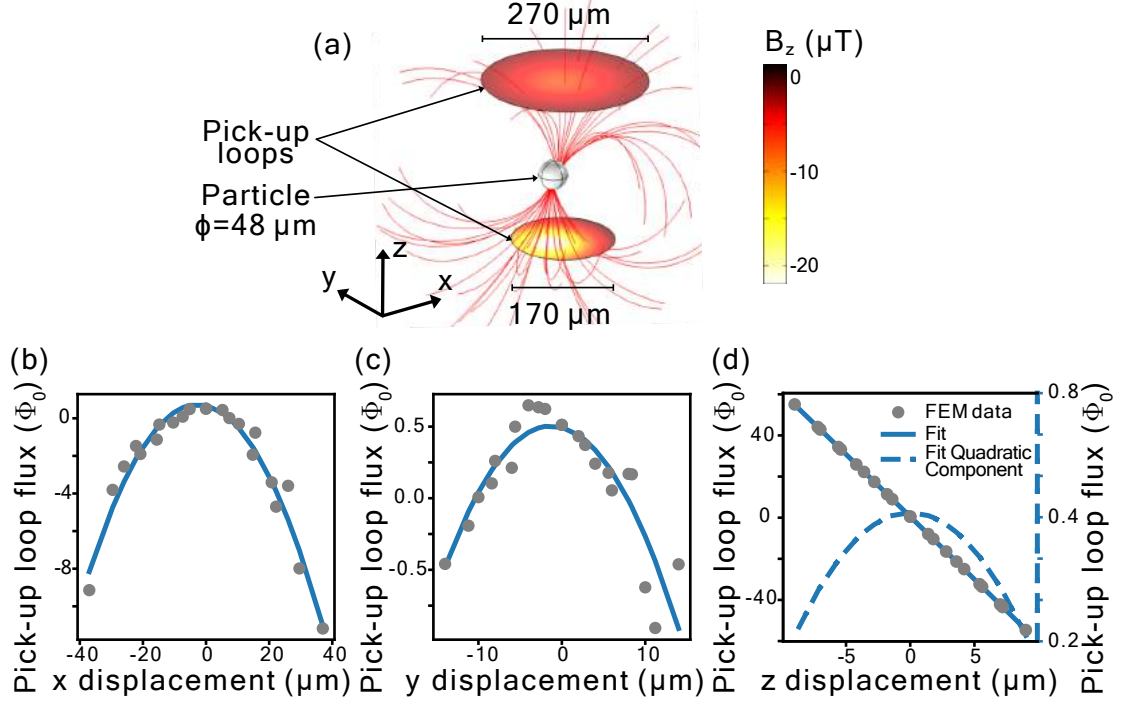
Figure 4.8: (a) FEM simulation of the back action field of a superconducting sphere inside a magnetic quadrupole trap between two pick-up loops. The field lines are shown as red lines, and the vertical component of the magnetic field is potted in the areas contained within the pick-up loops. Magnetic flux in the top and bottom loops induced by the particle displacement in the (b) x , (c) y , and (d) z directions (taken from Paper C).
