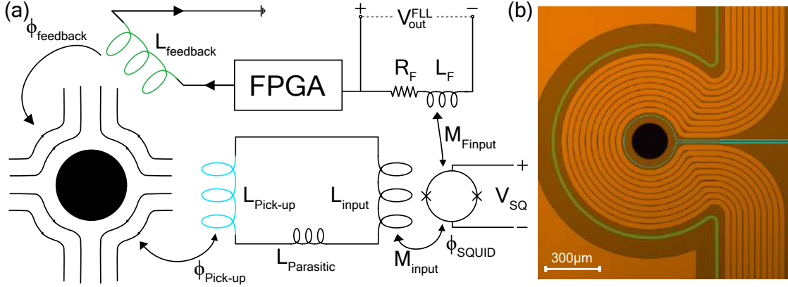
Figure 3.23: (a) Schematic representation of the feedback circuit used in the experiments. The SQUID is assumed to be operated in FLL. (b) Colored optical microscope picture of the top chip, showing the trap coil (orange), the pickup coil (cyan), and the feedback coil (green) as colored in (a).
