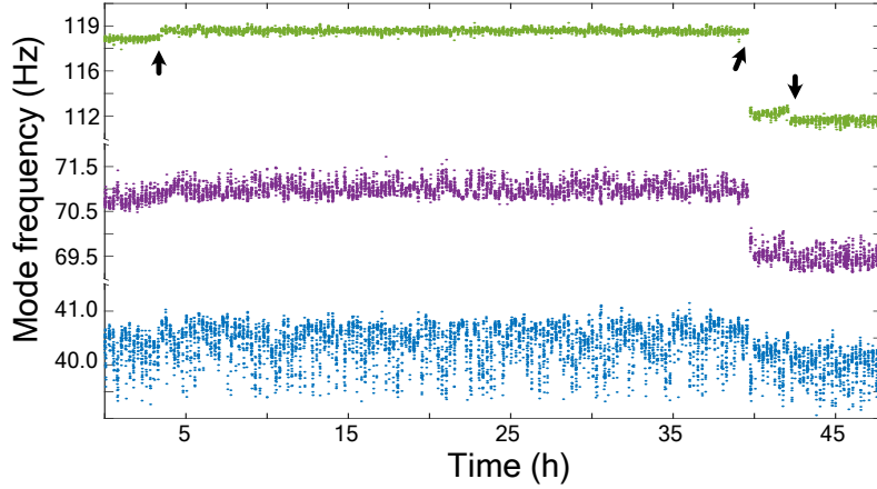
Figure 4.13: Particle frequencies measured of a 48 h time period. The arrows indicate the times when discrete frequency jumps occur (taken from paper C).
