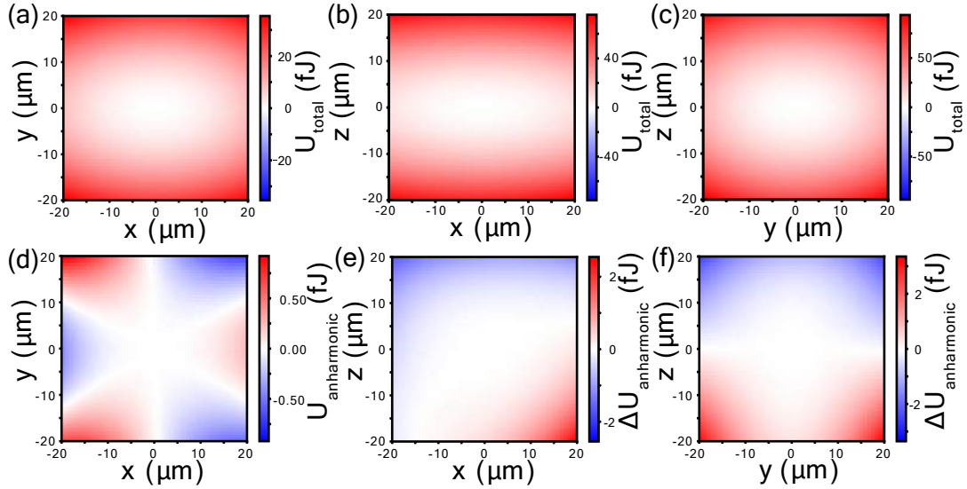
Figure 4.7: Model of the potential energy landscape of a 48\text{ }\mu\text{m} diameter particle in the chip trap. (a-c) 2D slices of the total potential energy landscape of the particle in the trap. (d-f) Anharmonic contributions to the potential energy landscape (adapted from Paper C).
