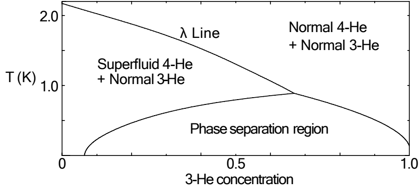
Figure 3.16: Phase diagram of 4-He/3-He mixture, adapted from [113].
