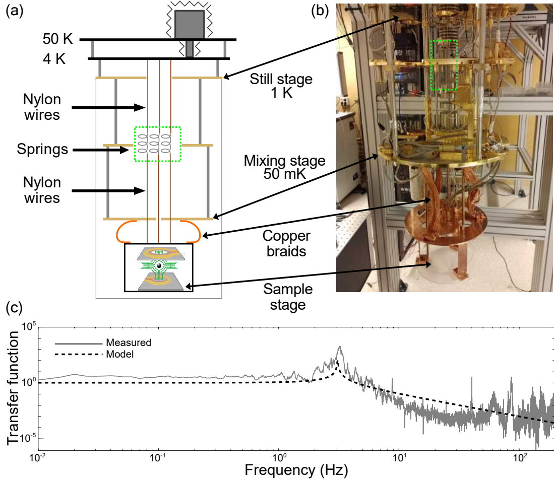
Figure 4.9: (a) Schematic representation and (b) picture of the sample stage with vibration isolation, which is hanging from three elastic pendula attached to the 4 K stage for mechanical isolation, as well as from unbraided copper braids attached to the mixing stage for thermalization. (c) The transfer function of the vertical displacement for the vibration isolation stage with respect to the 4 K stage is measured with a geophone in gray and predicted by the model in a dashed black line.
