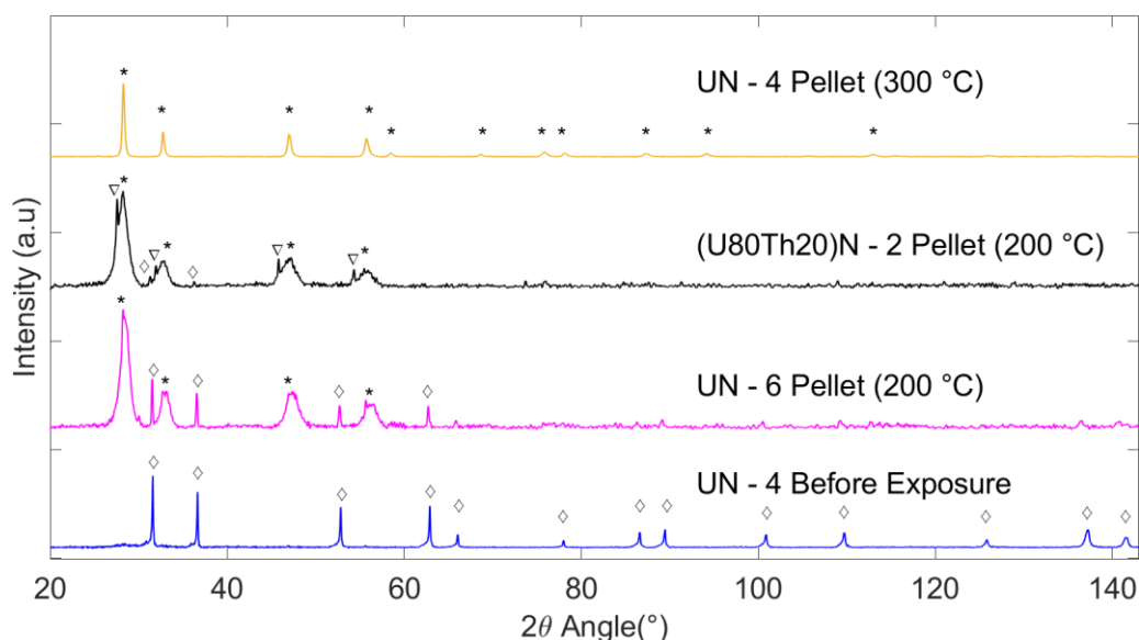
Figure 6.11. X-Ray diffractograms for powders collected after pellet disintegration in the corrosion testing compared to the UN pellet before interaction, where UN(◇), UO_2 (*), or ThO_2 (▽) peaks were identified.
