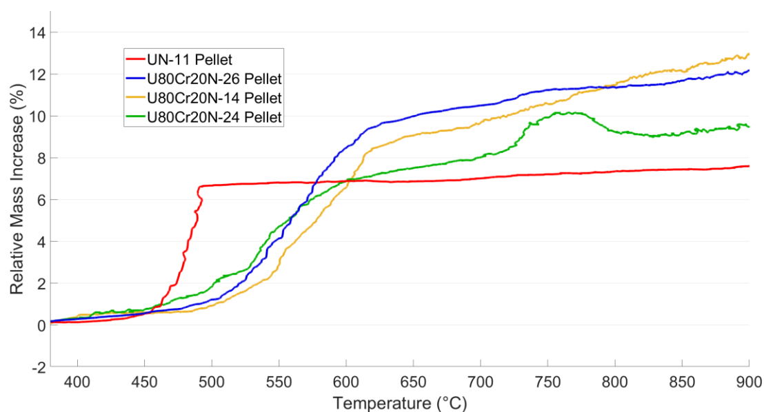
Figure 6.26. Steam TGA curves for hydrolysis of uranium nitride and chromium-doped uranium nitride pellets from Batch B.
