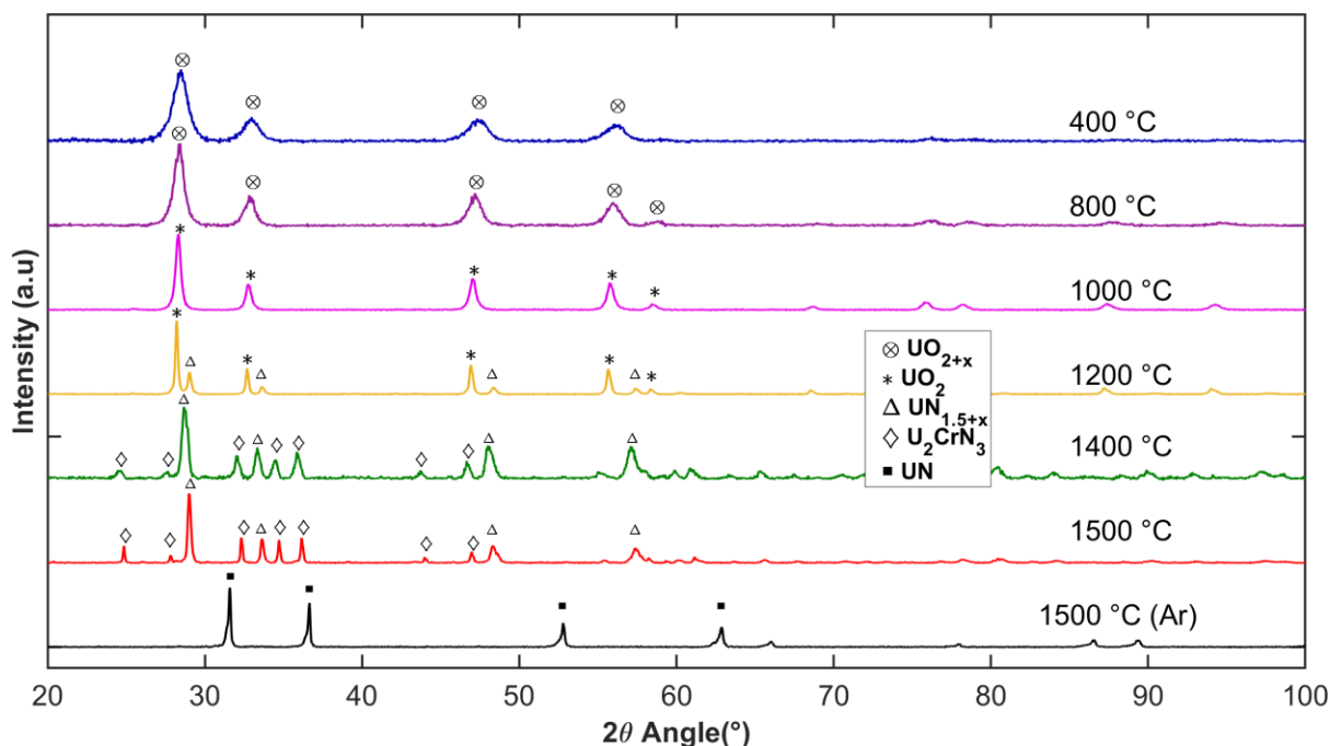
Figure 6.16. XRD patterns measured for the materials heated to different temperatures and cooled in the synthesis gas (H 2 /N 2 ). Phases present were: UO 2+x (⊗), UO 2 (*), UN 1.5+x (Δ), U 2 CrN 3 (◇), UN (■).
