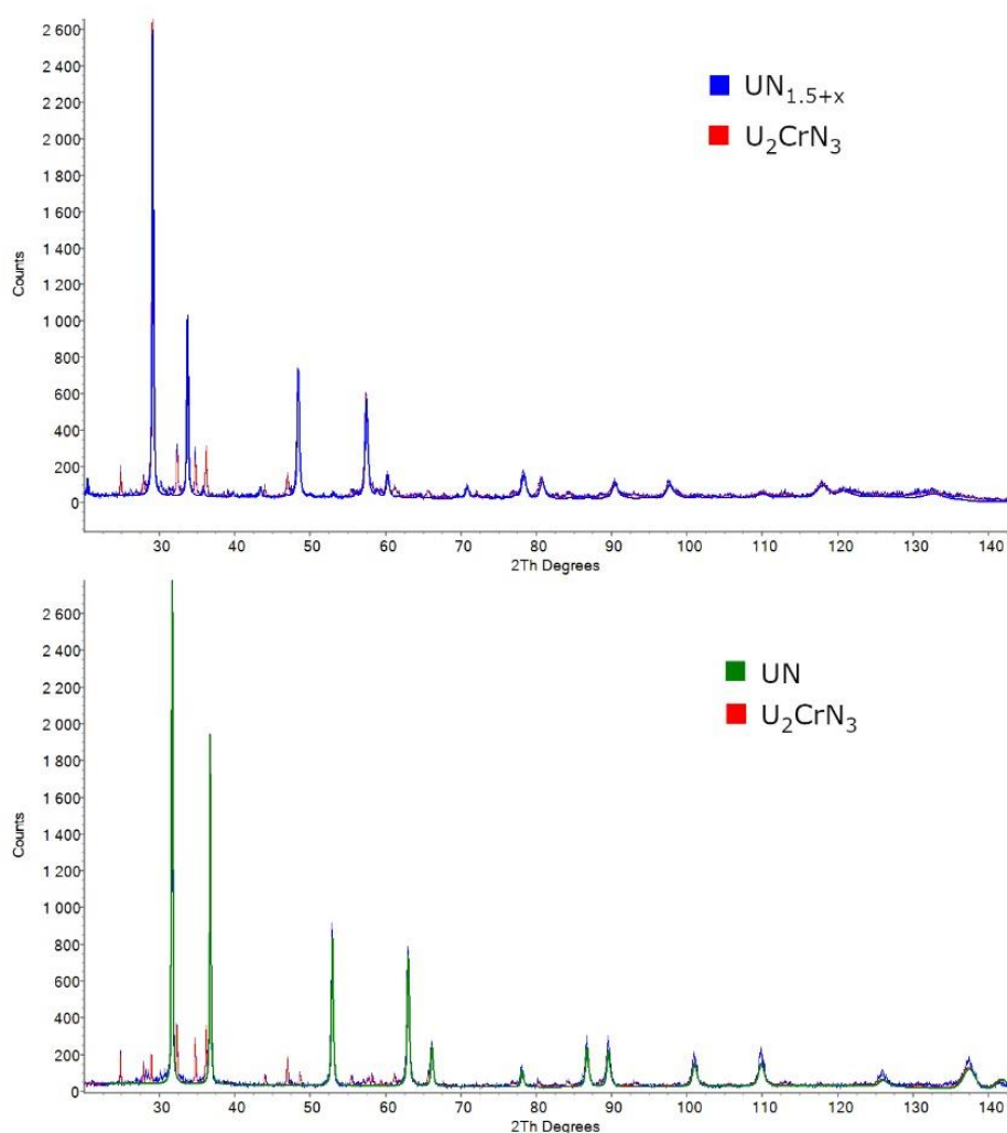
Figure 6.20. Diffraction patterns of sample U80CR20N-23 before (upper) and after (lower) denitridation at 1200 °C showing the transformation of the \text{UN}_{1.5+x} into UN while the ternary phase remained intact.
