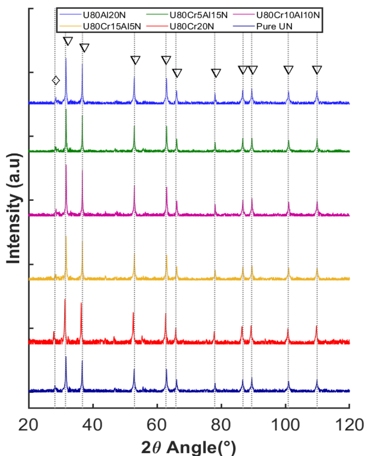
Figure 6.32. X-ray Diffractograms of UN doped with different ratios of chromium and aluminum. Phases observed were UN (∇) and UO 2 (◇).
