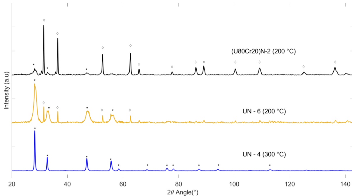
Figure 6.29. X-Ray diffractograms for powders collected after pellet disintegration in the corrosion testing of Cr-doped UN pellets, where UN(◇) and UO 2 (*) signals were identified.
