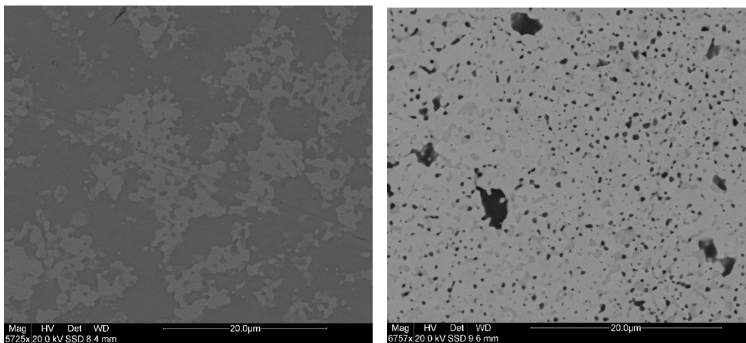
Figure 6.22. SEM of the surface of the U80Cr20N-23 pellet (left) made from spheres containing the ternary phase and the U80Cr20N-13 pellet (right) made from spheres that did not contain the ternary
