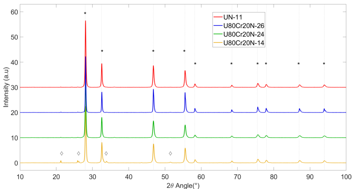
Figure 6.27. X-Ray diffractograms for powders collected after pellet disintegration in the steam interaction experiments, where \text{UO}_2 (*) and \text{U}_3\text{O}_8 (◇) signals were identified.
