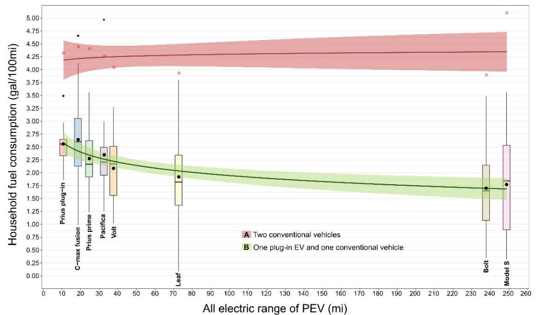
Figure 3. Household fuel consumption vs. range of PEV in two-car households.
