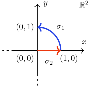
Figure 1.5: The submanifold K used in Example 3. It consists of a quarter circle of radius 1 starting in (1,0) and a line segment from the origin to (1,0) . As the submanifold consists of two distinct parts, we will need two 1-cells to integrate over it.
