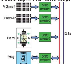
FIGURE 1. - Conventional Multi-input converter
