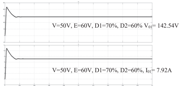
FIGURE 13.- Output voltage and current waveforms of topology (discharging)
