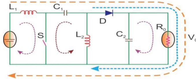
FIGURE 3. - Schematic of SEPIC
