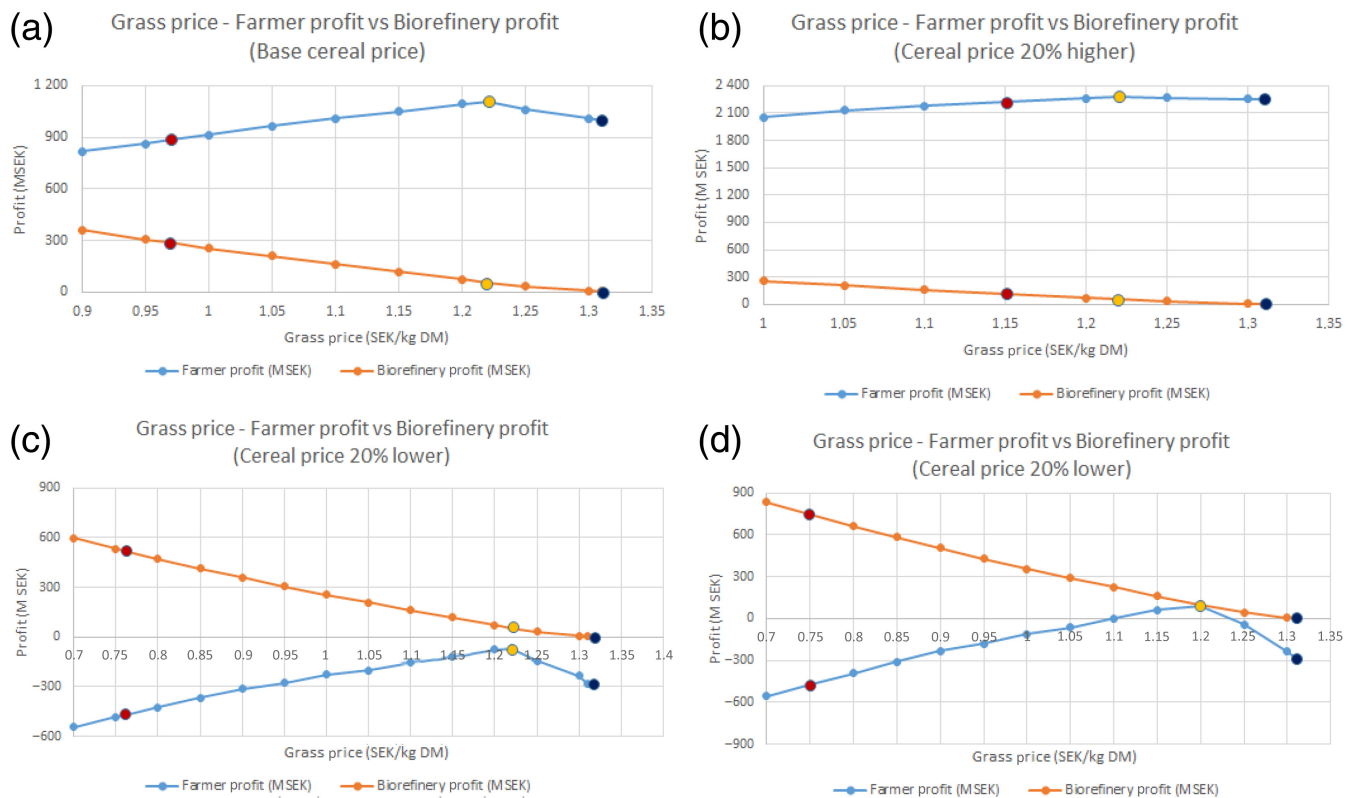
Figure 8. Change in farmer and GB profits with varying biomass prices [the break-even price for the farmer (BEP-F), the price ensuring maximum profit for the farmer (PMP-F) and the break-even price for the GB (BEP-B) are shown with red, yellow and dark-blue dots, respectively].
