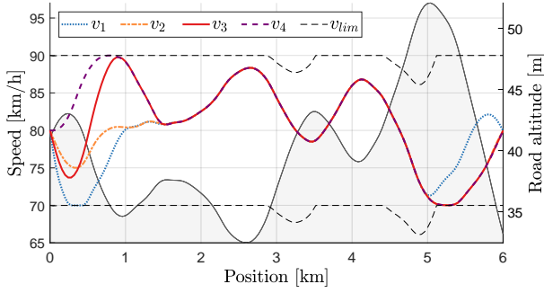
(a) Speed profiles for all trucks.
