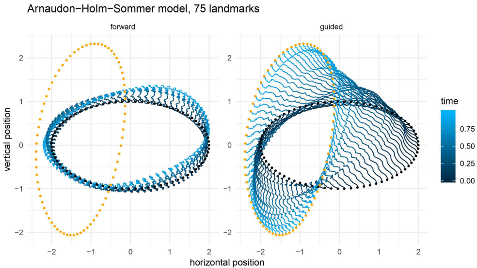
Figure 3. Illustration of the landmarks registration problem. In both figures, the black and orange points are landmarks that represent the shape at time 0 and time 1, respectively. Left: a sample path of the unconditioned process. Right: a sample path of the guided process.
