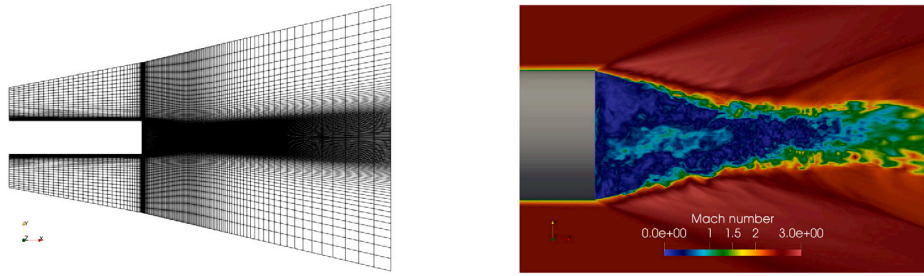
Fig. 7. Supersonic base flow. Illustration of computational domain (left) and visualization of flow field in the near wake of the cylinder (right). Simulation results acquired using LD2C on the finest grid.
