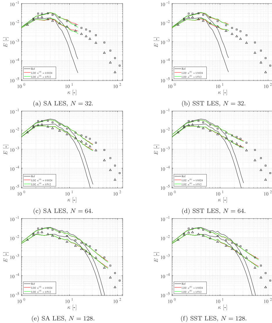
Fig. 3. DIT. Prediction of energy spectra in comparison with experimental data at non-dimensional times \tilde{t} = 0.87 ( \square ) and \tilde{t} = 2.0 ( \Delta ). Effects of numerical scheme. The legend is referred to Table 1.
