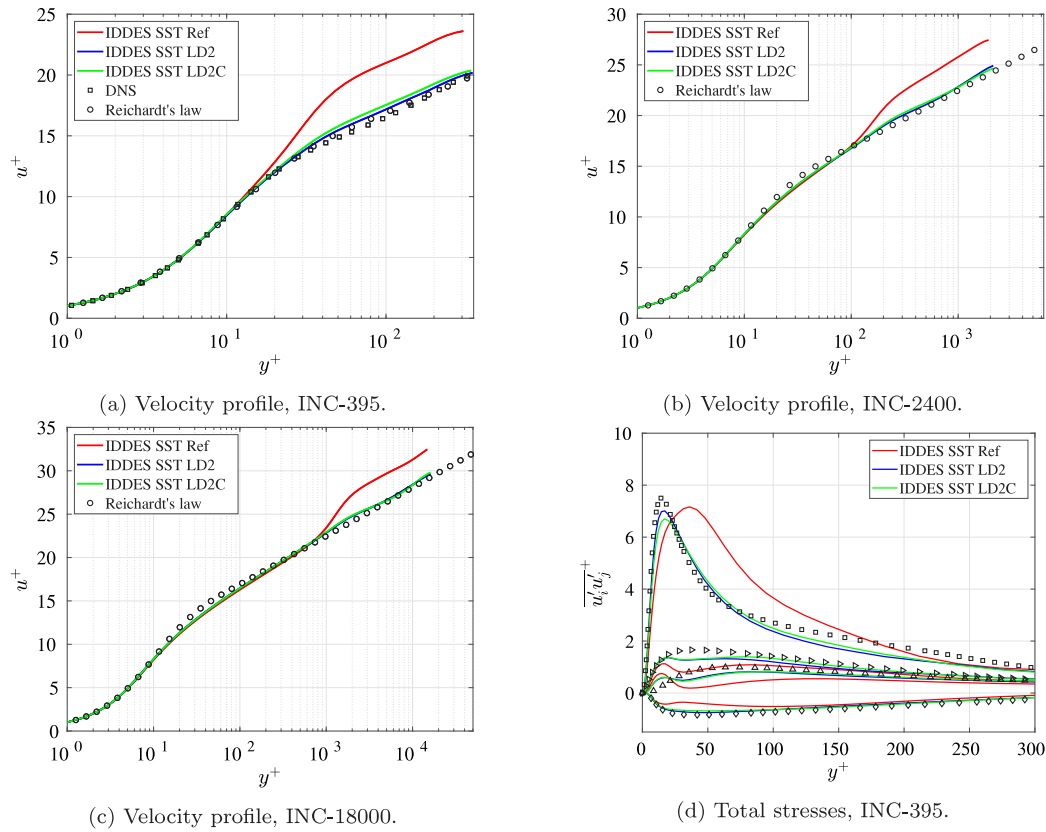
Fig. 4. Fully developed turbulent channel flow with bulk Mach number M_b = 0.15 using SST-IDDES. Effects of numerical scheme. Results compared with Reichardt's law [48] and DNS [44]: \square : \overline{u'u'} , \triangle : \overline{v'v'} , \triangleright : \overline{w'w'} , \diamond : \overline{u'v'} .
