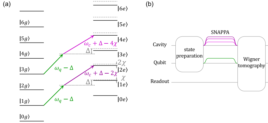
Figure 5.2: (a) Level diagram sketching the SNAPPA gate, here implemented to map the cavity odd parity subspace onto the even-parity subspace, without compromising the even-parity states. The qubit off-resonant drive at frequency f_q - \Delta is common for all the transitions (green arrows). In different shades of magenta arrows, the cavity off-resonant drives at frequencies f_c + \Delta - (n + 1)\chi enable the transition from |n\rangle|g\rangle to e^{i\theta_n}|n + 1\rangle|e\rangle , for each odd n respectively. The phase \theta_n is directly related to the relative phases of the drives. (b) Pulse sequence used to apply the SNAPPA gate. We initialize cavity and qubit to |\Psi\rangle|g\rangle , apply the SNAPPA gate, and perform direct Wigner tomography to measure the state of the cavity.
