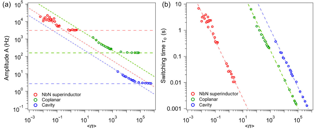
Figure 3.4: Adapted from paper II. Power dependence of the Lorentzian noise (a) amplitude A and (b) switching time \tau_0 for the three different resonators. The horizontal dashed lines in (a) indicate the saturation amplitude A_0 related to minimum FWHM in Fig. 3.3(b). Diagonal lines in (a) indicate 1/\sqrt{n} scaling and not a fit. The dashed lines in (b) are fits of \tau_0 to empirical power law (\langle n \rangle / n_c)^{-\alpha} with \alpha = 1.1 .
