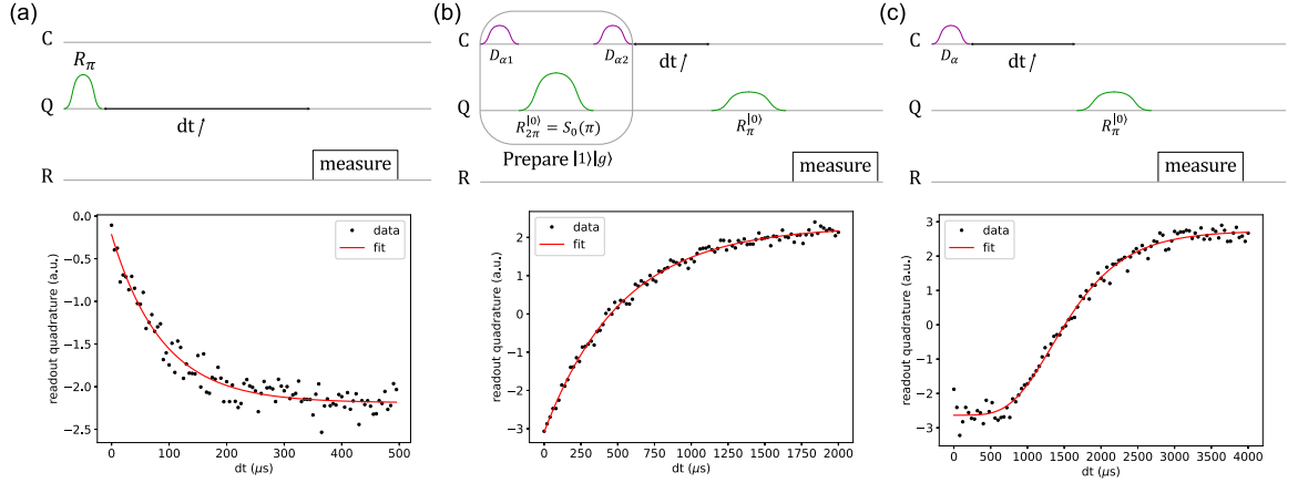
Figure A.2: Calibrating the relaxation time of the qubit (a), and the cavity (b) and (c). The pulse sequence to perform the experiment (top) and an example of the measurement data with the exponentially decaying fit (bottom). One way to prepare Fock state |1\rangle is to apply displacement \alpha_1 = 1.14 , SNAP gate that adds \pi phase to Fock state |0\rangle and another displacement \alpha_2 = -0.58 . \alpha = 3.3 is the displacement amplitude in the example in panel (c).
