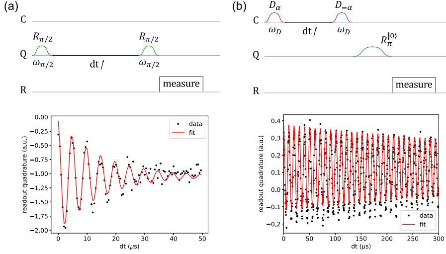
Figure A.1: Calibrating the frequency of the qubit (a) and the cavity (b). We use a Ramsey experiment that we fit to an exponentially decaying oscillation. The pulse sequence to perform the experiment (top) and an example of the measurement data with the fit (bottom).
