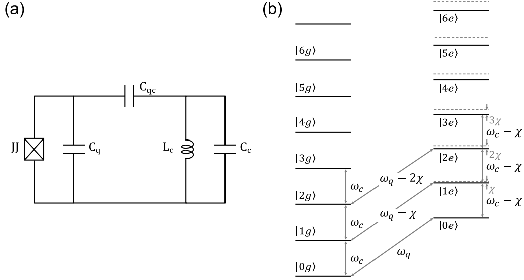
Figure 4.3: (a) Circuit representation and (b) energy spectrum of a resonator dispersively coupled to the two levels of a qubit. The dispersive coupling \chi modifies the frequency of both the resonator and the qubit depending on the state of the other.
