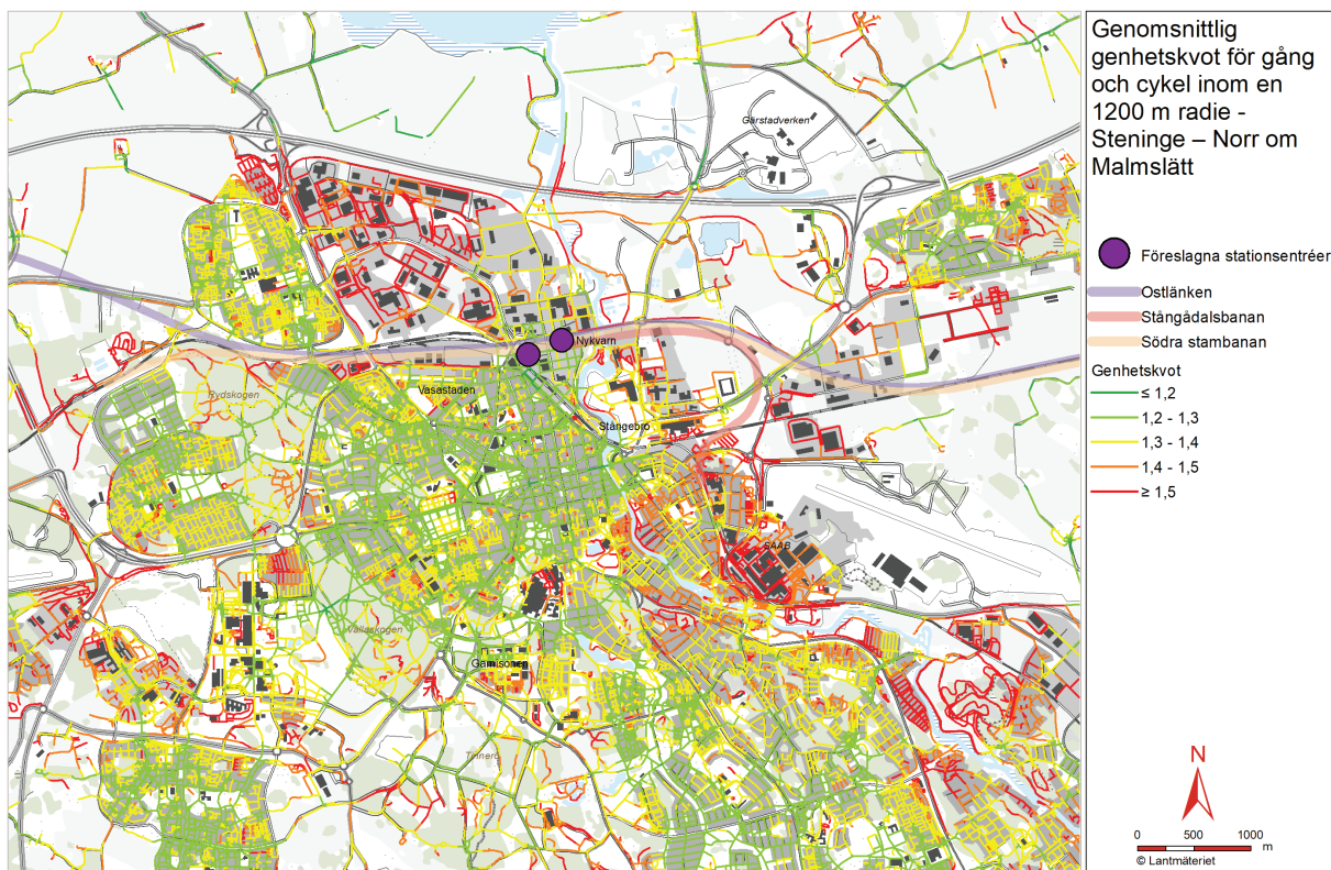
Figure 4 Example of the results of one of the BEA: Analysis for the Steninge corridor of the average detour factor for cycle and pedestrian trips within a radius of 1 200 m from each street segment. Range detour factors between \leq 1,2 and \geq 1,5 .
