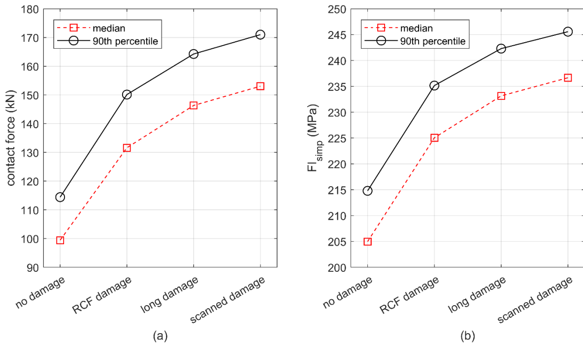
Figure 26: Median (dashed red line) and 90 th percentile (solid black line) of (a) the vertical wheel–rail contact force and (b) the subsurface fatigue index FI_{simp} simulated for a wheel without damage and for the three types of damage studied in Figure 19.
