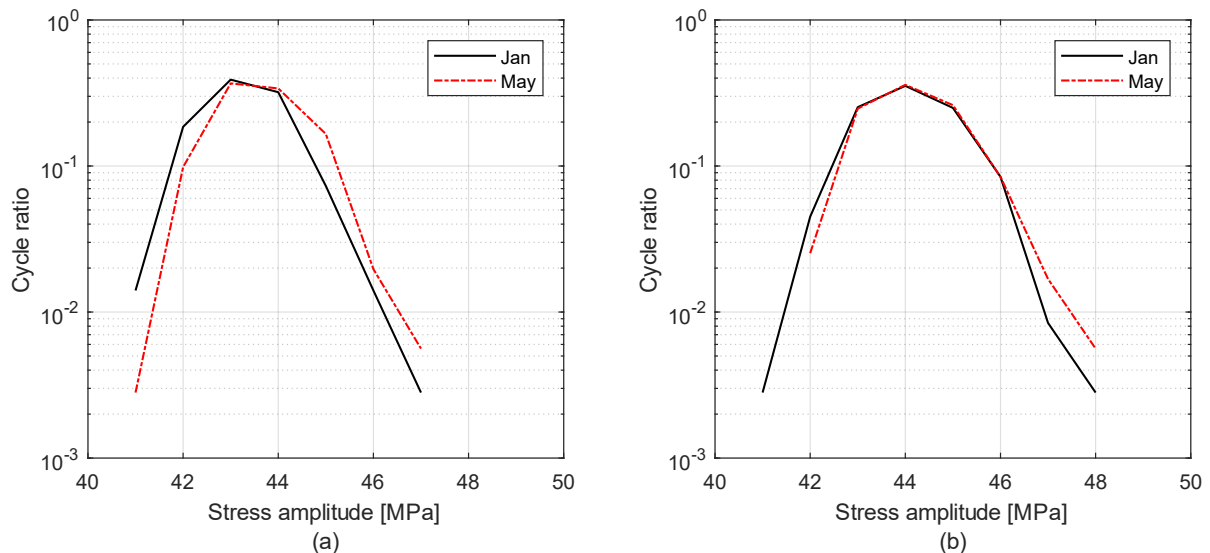
Figure 22: Simulated ratio between number of cycles at different stress amplitudes versus total number of cycles for OOR measured in January 2019 and May 2019 (a) 'Tangent track' and (b) 'Curved track' ( R=500 m). Rail roughness based on ISO 3095 spectrum.
