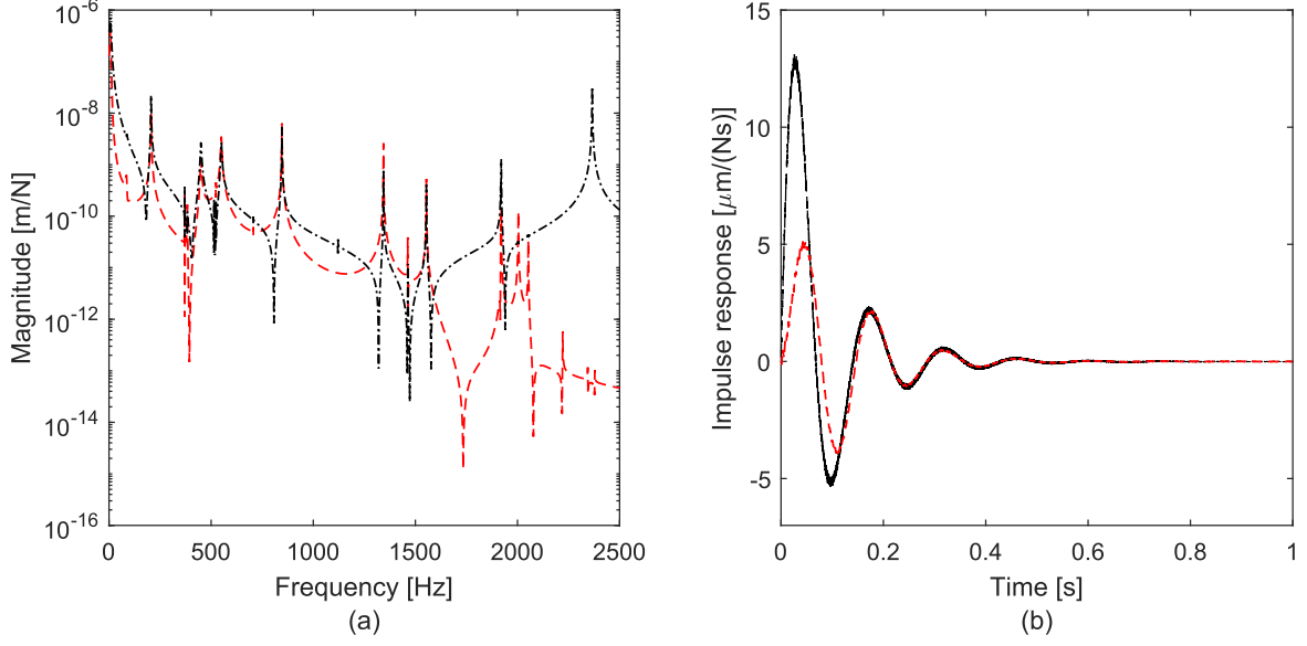
Figure 14: (a) Frequency response functions and (b) corresponding Green's functions for the wheelset model in Paper A and Paper B . The direct receptance and its Green's function obtained for the wheel on the opposite side of the gearbox (named Wheel 1 in the papers) are plotted in black. The cross receptance in the contact point of the opposite wheel and its Green's function are plotted using a red dashed line
