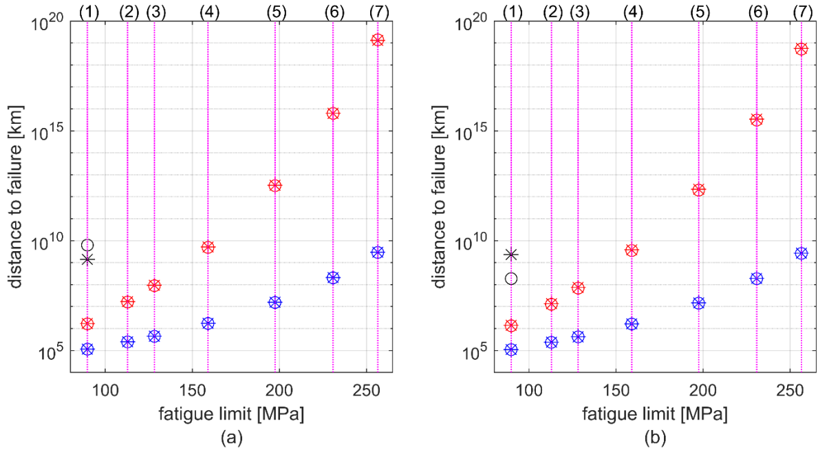
Figure 27: Estimated distance to failure for the instrumented axle for the stretches (a) Hallsberg–Örebro and (b) Örebro–Västerås. Fatigue lives marked with asterisks correspond to statistical models of stress spectra, while those marked with circles are obtained directly from field test spectra. Black markers indicate expected distances to failure if stress amplitudes below the fatigue limit are assumed not to cause any damage. Red and blue markers correspond to assumptions that there is no fatigue limit and the Wöhler curve continues after 10^7 cycles with one third of the original slope or with unchanged slope, respectively. Fatigue limits correspond to different axle surface conditions: (1) corroded in salt water, (2) as forged, (3) corroded in tap water, (4) hot-rolled, (5) machined, (6) fine-ground, (7) mirror polished. A similar figure was produced in Paper C for the stretches Gothenburg–Skövde and Skövde–Hallsberg
