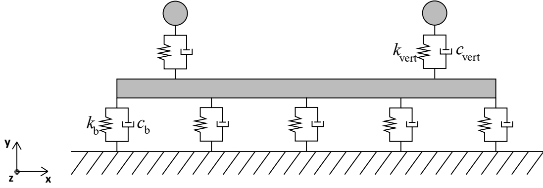
Figure 15: Cross-section of track model used in Paper A , Paper B and Paper E . The view features one sleeper (the horizontal rectangle) and two rails (circles). The sleeper is connected to the ground by non-interacting springs and dampers coupled in parallel. Rail pads are modelled by accounting for both vertical and rotational (with respect to x , not shown in the figure) stiffness and damping
