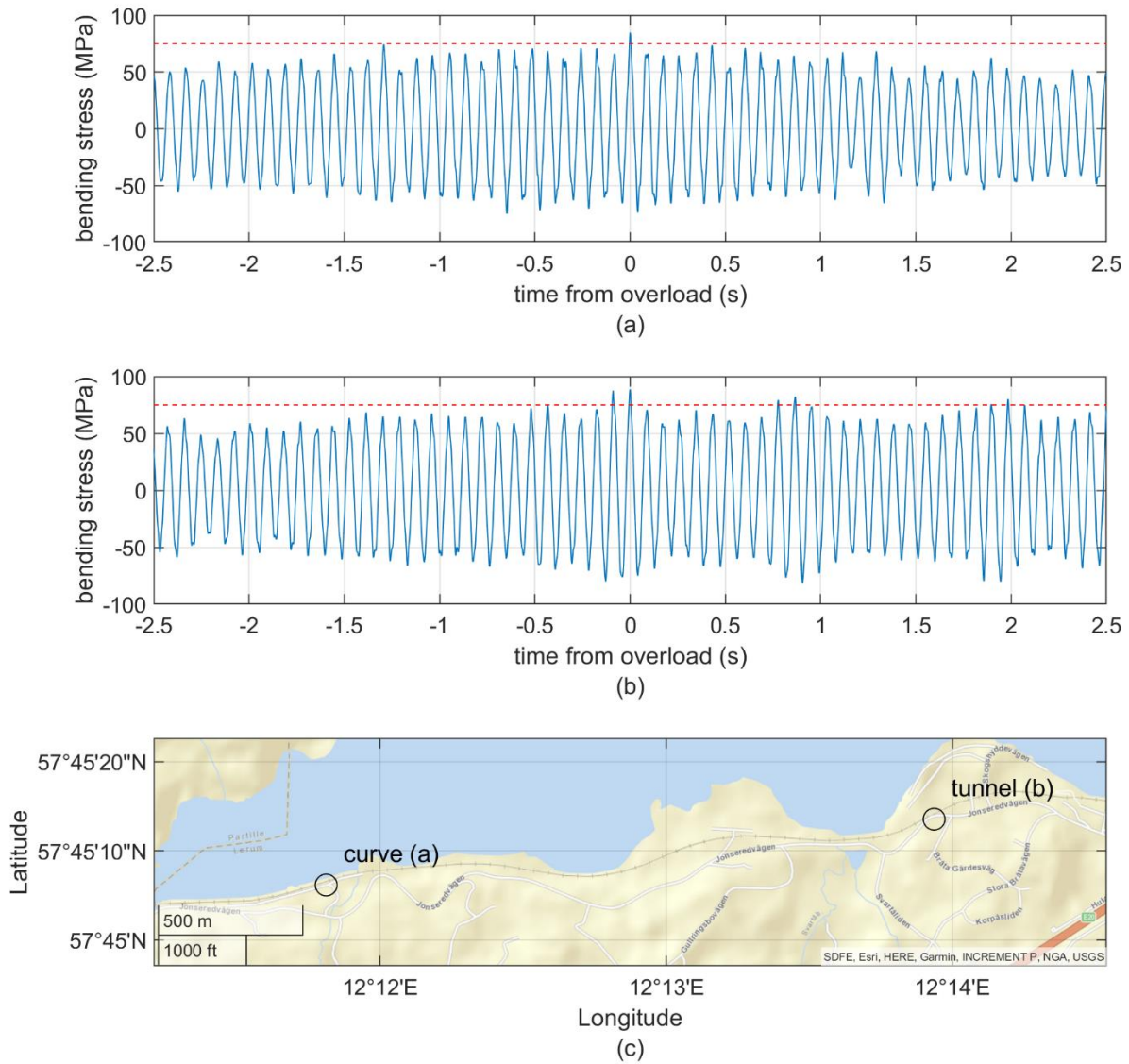
Figure 21: Measured time histories of axle bending stresses for a train ride over (a) a circular curve ( R = 581 m) and (b) a transition curve ( R = 585 m to R=583 m, but with opposite curvatures) in a tunnel. The horizontal red dashed lines indicate the stress threshold used in the study. The locations where peak loads have been registered for the two cases are marked in (c) in the map produced using MATLAB mapping toolbox [77]. Source: Paper D
