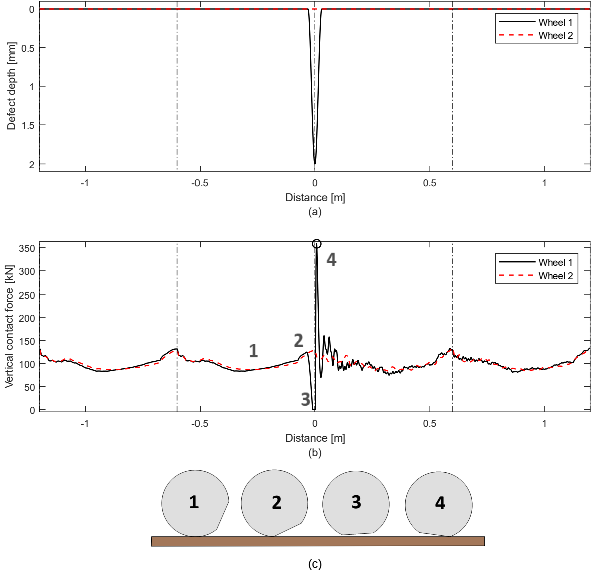
Figure 16: (a) Modelled irregularity at the nominal rolling circle of wheel 1, (b) calculated time history of vertical wheel–rail contact forces for both wheels, and (c) schematic representation of the relative position of the wheel tread defect with respect to the rail. Distance is measured from a point where the circumferential centre of the defect is aligned with a position on the rail directly above a sleeper. Axle load 20 tonnes and train speed 100 km/h. The vertical dashed-dotted lines indicate sleeper positions along the track. Maximum contact force is marked with a circle. Source: Paper A
