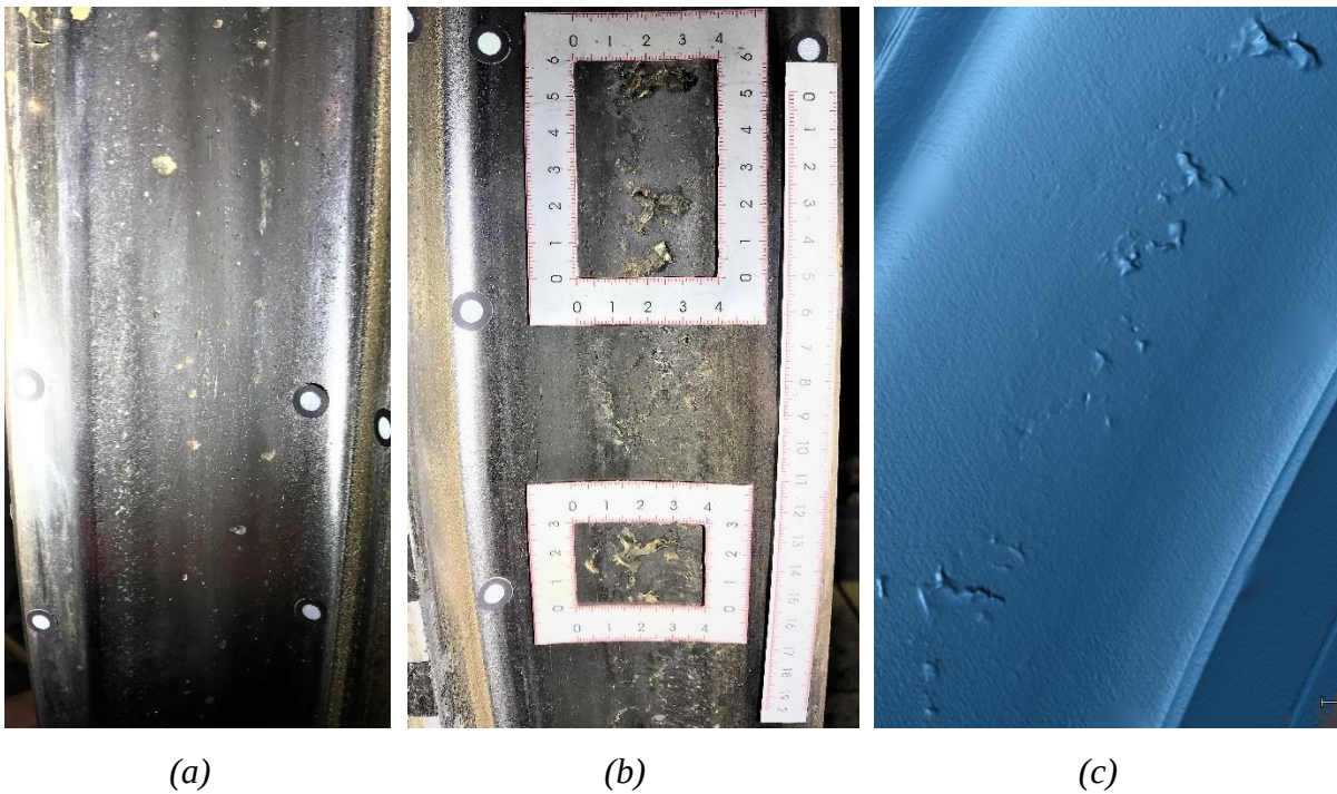
Figure 17: Wheel tread sections of the (a) less damaged wheel and (b) severely damaged wheel used in the field test and (c) surface geometry generated by scanning the severely damaged wheel. Source: Ref. [19] and Paper E
