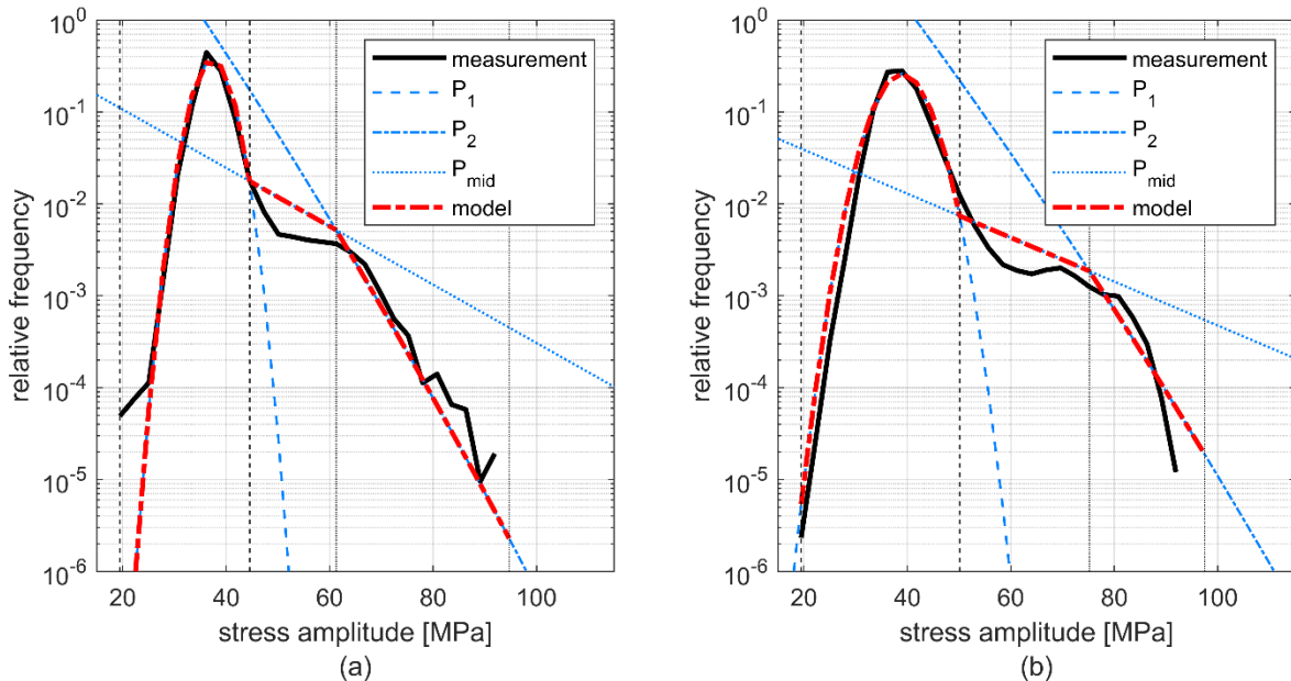
Figure 23: Relative frequency of occurrence of measured stress amplitudes, the probability distributions P_1 , P_2 and P_{mid} and the resulting statistical model of the stress spectrum obtained for the railway lines (a) Hallsberg–Örebro and (b) Örebro–Västerås. A similar figure was produced in Paper C for the lines Gothenburg–Skövde and Skövde–Hallsberg
