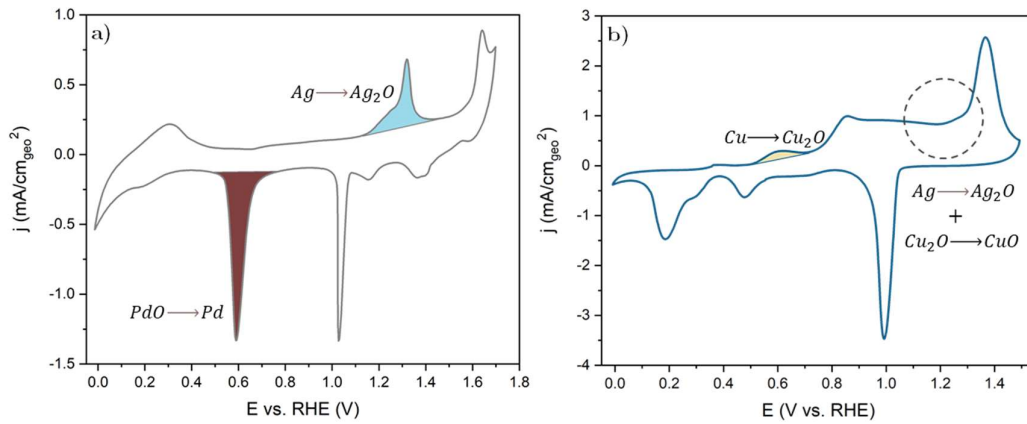
Figure 4.6 Cyclic voltammograms of (a) PdAg and (b) CuAg thin films at 50 mV/s in 0.1 M KOH with the Ag/Pd/Cu redox peaks used for ECSA determination. Although they have both been fabricated with the same Ag loading, they exhibit different Ag peak intensities due to different amount of surface Ag after potential cycling.
