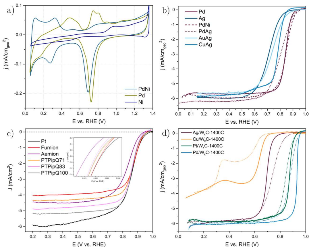
Figure 5.6 Examples of electrochemical screening of electrocatalysts by means of RDE: (a) Cyclic voltammometries of Pd, Ni and PdNi annealed at 500 °C thin films in 0.1 M KOH at 50 mV/s. (b) ORR polarization curves of Pd, Ag and Pd and Ag bimetallic thin films in KOH 0.1 M at 50 mV/s. (c) ORR testing of different alkaline ionomers drop-casted on Pt and their kinetic activities at ~0.9 V. (d) ORR activity of noble metals supported on WxC annealed at 1400 °C in inert atmosphere with the respective pure metals (dashed lines) in 0.1 M KOH.
