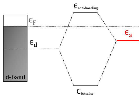
Figure 3.4 Schematic model regarding the whole d-band located at its center and interacting with an adsorbate, together with the resulting bonding and anti-bonding states.
