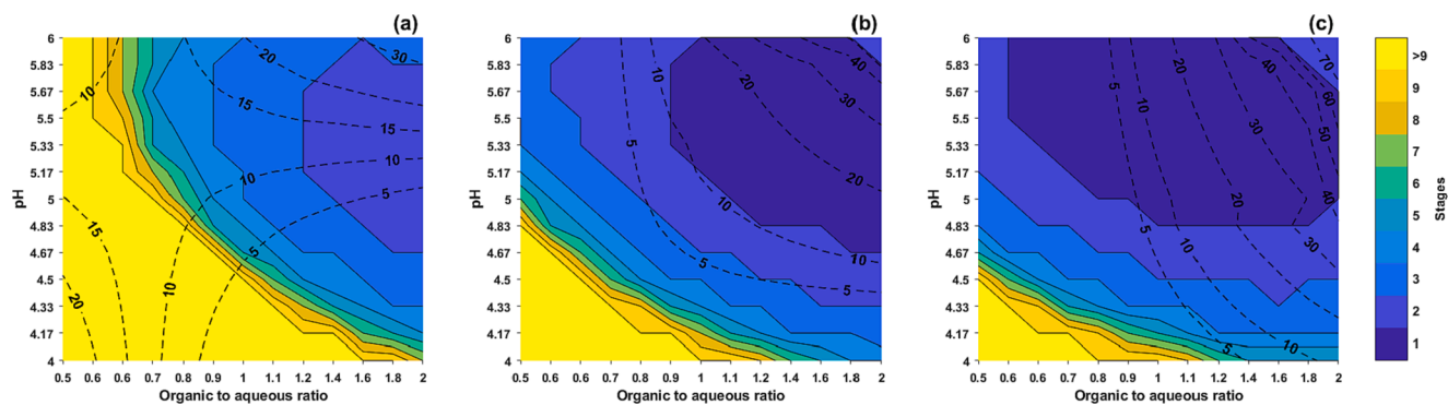
Fig. 8. Response surfaces representing the number of extraction stages estimated to be needed to reach 98% extraction efficiency of Co under different conditions. Dotted response surface representing the co-extraction of Ni. Concentrations of Cyanex 272: (a) 0.4 M, (b) 0.6 M and (c) 0.8 M.
