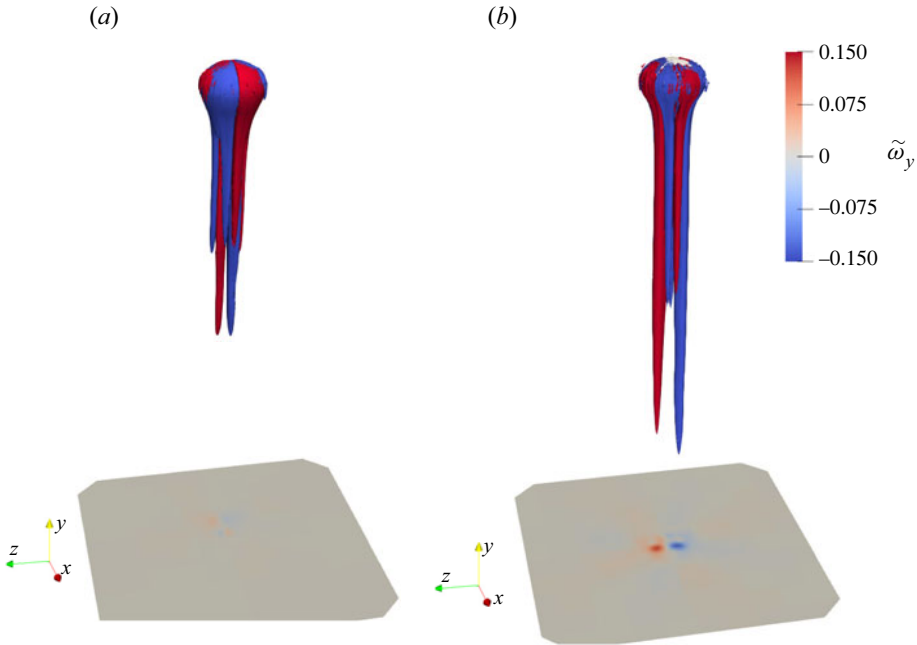
Figure 7. Isosurfaces of the streamwise vorticity \tilde{\omega}_y in the case ( Ga = 240, Eo = 0.1, Sr = 0.05 ) dominated by the L-mechanism. The blue surface indicates the value -0.05 , and the red is 0.05 . (a) The bubble is moving freely in all directions. (b) The bubble is kept fixed in the x - and z -directions using a body force on the bubble but is free to move in the y -direction. The plane below the bubble illustrates the downstream cross-section A_{wake} at which the integration of D_{x,\omega_y} is performed in (5.12). The bubble in (a) moves in the positive x -direction, and the relative transverse velocity generates a secondary \tilde{\omega}_y field at the bubble surface (also illustrated in figure 8) with the opposite sign as the dominant trailing vortices, generated by the L-mechanism, in the wake. The streamwise vorticity is cancelled by cross-diffusion in the wake, and the force D_{x,\omega_y} predicted by (5.12) goes to values much smaller than the lift force at a steady state. This does not happen in (b), where the lift force induced by the trailing vortices is instead balanced by an artificial body force keeping the bubble fixed in the x -direction. (a) Freely moving and (b) fixed in the x - and z -directions.
