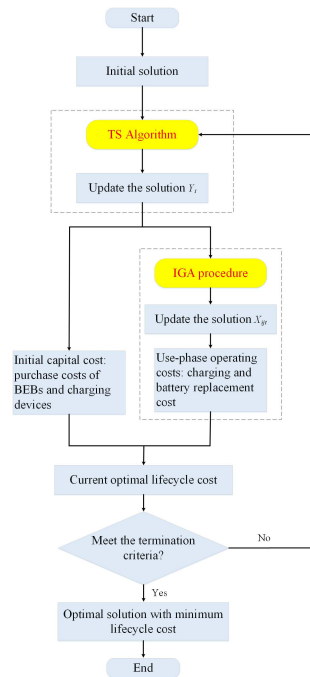
Fig. 2. Flowchart of the hybrid TS-IGA solution method.
