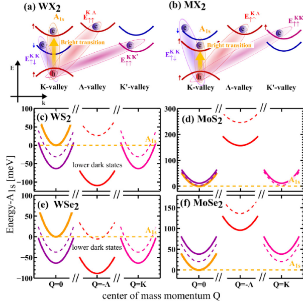
Figure 2.1: Excitonic Landscape for a hole in the K valley. Schematic representation of electronic dispersions around the K and valley for (a) tungsten-based TMDs (WS 2 and WSe 2 ) and (b) molybdenum-based TMDs (MoS 2 and MoSe 2 ). Exciton dispersion in (c) WS 2 , (d) MoS 2 , (e) WSe 2 , and (f) MoSe 2 in SiO 2 substrate calculated by solving the Wannier equation. The figure is taken from [40].
