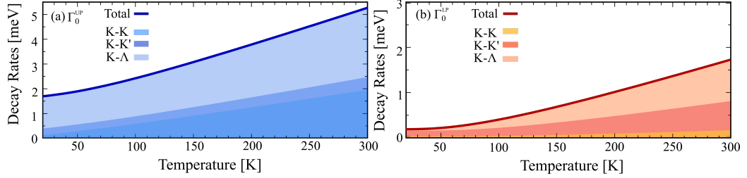
Figure 3.5: Temperature study for WSe 2 . Polariton-phonon scattering rate \Gamma_{\mathbf{k}}^n for the (a) upper (UP) and (b) lower polariton branch (LP) at k=0 as a function of temperature (for Q_f \approx 160 ). We identify the contributions of the intravalley ( KK ) as well as intervalley ( KK' , KA ) scattering channels (shaded areas).
