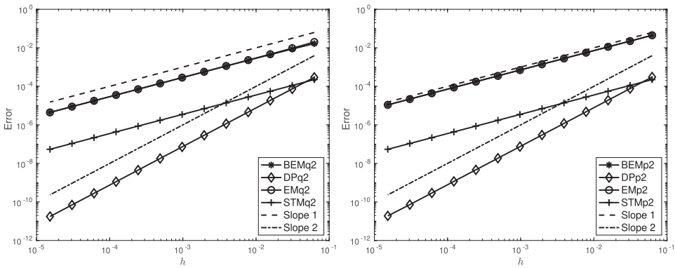
(B) Errors in the second moment of q (left) and p (right).
