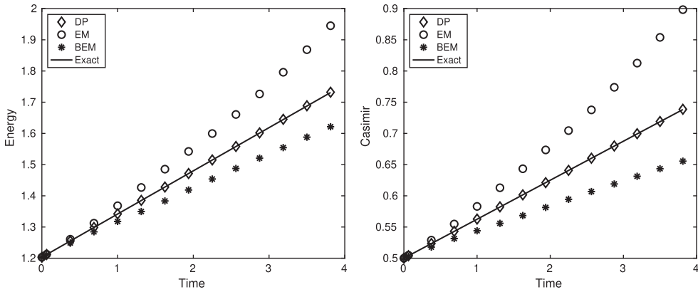
Figure 9. Stochastic rigid body problem with two-dimensional noise: numerical trace formulas for the energy \mathbb{E}[H(X(t))] (left) and for the Casimir \mathbb{E}[C(X(t))] (right) for the drift-preserving scheme (DP), the Euler–Maruyama scheme (EM), the backward Euler–Maruyama scheme (BEM), and the exact solution.
