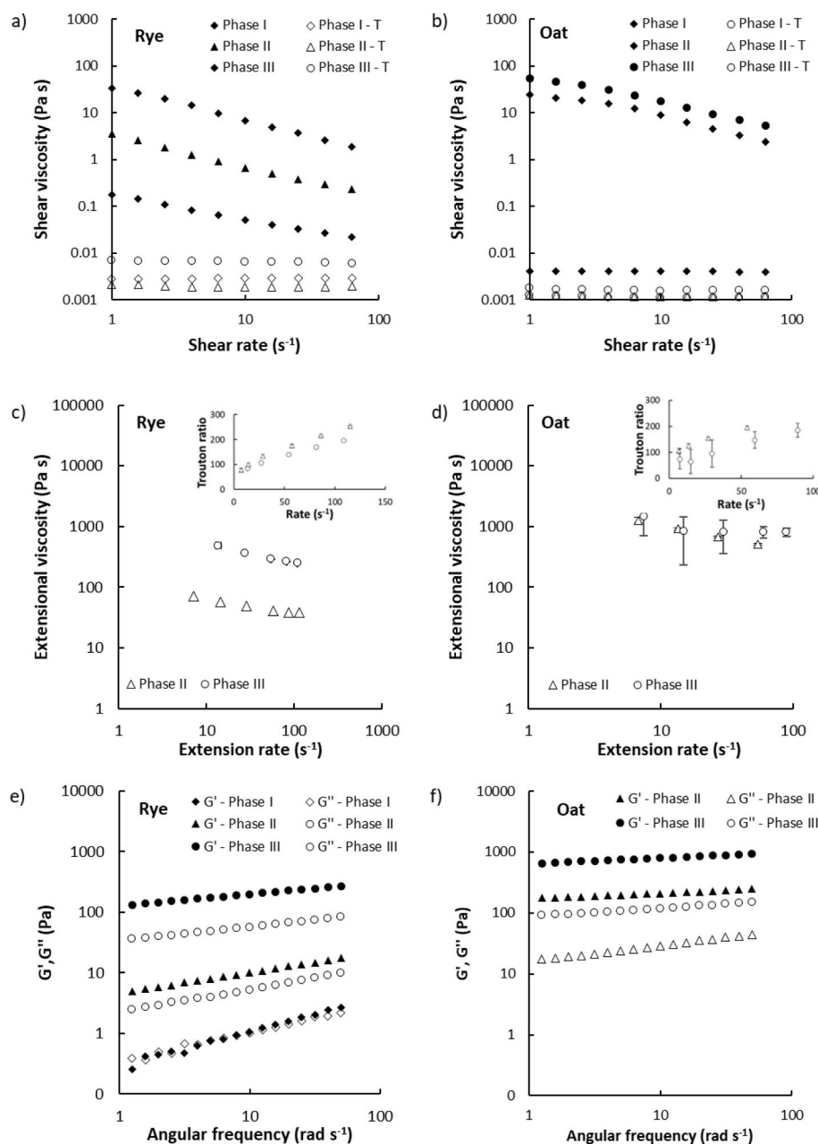
Fig. 4. Representative shear viscosity as a function of the shear rate of phases before and after treatment to hydrolyse starch and remove proteins (T) for (a) rye and (b) oat. Extensional viscosity as a function of the extension rate of phases before treatment for (c) rye and (d) oat. No extensional viscosity was detected for the rye Phase I and oat Phase I. Due to their Newtonian behaviour it was not possible to measure the extensional viscosity of the phases after treatment. The insert represents the Trouton ratio of the oat suspensions. The error bars indicate the standard deviation of three measurements. Representative elastic modulus G' and viscous modulus G'' as a function of the angular frequency of (e) rye and (f) oat suspensions and their related phases before treatment. Due to their Newtonian behaviour, the viscoelastic properties were not measured after treatment.
