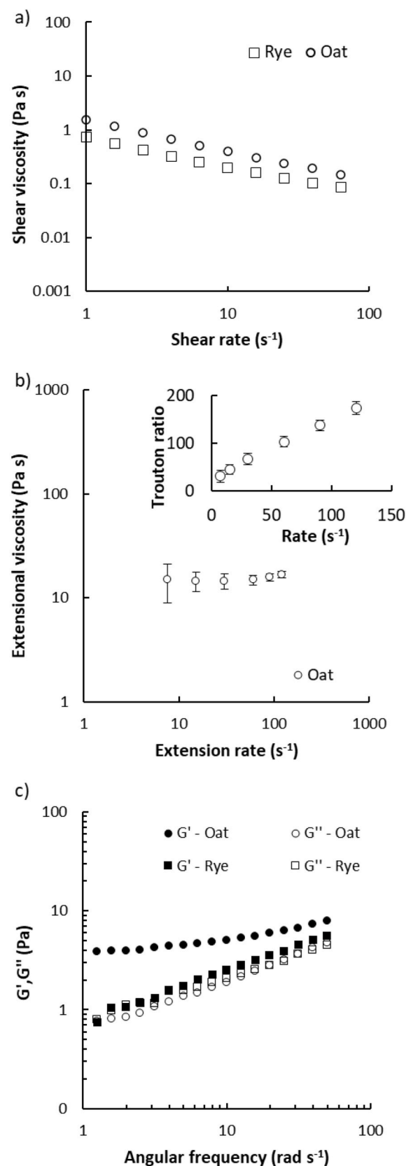
Fig. 3. Rheological properties of rye and oat suspensions (3.5 wt%): (a) shear viscosity as a function of the shear rate; (b) Extensional viscosity as a function of the extension rate. Rye suspensions did not show any extensional behavior. The insert represents the Trouton ratio of the oat suspensions. The error bars indicate the standard deviation of three measurements. (c) Elastic modulus G' and viscous modulus G'' as a function of the angular frequency.
