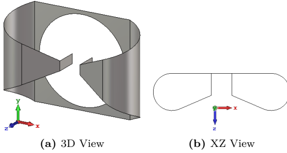
Figure 2: Self-grounded bow-tie antenna optimized for the 250 \sim 500 \text{ MHz} band. The antenna's polarization axis u is aligned with the x axis (red), while its main directivity axis w is aligned with the z axis (blue). The center of the antenna's local coordinate system corresponds to the center of its ground plate, which is also the center of the circular feed opening. The overall dimensions are 8.7 \text{ cm} along x , 6.2 \text{ cm} along y , and 2.4 \text{ cm} along z .
