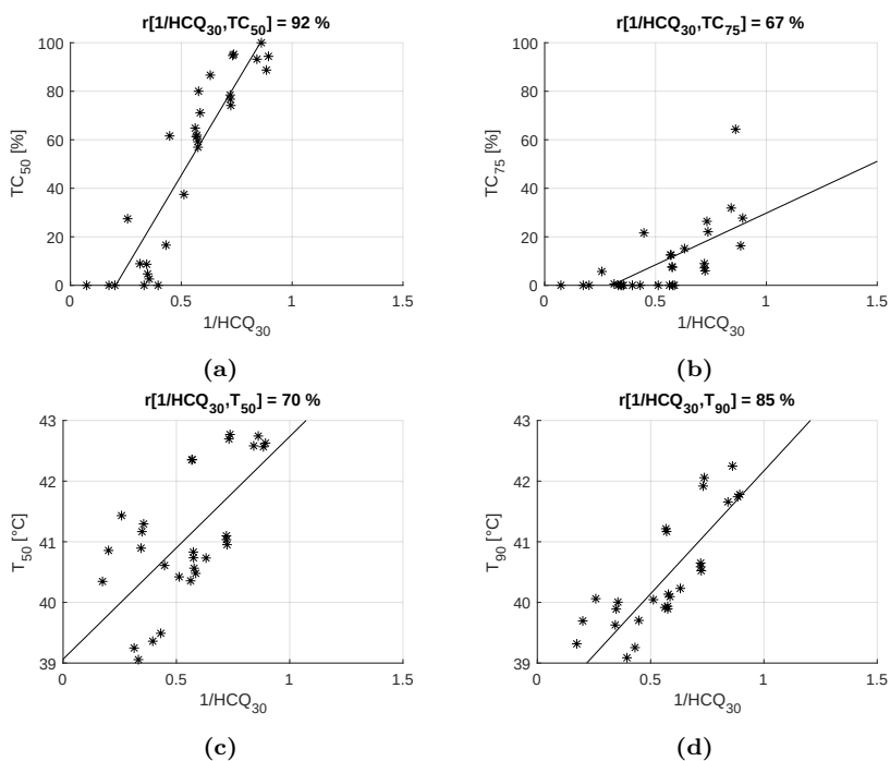
Figure 9: Dispersion plots and linear regression models for the relationship between \text{HCQ}_{30} and the clinical indicators. Model fit on all treatment plan values excluding samples relative to Venus.
