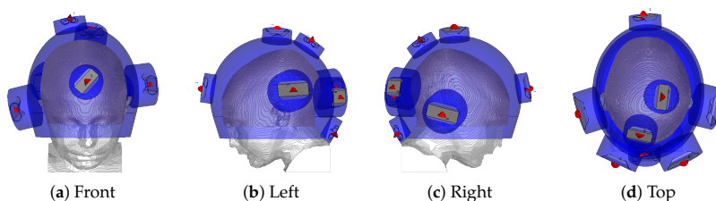
Figure 2. Helmet applicator optimized for the thermal treatment of the tumour considered in this study. The red cones indicate the feed point and polarization direction of each antenna. The blue shade indicates water.
