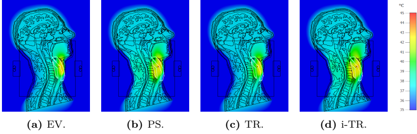
Figure 13: Temperature distributions in the larynx realistic case for all HTP algorithms at 400 + 500 MHz. Maximum temperature in healthy tissues is 43^{\circ}\text{C} in all cases. The target volume is outlined in white. Sagittal section at tumor center.
