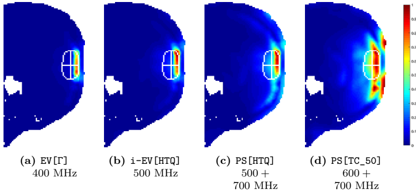
Figure 7: SAR distributions in the meninges case for each optimisation strategy at its optimal frequency or combination of frequencies. Sagittal sections. The target is outlined in white. The sections are taken at the target center, which is indicated by a white cross. The SAR values are normalized to the highest peak inside the patient. The SAR is not calculated for those voxels belonging to background or to the patient's lumina, since they do not represent biological tissue. The sections are rotated by 90^\circ for optimal layout.
