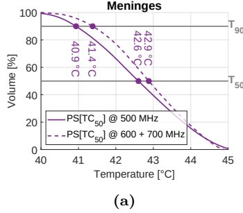
Figure 11: Cumulative histograms of the temperatures reached inside the meningioma target using the TC_{50} -best single-frequency (solid line) and multi-frequency (dashed line) solutions. The gray lines indicate the reference for the 50th and 90th volume percentiles. The dots further report the actual values of T_{50} and T_{90} for these solutions.
