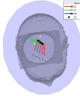
Figure 9: Location sweep for the sensitivity analysis of the field interpolation error. The black circles represent the interpolation grid points. The yellow dots are the grid points selected for interpolation, and are the corners of the triangular patch of largest area. The gray shade is the patient in bird's eye view. The local coordinate systems of each antenna location to be approximated are shown as superimposed triplets.
