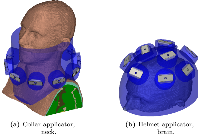
Figure 4: The simulation setups for the collar (a) and the helmet (b) applicators, consisting of patient voxel model, water bolus, and 10 SGBT antennas each.
