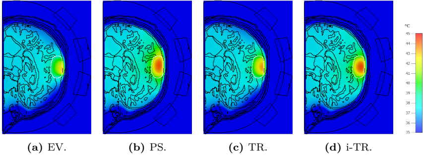
Figure 14: Temperature distributions in the meninges realistic case for all HTP algorithms at 400 + 600 MHz. Maximum temperature in healthy tissues is 43^{\circ}\text{C} in all cases. The target volume is outlined in white. Sagittal section at tumor center.
