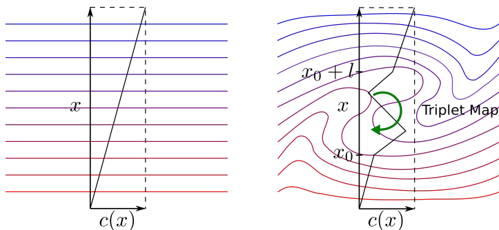
Figure 2.1: Triplet map approximates the stirring effect of a single turnover of an isotropic turbulent eddy; the coloured lines are concentration isopleths for a scalar; the figure on the left represents a scalar gradient where the straight line shows concentration.
