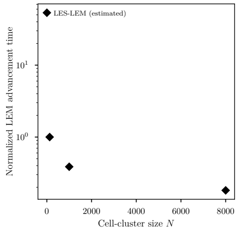
Figure 3.3: Compute times (normalized) for LEM advancement for the test case - data for the three super-grid simulations was recorded from complete runs while the LES-LEM time was estimated from a partial run.
