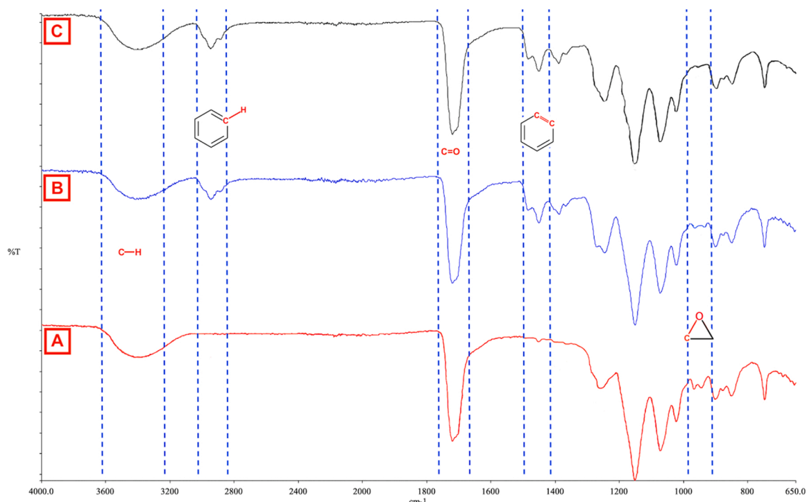
Fig. 2. The FTIR spectra of p(HEMA-co-GMA) (A), and p(HEMA-co-GMA) membranes treated with EGCG at a concentration of 100 (B) and 1000 (C) µg/mL, respectively.
