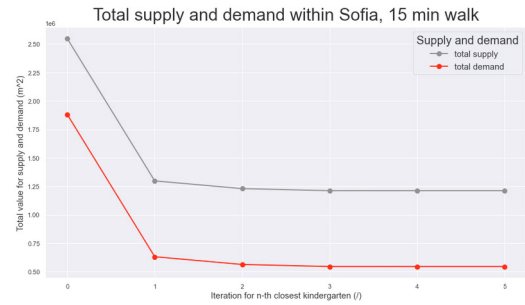
Fig. 4. Convergence curve for 15 minute walking distance
