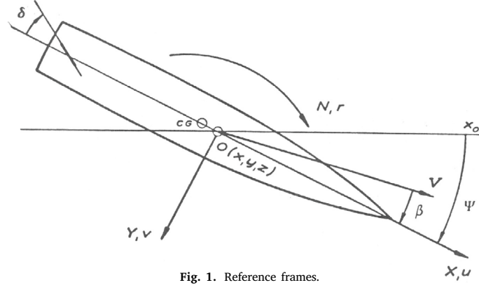
Fig. 1. Reference frames.
