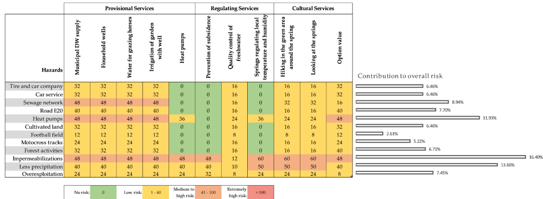
Figure 13. Assessment matrix contrasting hazard sources and their impact on water system services. Numbers from 0 (minimum risk score) to 125 (maximum risk score possible) in the matrix represent the calculated risk score for each hazard-service pair. The bar chart on the right indicates the contribution of each hazard source to the overall risk. (from Gärtner et al., 2022)
