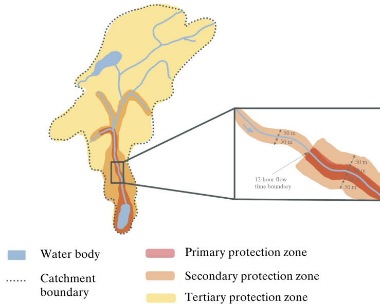
Figure 4. Delineations of surface waters. The illustration on the left illustrates the three protection areas. The illustration on the right shows the two beach zones (modified after SEPA, 2011).
