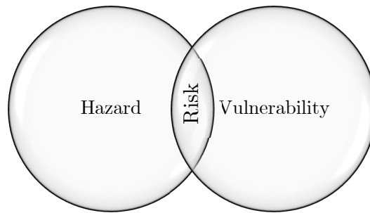
Figure 2. Illustration of the interplay of hazard, vulnerability, and risk towards a drinking water source
