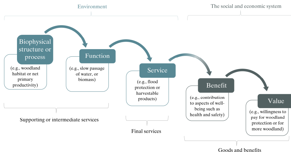
Figure 10. The CICES cascade model modified after (Haines-Young and Potschin, 2018a)
