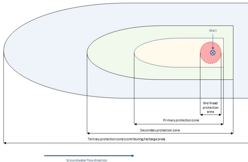
Figure 3. Theoretical wellhead protection zones
