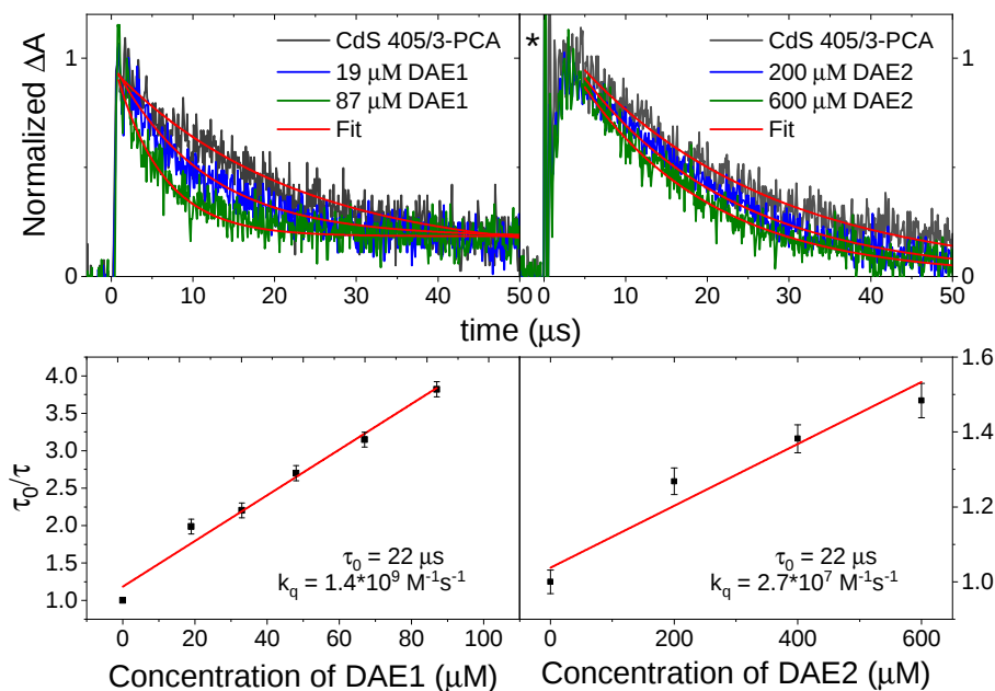
Figure 5.5: DAE quenching of the CdS 405/3-PCA hybrid triplet state. Top figures: Time-resolved transient absorption decays of CdS 405/3-PCA (1.5 \mu\text{M} CdS 405 and 300 \mu\text{M} 3-PCA) in deareated toluene, recorded at 470 nm upon 415 nm pulsed excitation adding DAE1 (left) and recorded at 450 nm upon 410 nm pulsed excitation adding DAE2 (right). *The initial rise in the DAE2 traces is due to laser scattering. Bottom figures: Stern-Volmer plots with linear fits (red lines) for DAE1 (left) and DAE2 (right) quenching of the CdS 405/3-PCA triplet lifetime.
