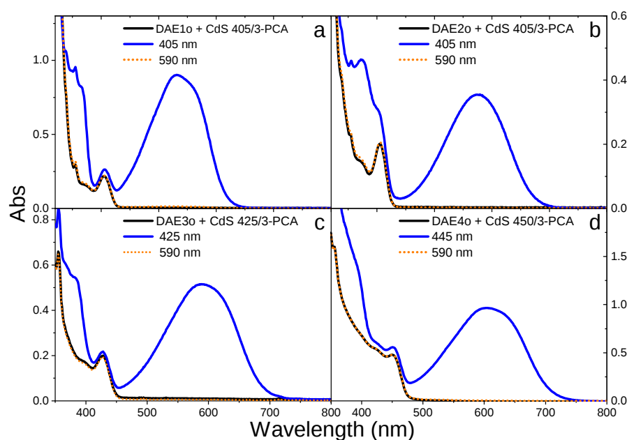
Figure 5.3: Absorption spectra of solutions containing the four DAE derivatives (50 \mu\text{M} of a) DAE1, b) DAE2, c) DAE3, and d) DAE4), CdS NCs (0.5 \mu\text{M} CdS 405 in a and b, 0.3 \mu\text{M} CdS 425 in c, and 0.5 \mu\text{M} CdS 450 in d) and 3-PCA (100 \mu\text{M} ) in deareated toluene. Spectra are recorded for the open isomers before (black lines) and after irradiation of 405 nm, 425 nm, and 445 nm light respectively (120 s, blue lines), and then after 590 nm light irradiation (90 s, orange dotted lines).
