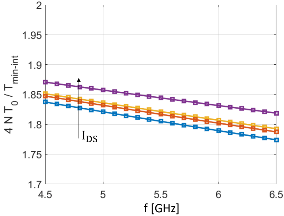
Figure 20: Variation of \frac{4NT_0}{T_{min-int}} with frequency at cryogenic temperatures, at I_{DS}[mA] = 2.5 - 10 , V_{DS} = 5 V – from [A].
