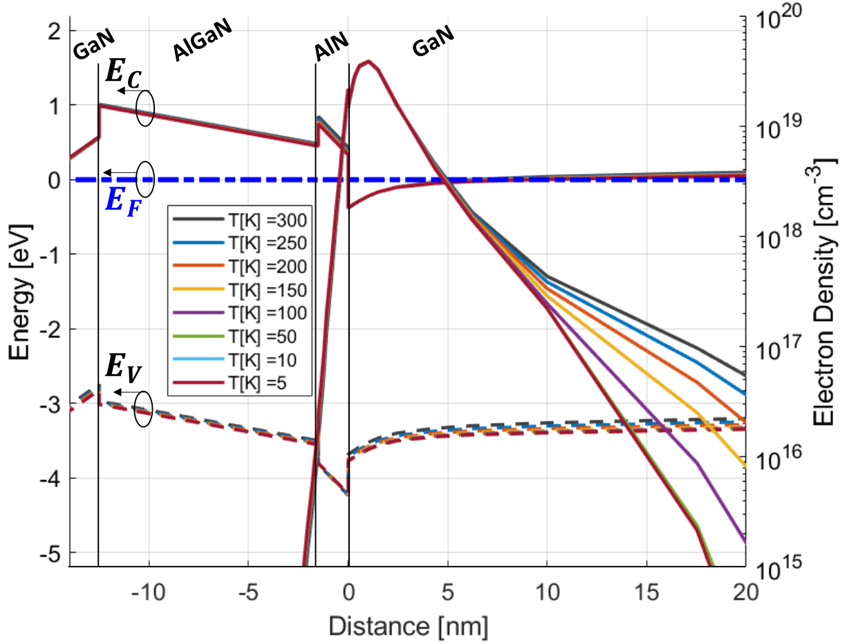
Figure 4: The spatial distribution along a vertical cutline from the cross-sectional view of the device of: the electronic energy bands (left axis); the valence band (dashed lines) and the conduction band (solid lines), E_F indicates the Fermi level (left axis, dot-dashed lines), and the electron density (right axis, solid lines). The results at 8 physical temperatures, T , from 300 down to 5 K are shown.
