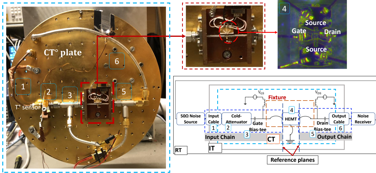
Figure 22: Image of the cryogenic noise measurements setup (left) with the corresponding block schematic (right). The image was mirrored to facilitate the readability of the schematic from left to right. In the top right is shown a microscopic top-view image of the transistor with the interconnecting bond wires, as mounted on fixture for the noise measurements. IT refers to the physical temperature of the cryostat stage interfacing the RT to the CT parts of the system. Reproduced from [A]
