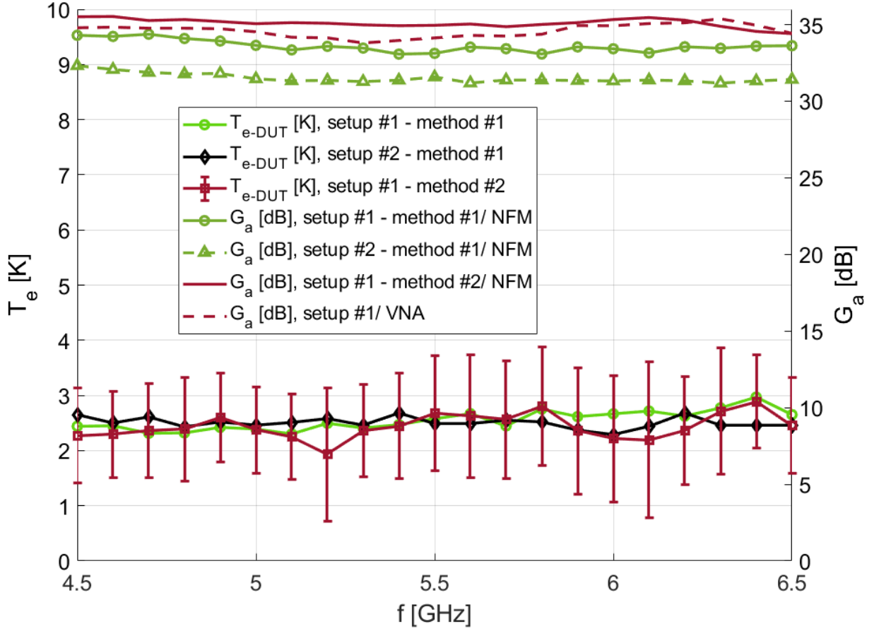
Figure 24: Comparison of the results of the calibrated LNA measured at \sim 10 K. The error bars are providing the RSS uncertainty of the noise temperature measured at each frequency point.
