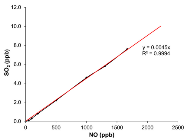
Figure 3. Sensitivity to NO of the Thermo 43i TLE sensor used in this study.
