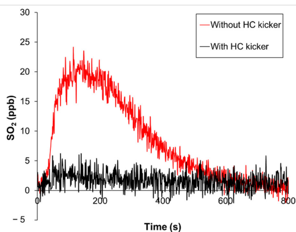
Figure 5. Erroneous SO 2 measured concentration indicates the effect VOCs (using spray paint in a lab environment) have on the SO 2 measurement signal. The red line shows the erroneous indicated SO 2 sensor reading without an HC kicker and the black line shows the erroneous sensor reading when the HC kicker was installed in the airflow before the SO 2 sensor.
