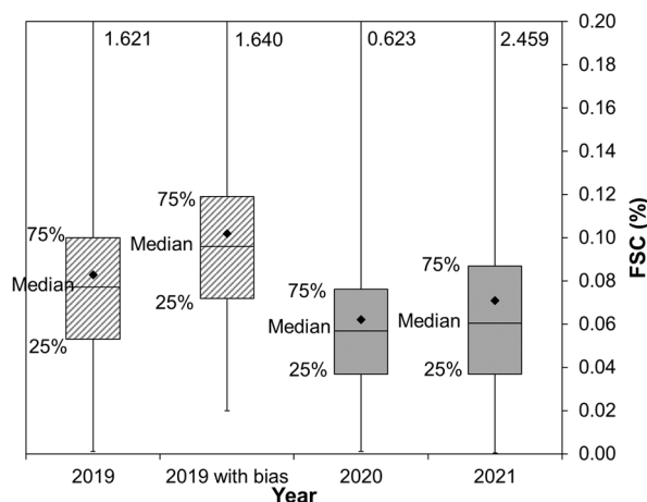
Figure 7. Box plot with 25, 75% percentiles medians and annual average (◆) of the monitored OGVs for the years 2019, 2020 and 2021. The data for 2019 is arched as the measurement for 2019 and were conducted with another measurement methodology with higher uncertainty. Both the uncorrected and corrected data for 2019 are visualized (bias of +0.0189% FSC).
