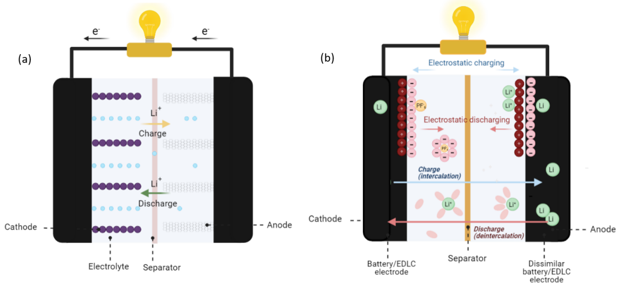
Figure 10. Schematic representation of (a) conventional lithium-ion battery and (b) hybrid configuration of lithium-ion capacitor.
