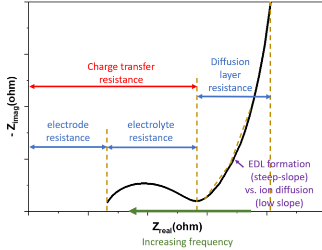
Figure 16. Nyquist plots of the impedance of a Randles circuit with Warburg impedance when the scale is orthonormal, and the low-frequency angle is 45°.
