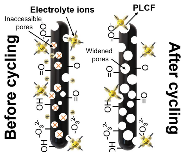
Figure 23. Schematic representation of the accessibility of solvated KOH electrolyte ions to unfit pores (red-crossed) after cycling over a series of continuous insertions and desortions in PLCF electrodes
