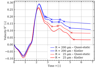
FIG. 11: The normalized velocity using two contact-angle models: the quasi-static model (the dashed lines) and the Kistler dynamic model (the solid lines) for two initial droplet radii R_i . The crosses (x) and circles (o) represent the moments where detachment and re-attachment occur. The normalized velocity plots illustrate how the use of different models affects the upwards velocity of the droplets. The use of the Kistler model results in the lower jumping velocity for both R_i .
