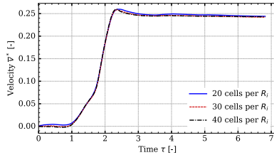
FIG. 3: Grid convergence study of the average upwards velocity in time, normalized by the capillary-inertial scales, for three different grid configurations for R_i = 25 \mu\text{m} . The cases involving 30 and 40 cells per R_i demonstrate convergence of the jumping velocity behavior.
