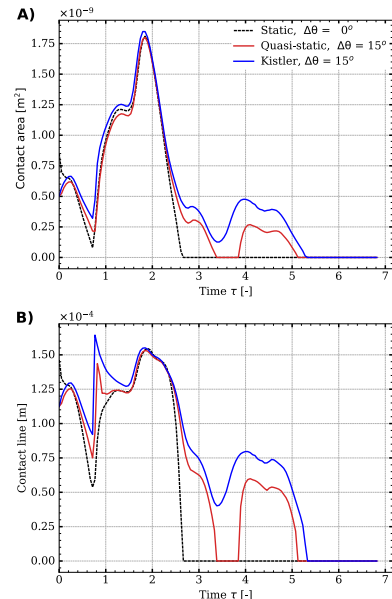
FIG. 14: A) Contact area evolution and B) the contact-line length evolution for the merged droplet on the superhydrophobic solid surface. Three different contact-angle implementations with the same equilibrium angle \theta = 155^\circ and the initial droplet radii R_i = 25 \mu\text{m} . A higher value of the contact area before the late detachment can be observed when stronger hysteresis is imposed. The contact line follows the same trend, despite a "spike" when the liquid bridge hits the surface.
