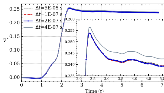
FIGURE 1 Demonstration of time convergence of our simulations. We note that the time convergence is achieved for a time step of \Delta t = 2 \cdot 10^{-7} s or shorter. The initial radius of merging droplets is 100 \mu\text{m} and \text{CFL} < 0.7 for the simulation. CFL, Courant number
