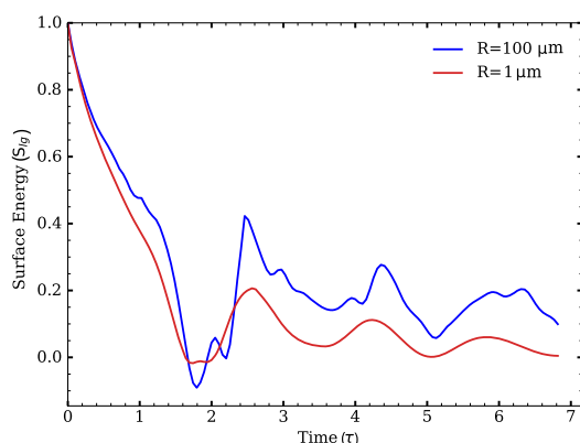
FIGURE 7 Surface energies ( S_{\text{ig}} ) for the R = 100 \mu\text{m} and R = 1 \mu\text{m} cases. The energies are computed from the interface area of the water–air interaction and are normalized by the available released surface energy for each case. A higher percentage of the available energy has been released during the early jumping stage for R = 1 \mu\text{m} droplets.
