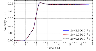
FIG. 2: Time convergence study of the average upwards velocity in time, normalized by the capillary-inertial scales. The radius of the initial droplets is 25 m.
