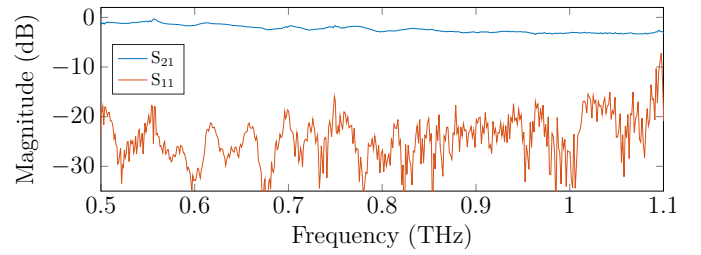
Fig. 8: Measured S-parameters for a 1-mm-long PGL fabricated in the same high-resistivity silicon membrane.
