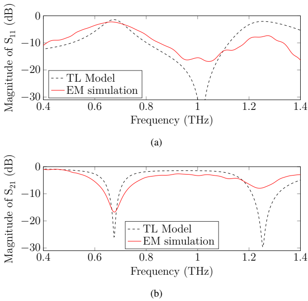
Fig. 4: S-parameter comparison of the transmission-line model and electromagnetic simulations for a single-resonator-pair filter. The model shows to properly reproduce the pass- and stopbands of the filter. (a) |S_{11}| and (b) |S_{21}| .
