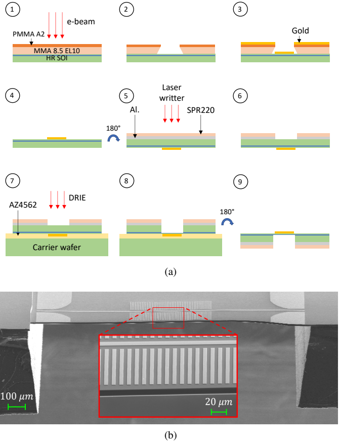
Fig. 6: (a) Sketch of the fabrication steps of the proposed silicon-on-insulator chip (NB! The drawings are not in scale). (b) Scanning-electron-microscope image of the filter fabricated on the high-resistivity silicon membrane. The inset shows detail of the membrane and resonators. Unfortunately, the left side of the membrane broke when cleaving the chip for the picture.
