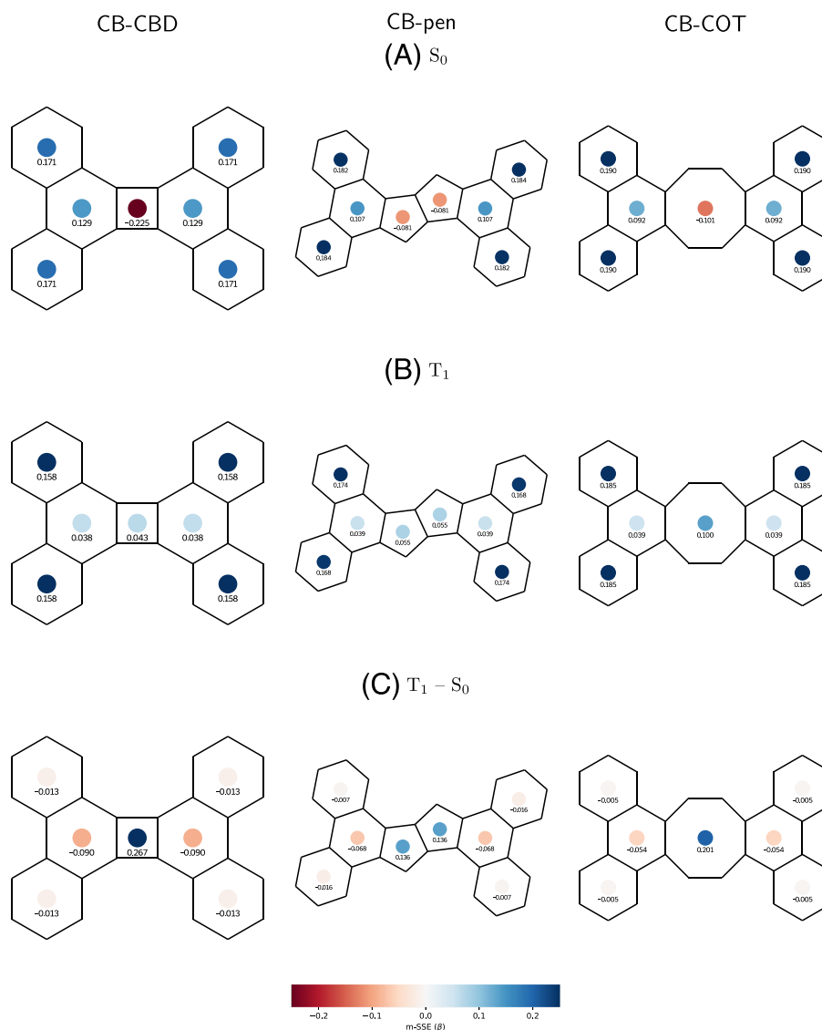
FIGURE 8 m-SSE values for CB-CBD , CB-pen , and CB-COT in (A) S_0 , (B) T_1 , and (C) the difference between T_1 and S_0 . Results with the variable \beta method and GFN2-xTB geometries. Colored blue circles indicate the m-SSE values (darker = higher value)
