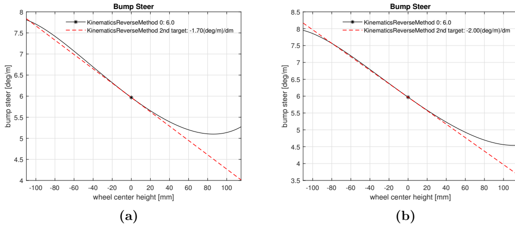
Figure 3.7: Simulation result of bump steer include the effect from toe and camber changes (a), and exclude the effect from toe and camber changes (b).
