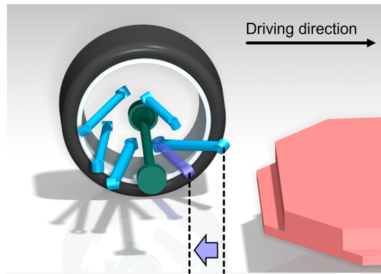
Figure 4.3: Application:Optimized Rear-Axle Concept for Battery Electric Vehicle.
