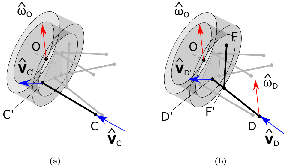
Figure 3.5: Motion ratio calculation.
