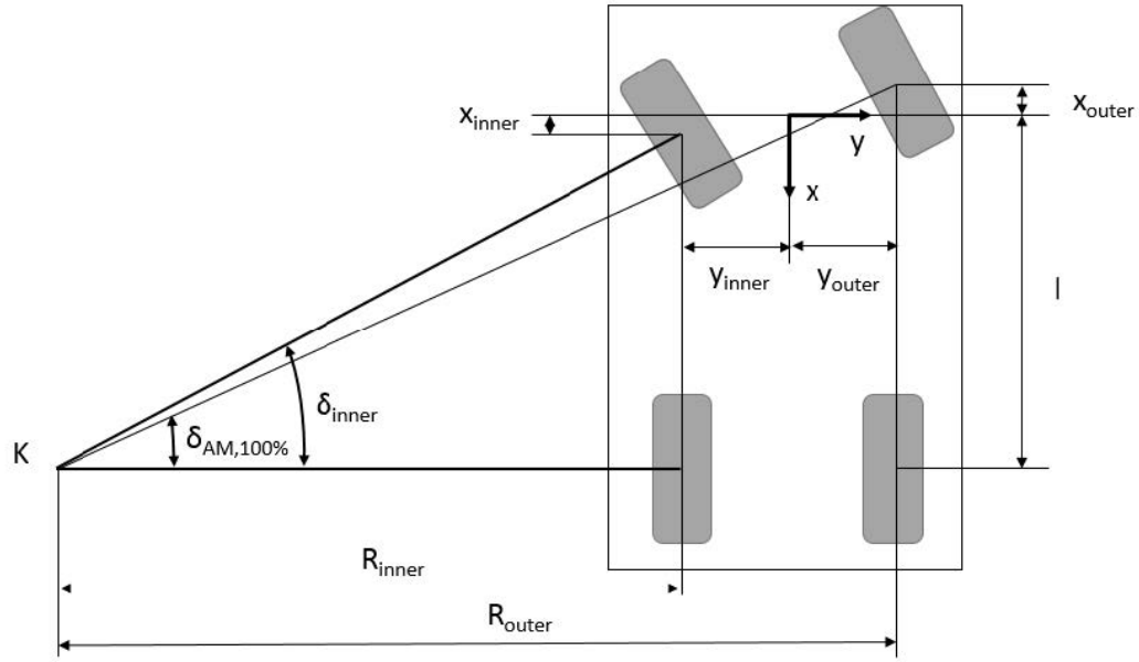
Figure 3.2: Configuration of Ackermann angle.
