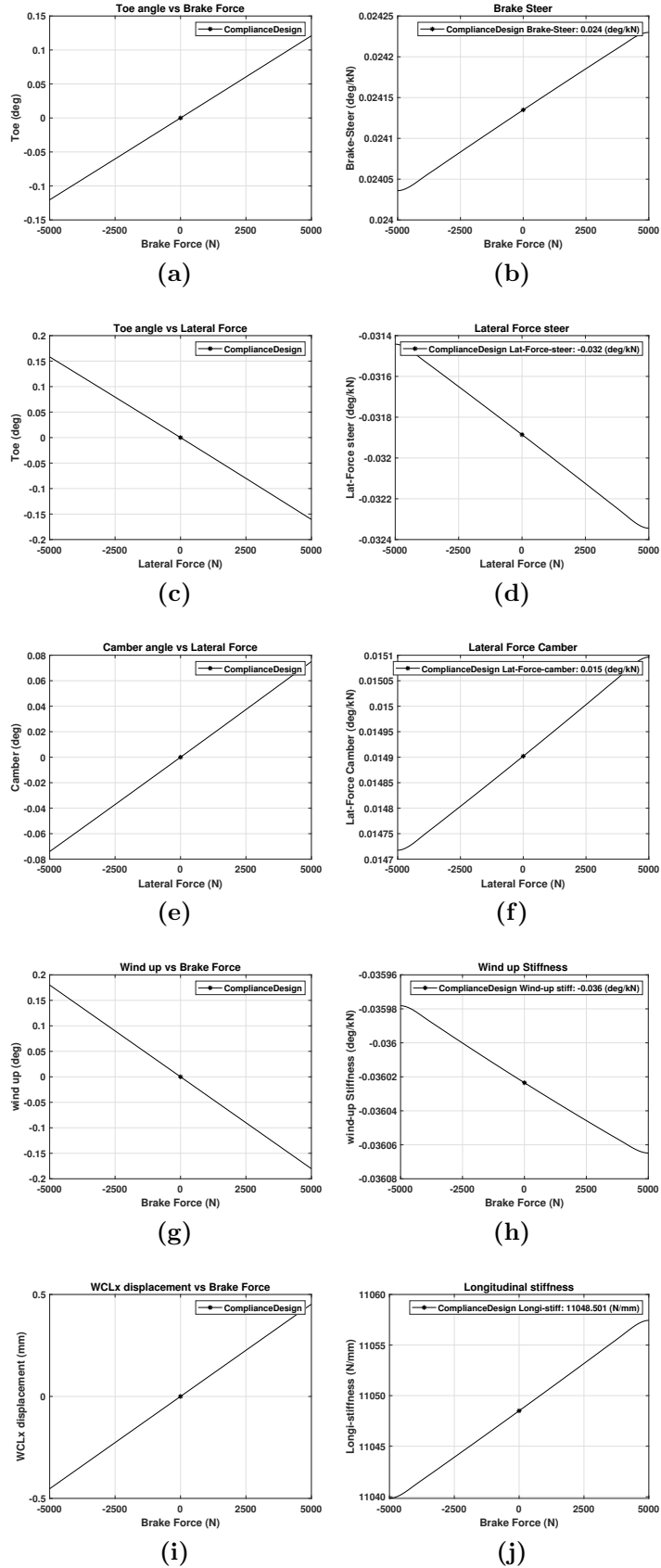
Figure A.2: Result from compliance simulation.
