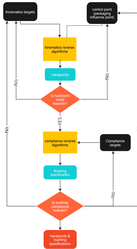
Figure 3.6: Flowchart for concept suspension development.
