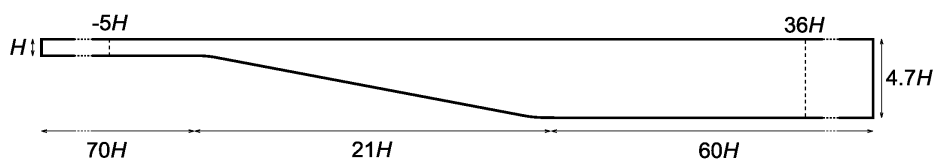
Figure 2. Asymmetric planar diffuser. The vertical dotted lines indicate the region where the fibers are present
