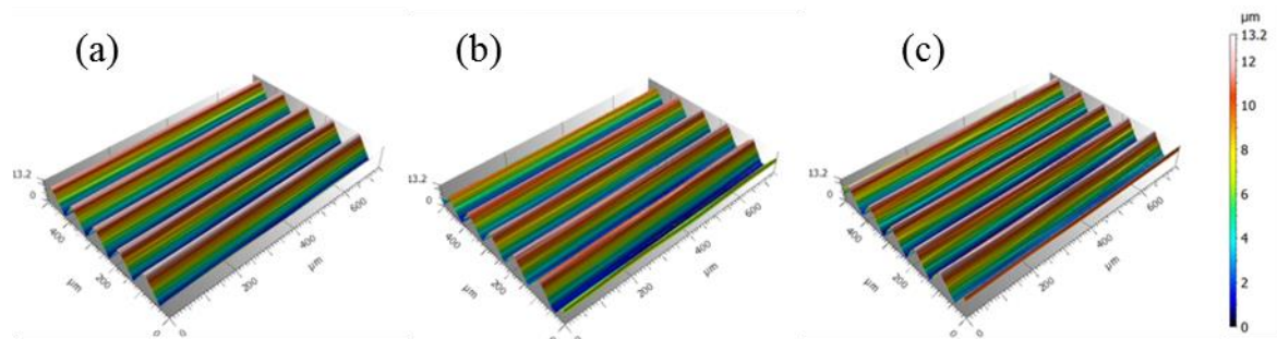
Figure 36. Areal surface topography of (a) CSI; and reconstructed SEM images from (b) PMF and (c) TA considering only the dominant wavelength. [71]
