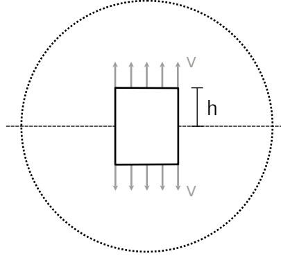
Figure A.7: Sketch of the cross-section of the 3D BEM model for investigating the effect of the protrusion of the sleeper through the infinite baffle. The top and bottom of the central box have a prescribed normal velocity v . The sound pressure is evaluated on a sphere with 30 m radius around the structure.
