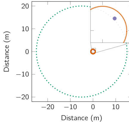
Figure A.4: Cross-section of the setup for the validation calculation. The thick blue dot marks the location of the line source. The smaller, orange circle represents the surface of the WBE structure while the larger, green circle of points are positions at which the sound pressure is evaluated.
