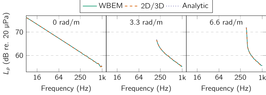
Figure A.5: Calculated pressure at one field point. The wavenumber \kappa along the structure is given in the top right corner.
