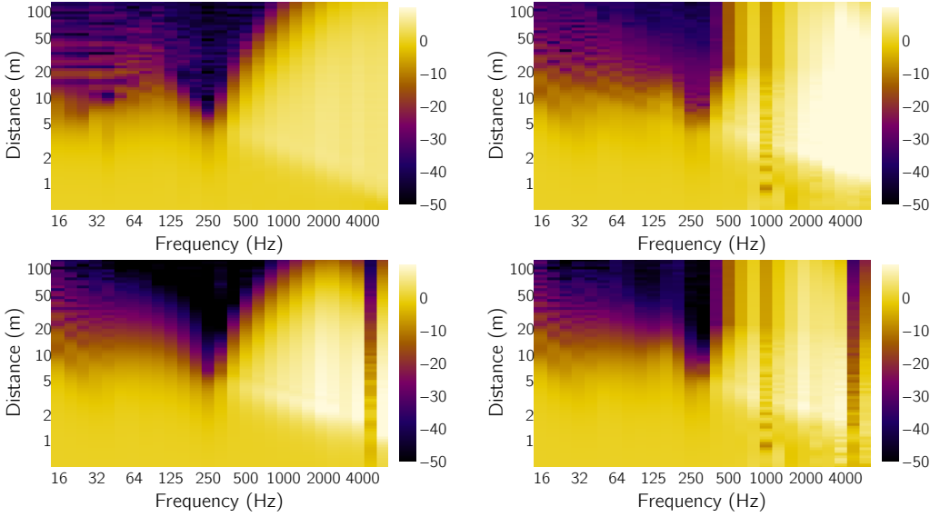
Figure 5.28: Decay of the sound pressure in a line along the track. Top: Beam models R2 and R3, bottom: WFE models R5 and R6. Each third octave band level is normalised to the level at 0 m.
