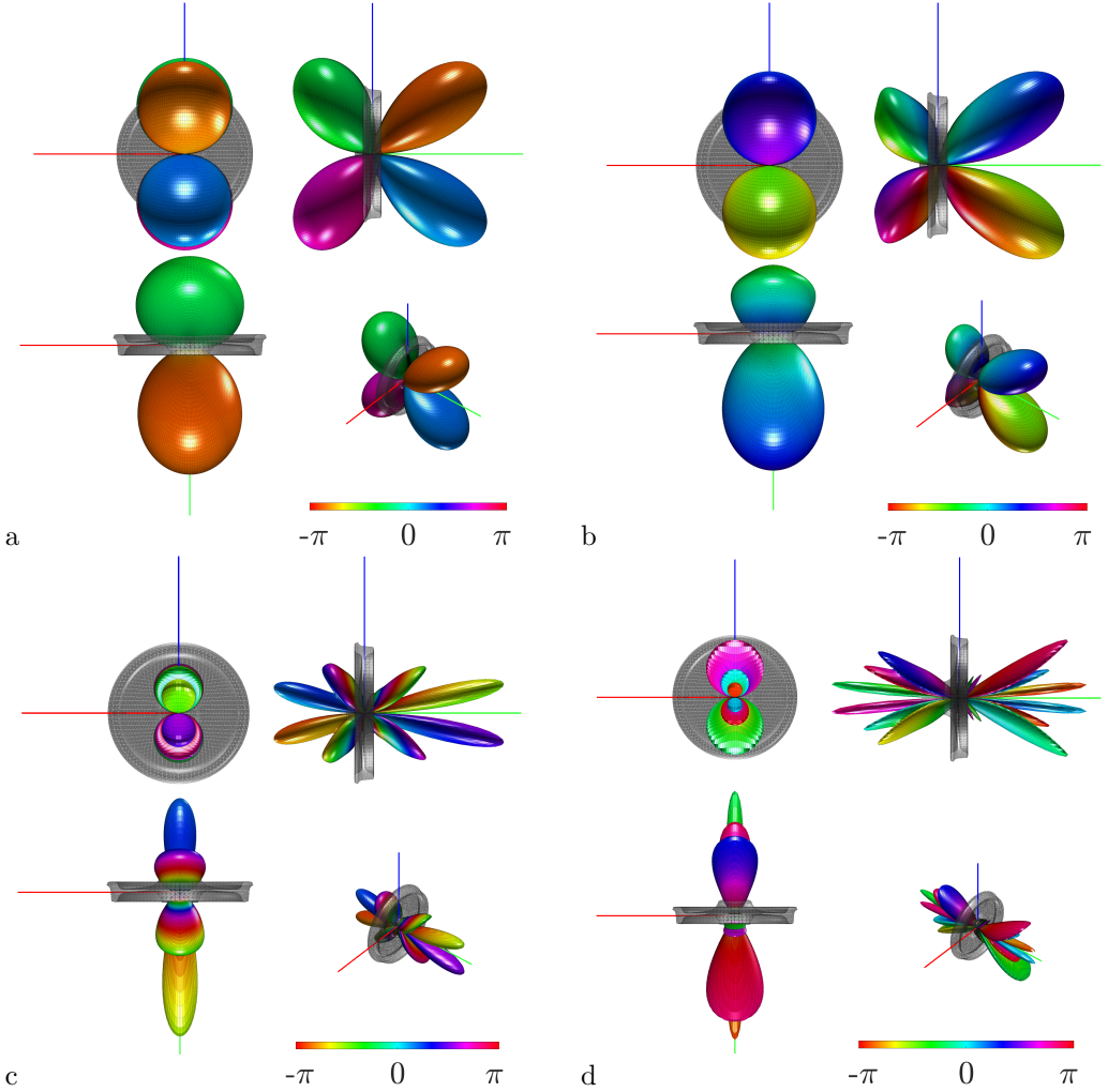
Figure 5.43: Directivity of the axial mode (1,0,a) for (a) 63 Hz, (b) 250 Hz, (c) 1000 Hz, and (d) 4000 Hz.
