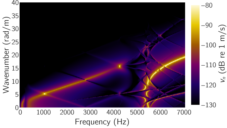
Figure 3.12: Normal velocity magnitude on top of the rail head over frequency and wavenumber for a discretely coupled rail.
