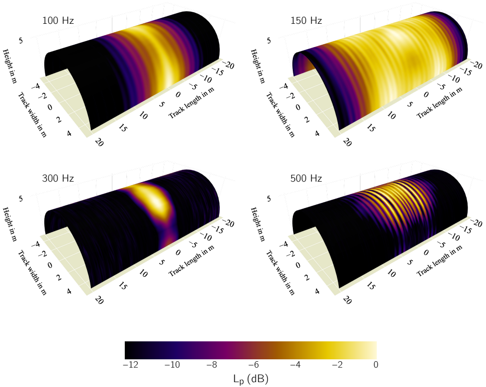
Figure 5.23: Sound pressure level on a 5 m cylinder around the track, created by the vibration of a series of 119 sleepers, coupled through a UIC 60 rail, which is excited with a vertical unit force, mid-span. The sound pressure level is normalized to 0 dB corresponding to the maximum L_p per frequency.
