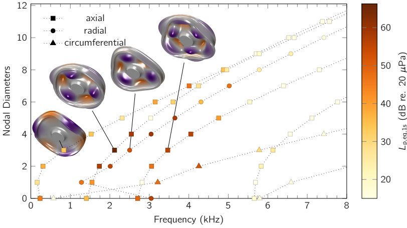
Figure 5.46: Contribution of each mode to the 1 s equivalent sound pressure level L_{p,eq,1s} .
