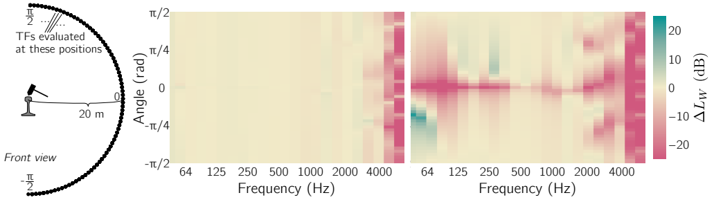
Figure 5.26: Difference of the sound pressure level at the half-circle of receiver points described on the left. Central image: central excitation on the rail head, right image: off-centre excitation.
