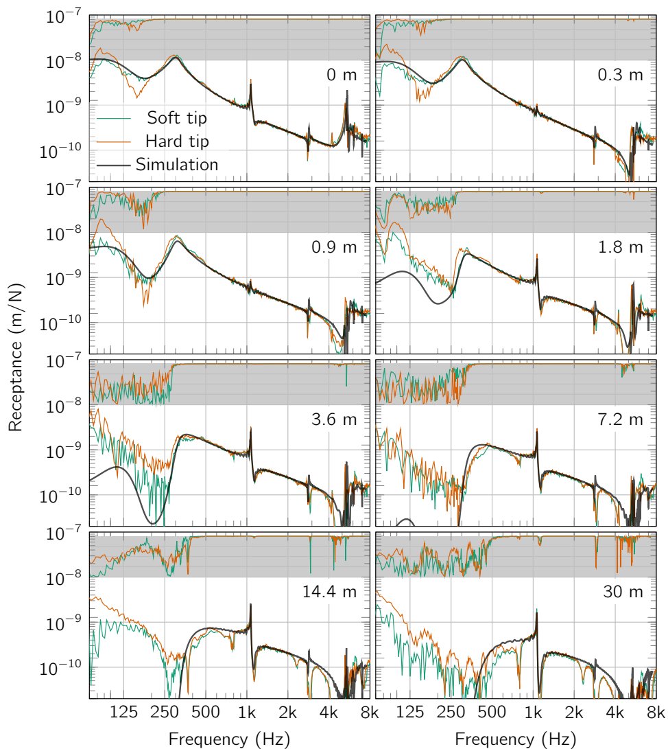
Figure 5.1: Measured and simulated vertical transfer functions of the ballasted track. 'Hard tip' and 'soft tip' refer to the impact hammer measurements with the corresponding hammer tip being used. The coherence of the respective measurement is indicated in the shaded rectangle at the top of each plot. The coherence takes values between zero and one, with one located at the top of the rectangle.
