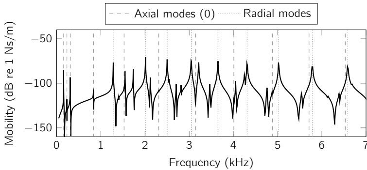
Figure 5.35: Radial input mobility of the wheel. The eigenfrequencies of radial modes and axial modes with zero nodal circles are indicated by vertical lines.
