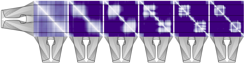
Figure 5.19: Transfer function from the velocity at each individual surface node (y-axis) to the sound pressure at each surface nodes (x-axis), displayed as the relative difference to the largest contribution, in dB. Left to right: 25 Hz, 500 Hz, 1000 Hz, 2000 Hz, 4000 Hz, and 7500 Hz.
