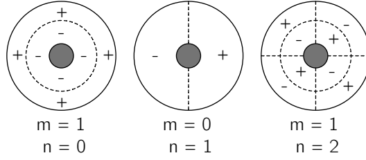
Figure 2.3: Sketch of the modes of a wheel characterized by their number of nodal diameters n and circles m , with a rigid axle in the centre.
