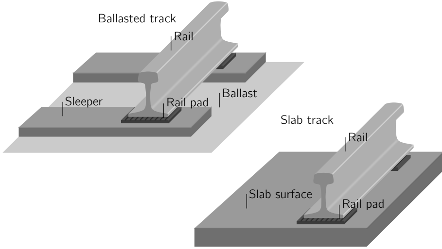
Figure 2.2: Considered components of ballasted and ballastless track systems that are included in the review.
