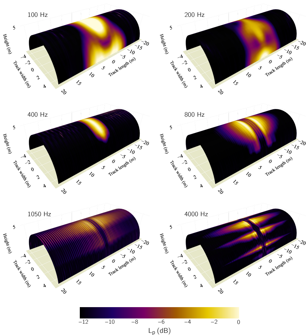
Figure 5.22: Sound pressure level on a 5 m cylinder around the track, created by the vibration of a UIC 60 rail excited with a vertical unit force, mid-span. The sound pressure level is normalized to 0 dB corresponding to the maximum L_p per frequency.
