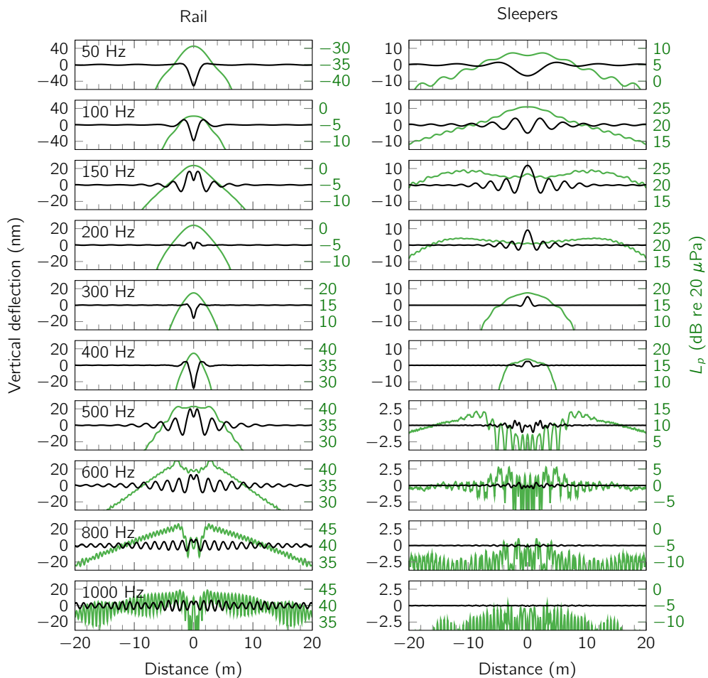
Figure 5.20: Rail and sleeper vertical deflection and sound pressure level measured in the (7.5 m, 1.2 m) standard position, along the track.
