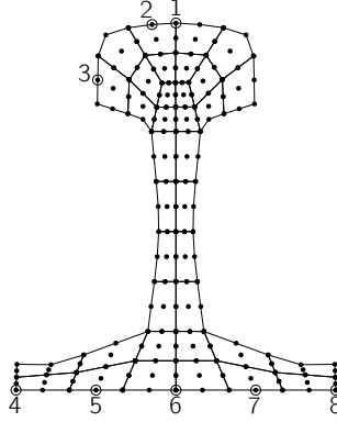
Figure 3.2: Discretised cross-section of the UIC60 rail geometry. Numbered nodes are referred to below.
