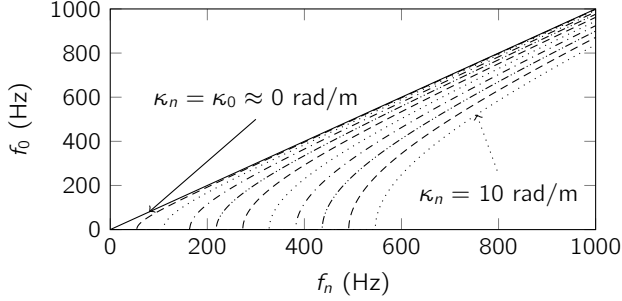
Figure 3.10: Mapping between f_n and f_0 for selected whole wavenumbers k_n 0 rad/m to 10 rad/m.
