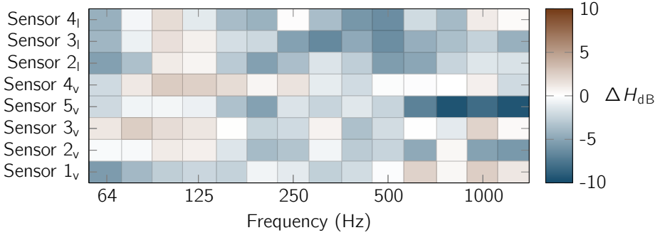
Figure 5.6: Difference between the predicted and measured transfer functions from a vertical excitation at \Pi_c to all sensors.
