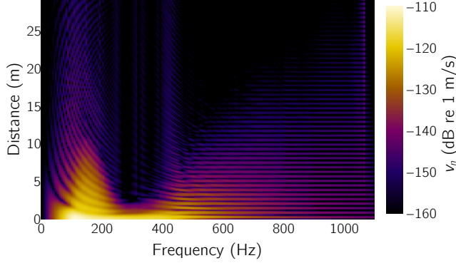
Figure 3.18: Sleeper velocity profile, neglecting wavenumbers that do not contribute to sound radiation.
