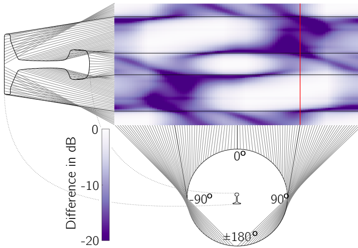
Figure 5.17: Transfer function magnitude between each source element on the rail and receiver point in a circle with 20 m radius around the the rail. The displayed transfer functions are calculated at 1100 Hz, which is typically close to the pinned-pinned frequency.
