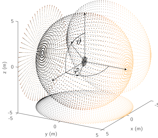
Figure 4.2: Position of the wheel and the receiver points on the reference surface in the FBEM calculation. Projections of the receiver points are included for orientation.
