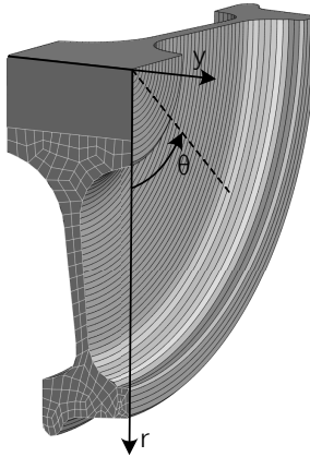
Figure 4.1: The curved waveguide model of the wheel. The cross-section is located in the (y, r) -plane.
