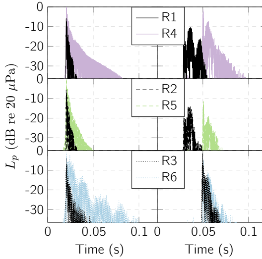
Figure 5.30: Comparison of the pressure impulse responses at 1 m and 64 m for different track models.
