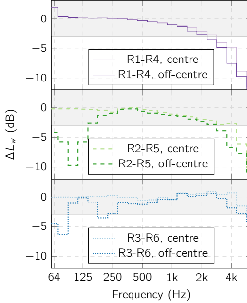
Figure 5.25: Difference between predicted radiated sound power of the beam models to the WFE model, per support type.
