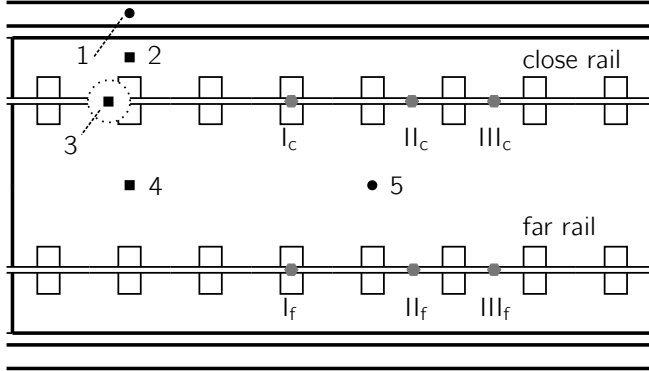
Figure 5.4: Locations of accelerometers and excitations in the measurement.
