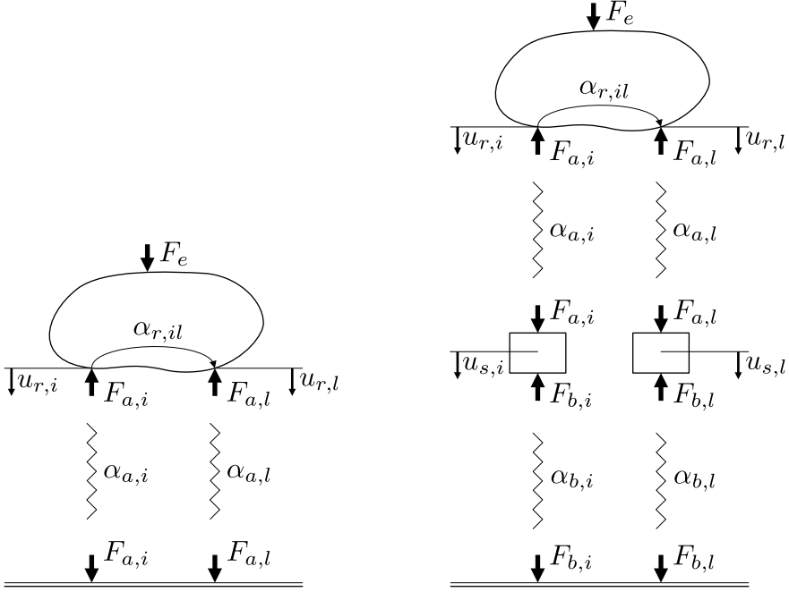
Figure 3.7: Discrete coupling in configuration a (left) and b (right).
