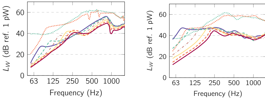
Figure 5.9: Radiation from a 20 cm slab at vertical excitation on the rail for different rail pad stiffnesses k_s : 10 kN/mm (—), 20 kN/mm (---), 40 kN/mm (-.-), 80 kN/mm (—), 160 kN/mm (···) and 320 kN/mm (—). Lateral excitation included for 20 kN/mm (····) and 160 kN/mm (····). Left: Discrete support, Right: Continuous Support.
