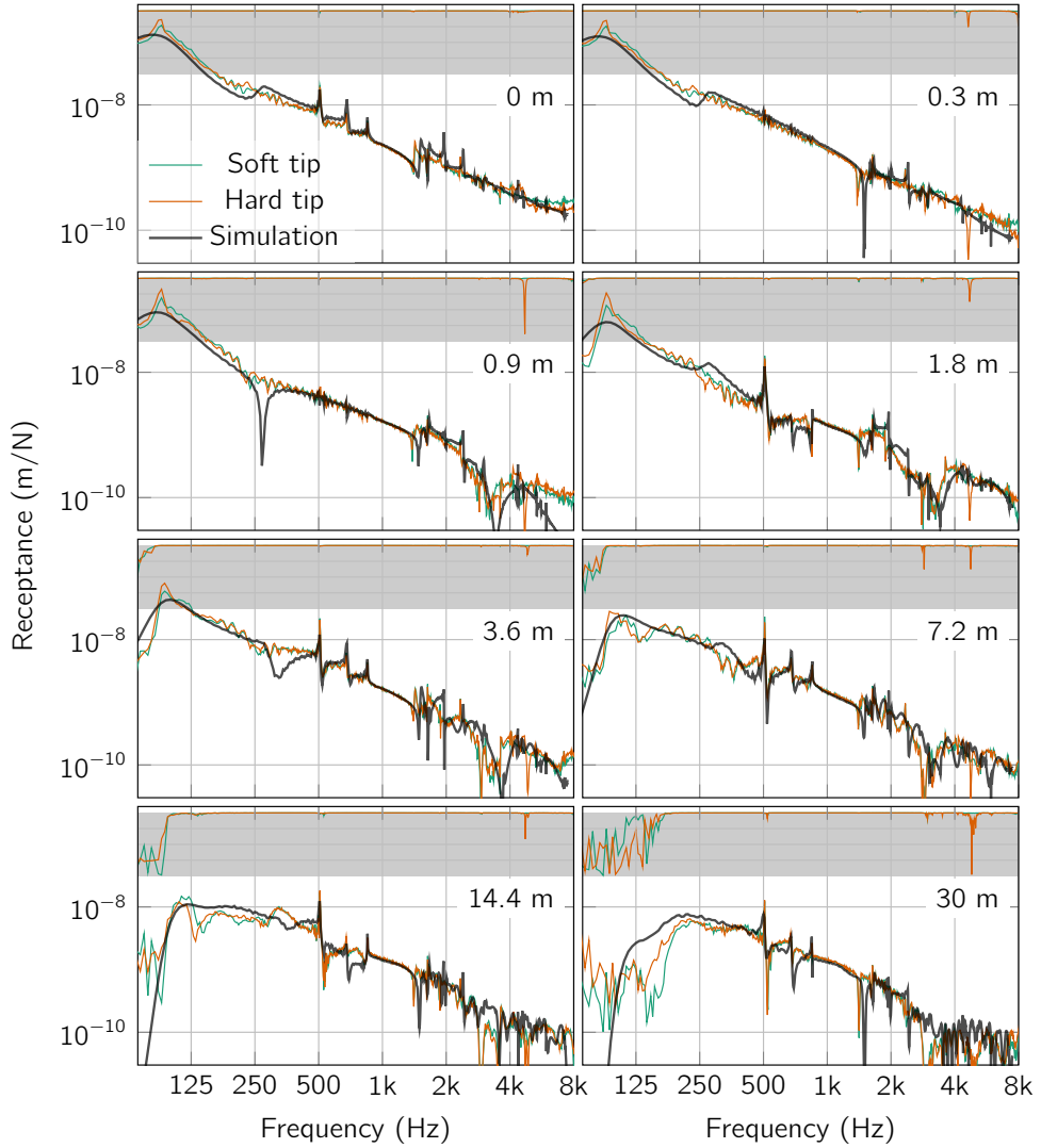
Figure 5.2: Measured and simulated lateral transfer functions of the ballasted track. 'Hard tip' and 'soft tip' refer to the impact hammer measurements with the corresponding hammer tip being used. The coherence of the respective measurement is indicated in the shaded rectangle at the top of each plot. The coherence takes values between zero and one, with one located at the top of the rectangle.
