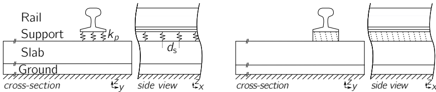
Figure 5.8: Model setup for the discretely (left) and continuously (right) supported rail. The lateral springs are not shown in the left image.
