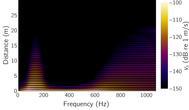
Figure 3.15: Sleeper velocity profile over space and frequency, for a unit force harmonic excitation at x = 0 m. Only half the considered track section is shown.
