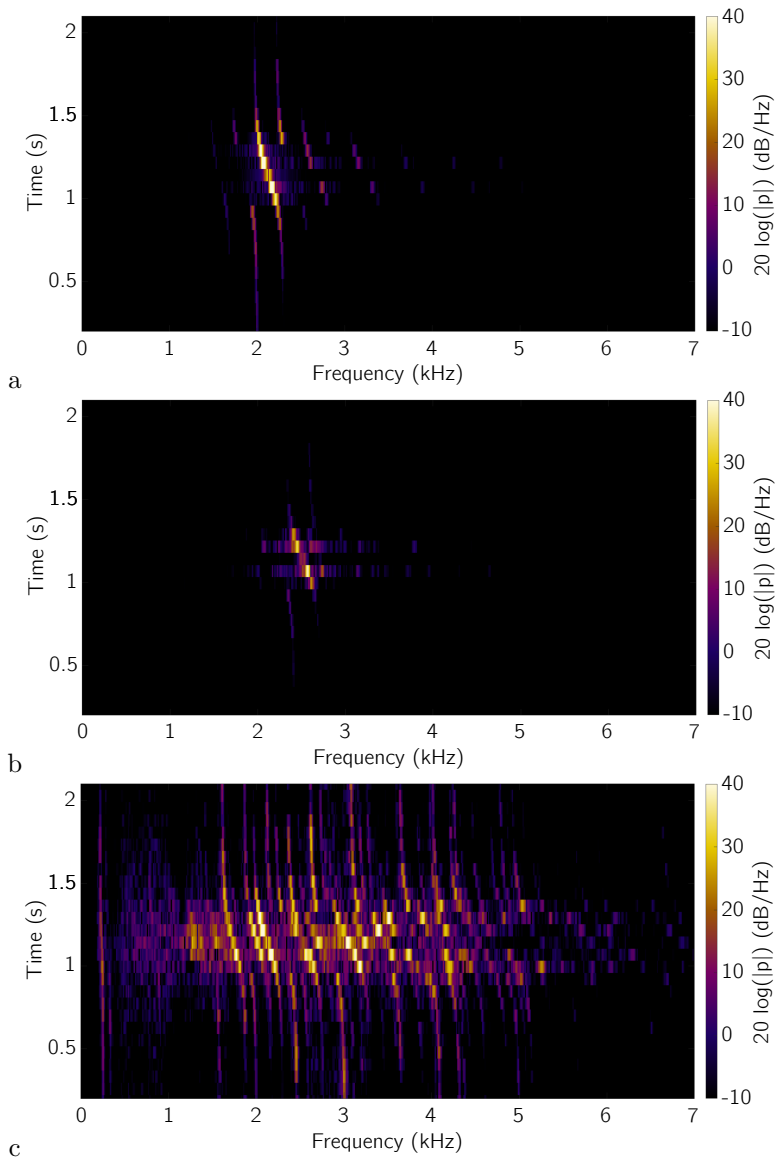
Figure 5.48: Spectrogram of a the pass-by sound pressure at a stationary microphone position. Top (a): mode (3,1,a), (b) mode (3,0,r), (c) total.
