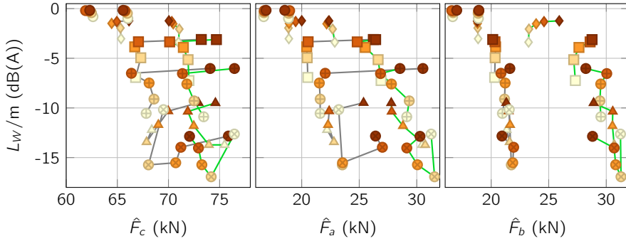
Figure 5.14: Comparison of the maximum forces in the rolling contact \hat{F}_c (left), the rail seat \hat{F}_a (centre), and into the slab \hat{F}_b (right) to L_W . The symbols' colours indicate the mass (□ ■ ■ ■ ■ for 8 kg, 16 kg, 32 kg, 64 kg and 128 kg, respectively), and their shapes represent different rail pad stiffnesses k_a (○ ◇ □ ⊕ △ ⊗ for 25 kN/mm to 800 kN/mm, respectively). The line color indicates the stiffness k_b , (— — for 20 kN/mm and 40 kN/mm, respectively).
