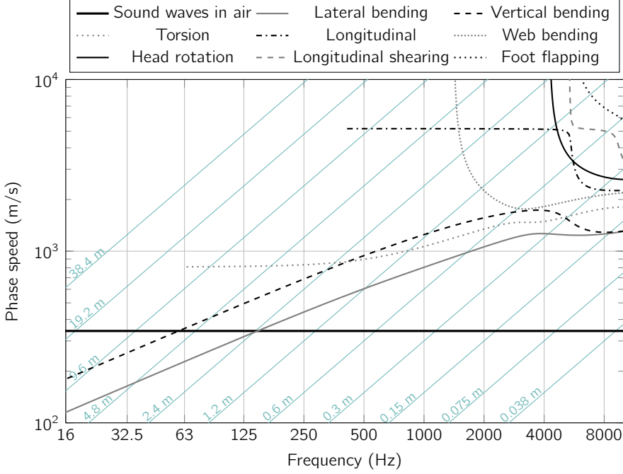
Figure 3.5: Frequency dependent phase speed of the waves in a free UIC60 rail. The diagonals lines indicate corresponding wavelengths.
