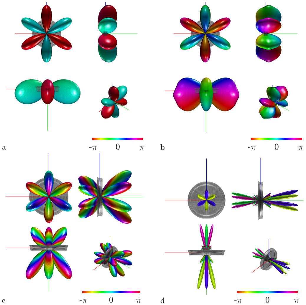
Figure 5.44: Directivity of the axial mode (3,1,a) for (a) 63 Hz, (b) 250 Hz, (c) 1000 Hz, and (d) 4000 Hz.
