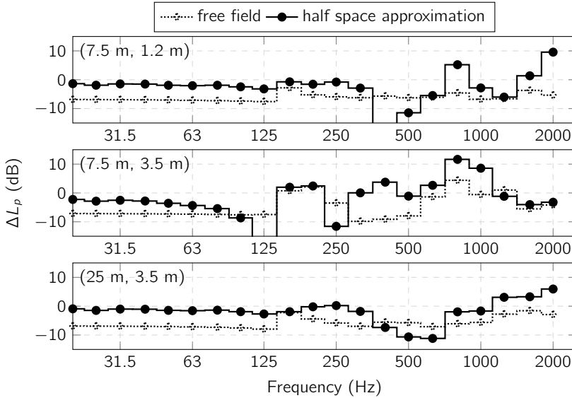
Figure 5.42: Free-field and mirror-source approximation compared to the coupled half-space solution.
