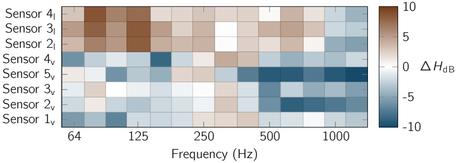
Figure 5.7: Difference between the predicted and measured transfer functions from a lateral excitation at \Pi_c to all sensors.
