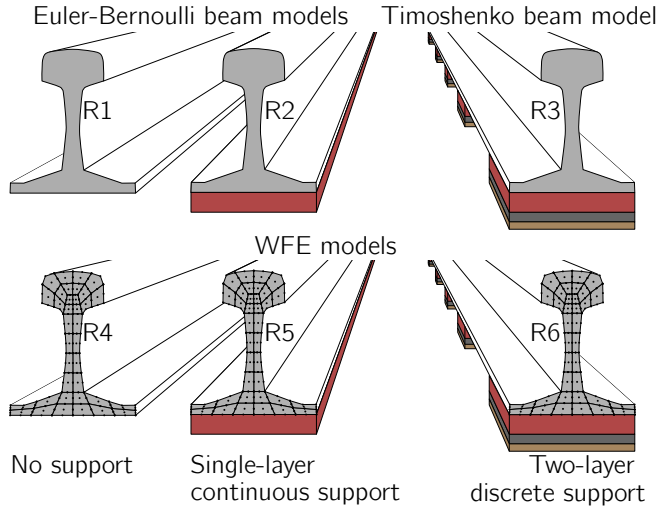
Figure 5.24: Considered track models included in the study.
