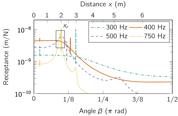
Figure 5.21: The top of rail vertical receptance in wavenumber domain, plotted over the angle \beta . The frequencies are chosen below, close to, and above the cut-on frequency of vertical bending waves. The sharp peaks at around \pi/8 radians, and the other maxima visible for 500 Hz and 750 Hz are an effect of the torsional and lateral bending wave.
