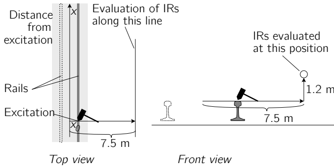
Figure 5.27: Location at which the impulse responses are evaluated.
