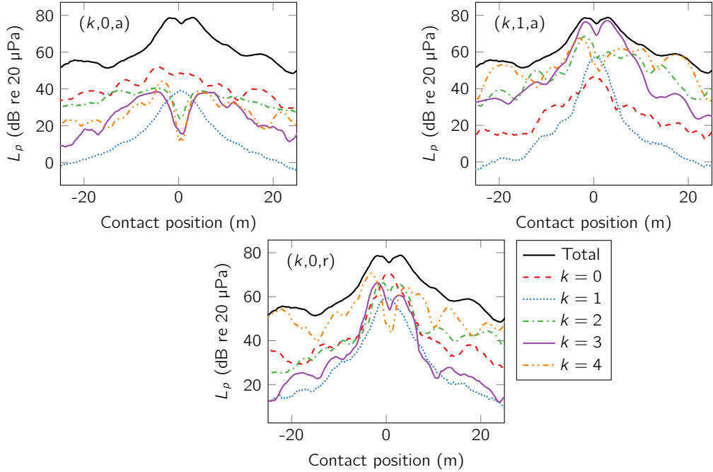
Figure 5.45: Contribution of each individual mode to the pressure during the pass-by of the wheel. The upper figures show axial modes with varying pressure numbers of nodal diameters k , for zero and one nodal circles. The lower figure presents the first few radial modes.
