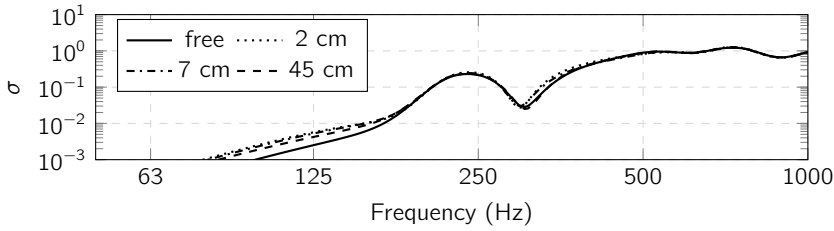
Figure 5.39: Radiation ratio \sigma for different heights of the reflective plane. The wheel is excited radially in the contact point.
