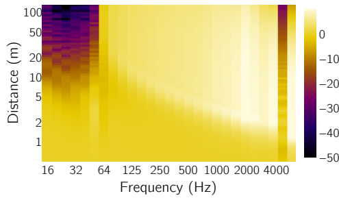
Figure 5.29: Decay of the sound pressure produced by a WFE-based rail that is acoustically free in space. Each third octave band level is normalised to the level at 0 m.
