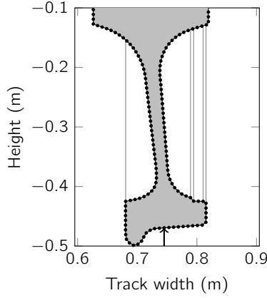
Figure 5.32: Lower part of the wheel cross-section, where the centre axis of the wheel is located at 0 m height. The arrow indicates the assumed contact location.
