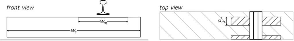
Figure 5.11: Sketch of the radiating surfaces, including a rail and an approximation of a track superstructure on which normal velocities are specified. An acoustically hard surface is included via half-space Green’s functions.
