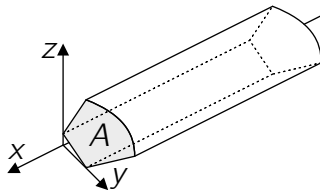
Figure 3.1: Orientation of the coordinate system in the WFE method (adapted from [42]).
