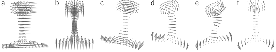
Figure 3.3: Cross-sectional deflections of selected wave types: a - lateral bending, b - vertical bending, c - torsion, d - web bending, e - head rotation, f - foot flapping.
