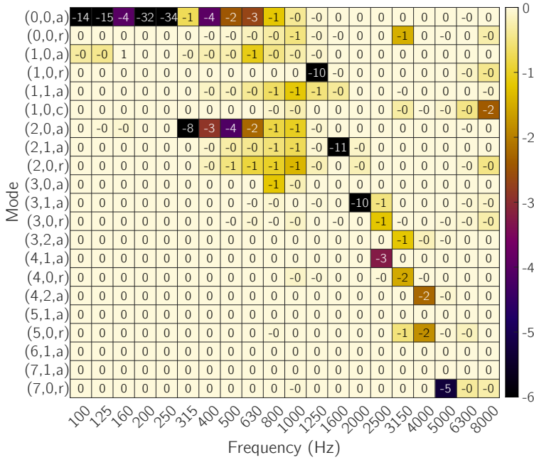
Figure 5.47: Effect of removing the contribution of a single mode on the L_{p,eq,1s} , in dB. The figure contains only a selection of modes, as modes with a negligible effect are not shown.
