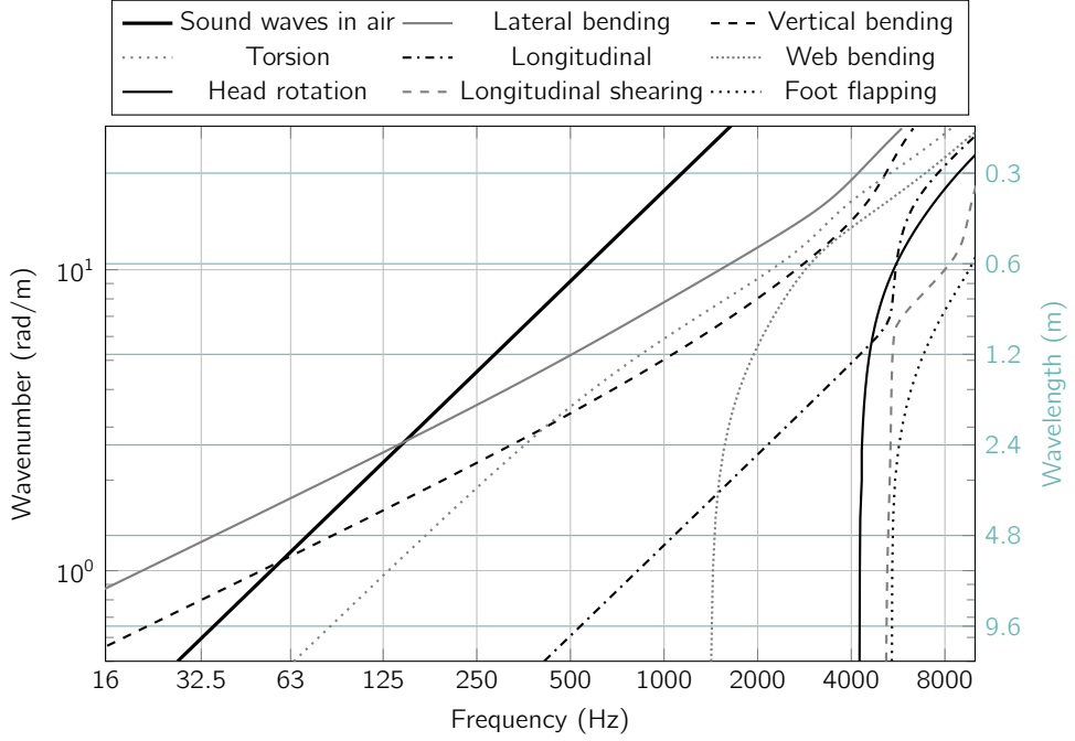
Figure 3.4: Dispersion relation of the waves in a free UIC60 rail. The corresponding wavelengths are indicated on the right.
