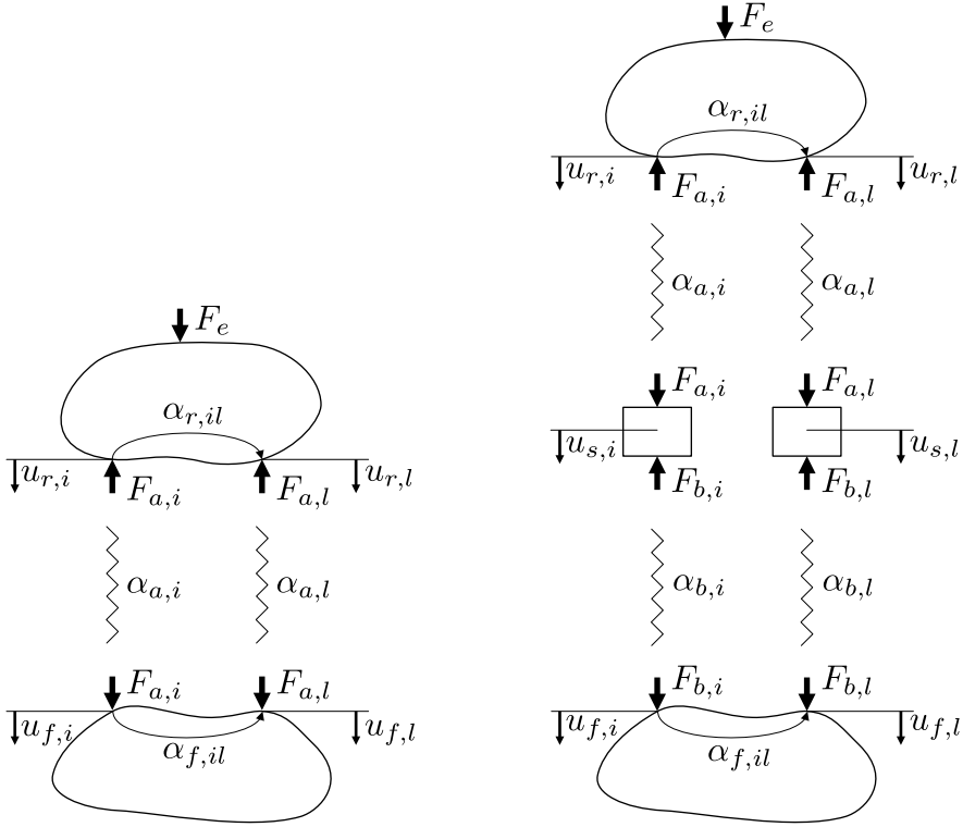
Figure 3.8: Discrete coupling in configuration c (left) and d (right).
