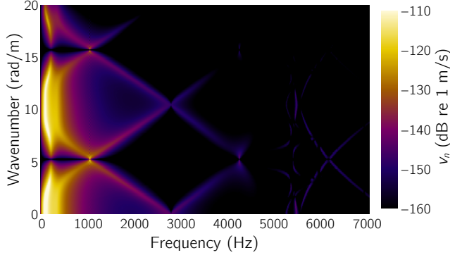
Figure 3.16: Vertical normal velocity profile of the track in the wavenumber-frequency domain.
