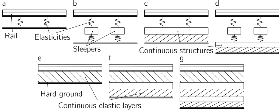
Figure 3.6: Rail support configurations a to g. The shaded areas represent continuous supports.
