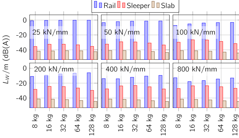
Figure 5.13: Normalised sound power radiated from the different components for different k_a as indicated in each top left corner. These are results for k_b = 40 kN/mm.
