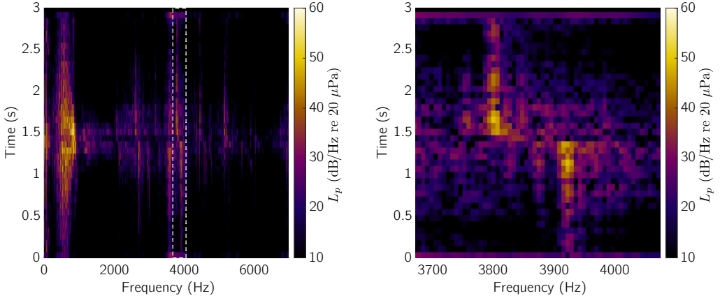
Figure 5.31: Spectrogram of the generated pressure signal at a stationary microphone during the pass-by of a moving force.
