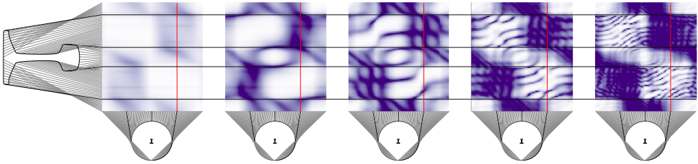
Figure 5.18: Transfer function from surface velocity on each individual node on the rail surface (y-axis) to the sound pressure in a circle around the rail (x-axis), displayed as the relative difference to the largest contribution, in dB. Left to right: 500 Hz, 1000 Hz, 2000 Hz, 4000 Hz, and 7500 Hz. The receiver angle zero degrees corresponds to a position vertically above the rail and increasing numbers indicate clockwise rotation.
