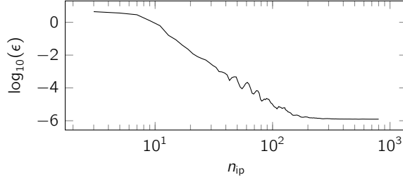
Figure A.3: Quality of integration in dependency of the number of integration points when using the resulting \kappa_{\min} and \kappa_{\max} found in the genetic algorithm.
