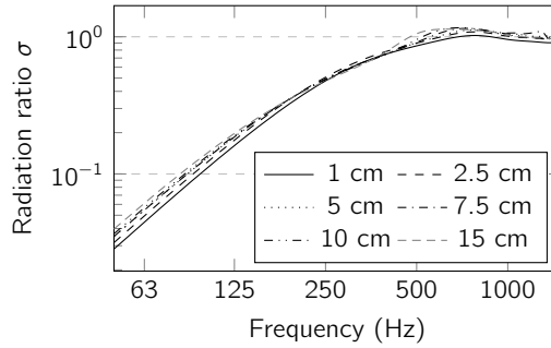
Figure A.8: Radiation efficiency \sigma for different heights of the sleeper.
