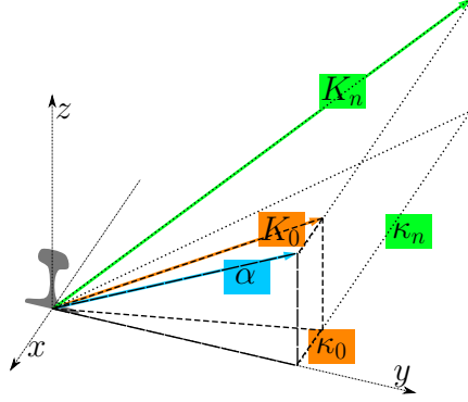
Figure 3.9: Relation between K , \kappa , and \alpha , corresponding to the wavenumbers in air, along the track, and in the (y, z) -plane, respectively.
