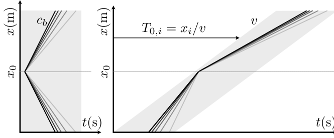
Figure 3.20: Aligning impulse responses to the velocity of a passing force to compute the pass-by pressure signal. Left: Impulse response matrix g_{da} , where diagonal lines symbolise the arrival of wave fronts at x_0 for an excitation at x . Right: Aligning the impulse responses with the location of the moving excitation force in space and time.
