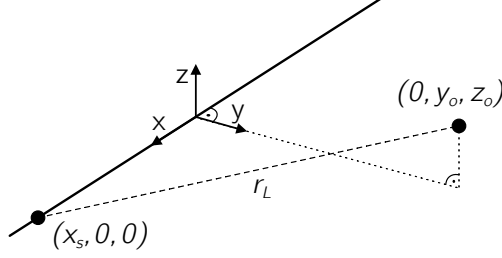
Figure 4.3: Axis definition and position of the wheel and stationary microphone. The solid line indicates the trajectory of the wheel.
