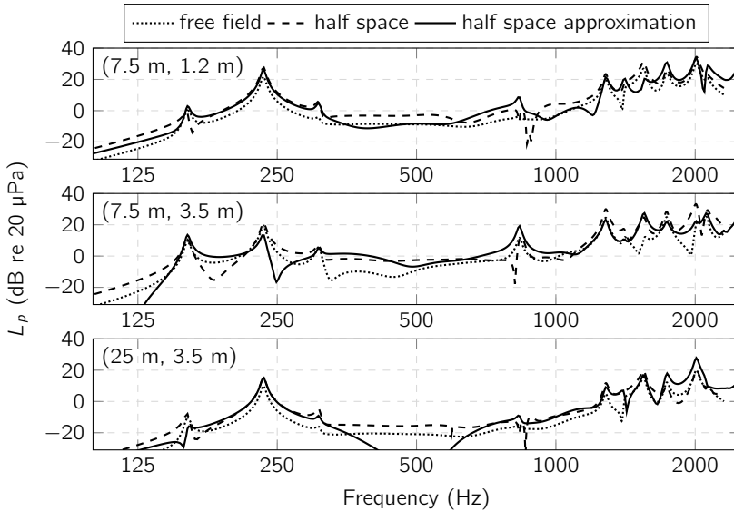
Figure 5.41: Calculated sound pressure level at three standard measurement positions for three different acoustic geometries: the wheel in free space, half-space with a perfectly reflecting boundary, and an approximation of the half-space by adding the mirrored sound field of the free wheel.
