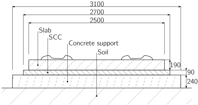
Figure 5.3: Cross-section of the CRTS-III track. Dimensions in mm.
