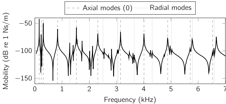
Figure 5.36: Axial input mobility of the wheel. The eigenfrequencies of radial modes and axial modes with zero nodal circles are indicated by vertical lines.
