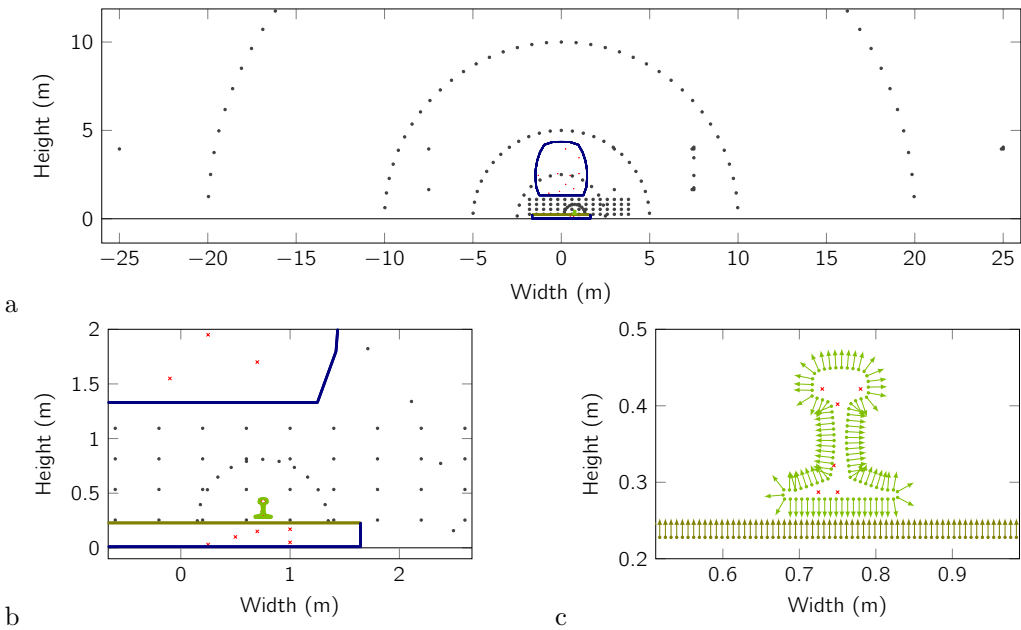
Figure 5.16: Setup (iv) for which the acoustic transfer functions were evaluated.
