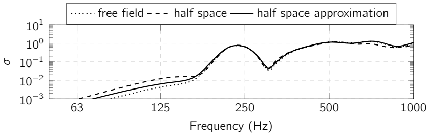
Figure 5.40: Radiation ratios for the radiation into free field and half space, comparing the fully coupled solution to the approximation via mirror sources. The excitation is axial at the contact point.
