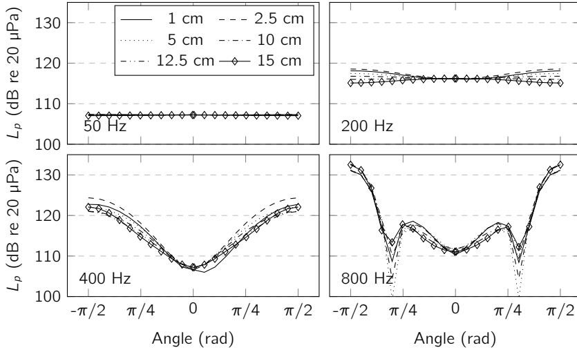
Figure A.9: Directivity of a rectangular piston protruding an infinite baffle with different heights at selected frequencies.
