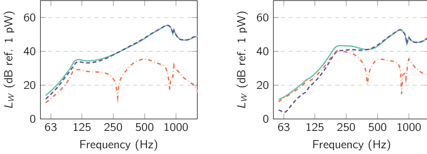
Figure 5.10: Contribution of rail (---) and slab (-.-) to the total radiated sound power (—) in case of a discretely supported rail on a 20 cm thick slab. Left: k_p = 20 kN/mm, Right: k_p = 80 kN/mm.
