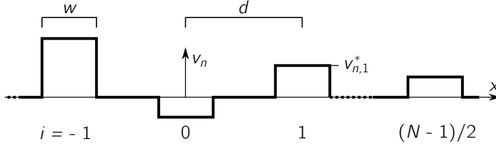
Figure 3.14: Normal velocity slice v_n over the length of the considered track section due to the vertical velocity at each sleeper.
