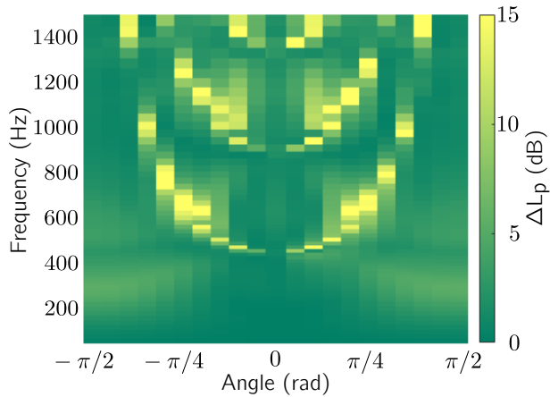
Figure A.10: Maximum sound pressure difference between the sleepers with different heights over frequency and angle.
