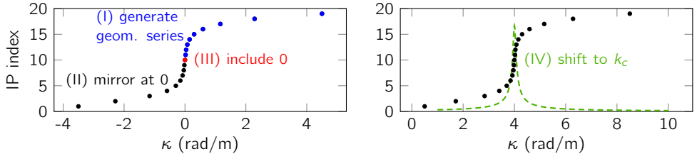
Figure A.1: Example distribution of integration points around k_c = 4 rad/m.
