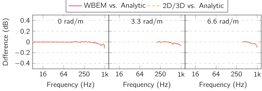
Figure A.6: Comparison of the mean difference at all field points.
