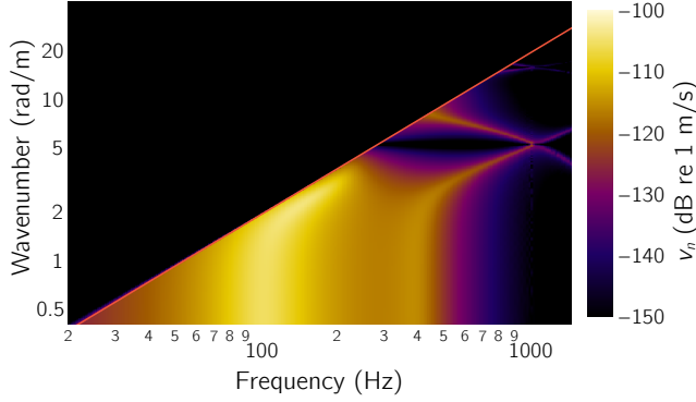
Figure 3.17: Velocity profile in frequency-wavenumber domain, including only wavenumbers relevant for sound radiation. The red line indicates the wavenumber in air. Note the logarithmic frequency axis.
