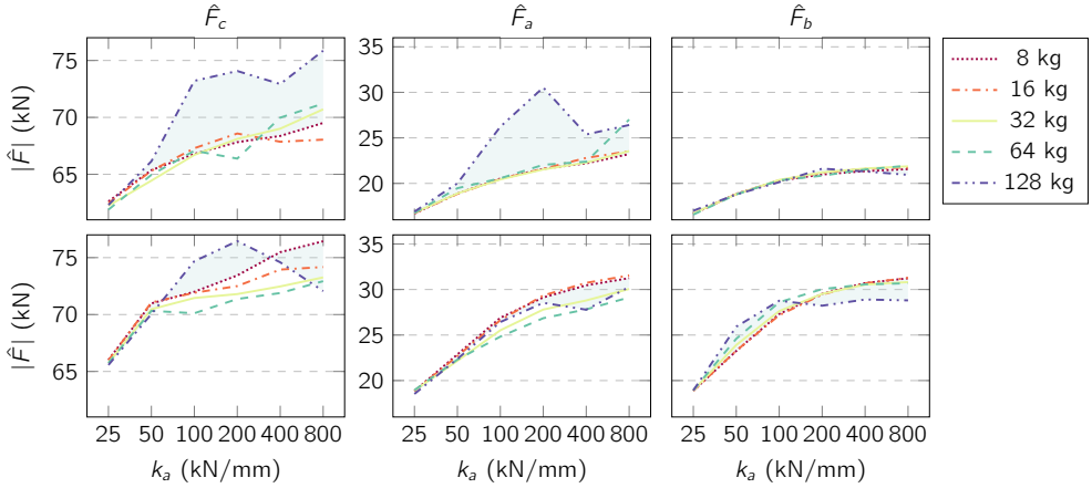
Figure 5.12: Influence of the support parameters on the peak forces \hat{F}_c , \hat{F}_a , and \hat{F}_b . For orientation, the area between the lightest and the heaviest mass is coloured in blue. Top: k_b = 20 kN/mm, bottom: k_b = 40 kN/mm.
