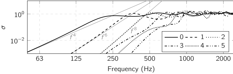
Figure 5.38: Radiation ratio \sigma of the wheel for different numbers of nodal diameters and radial excitation at the contact point. The slopes of the functions proportional to f^4 , f^6 , and f^8 are included as a reference.
