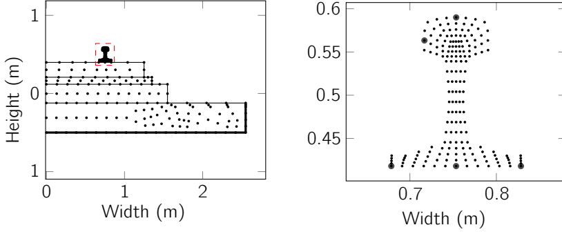
Figure 5.5: FE nodes of the cross-section of the slab track model. The thick nodes on the rail head mark excitation positions, and the ones on the rail foot mark the nodes at which the rail was connected to the slab via the rail pad stiffness. Only half of the symmetric slab track is shown.
