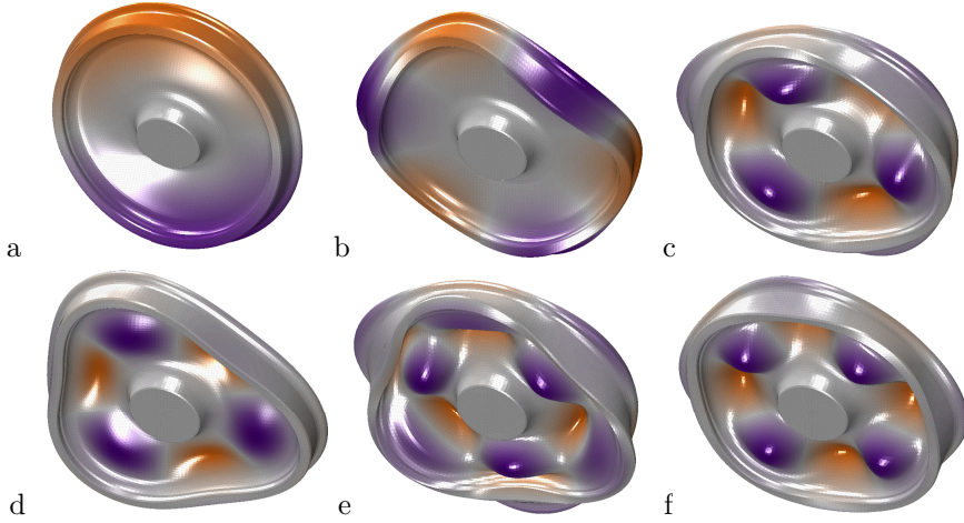
Figure 5.34: Vibrational mode shapes of the wheel. a) (1,0,a) , b) (3,0,a) , c) (3,1,a) , d) (3,0,r) , e) (3,2,a) , f) (4,1,a) . The colour indicates axial deflection.
