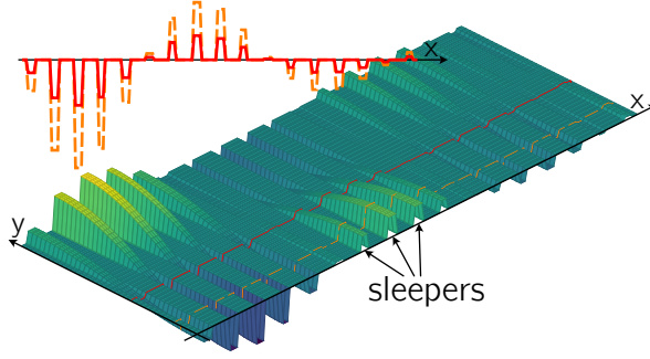
Figure 3.13: Example velocity profile along the length of the track, assuming monoblock sleepers. Each slice along the track produces a different profile, which can be expressed as a wavenumber spectrum.
