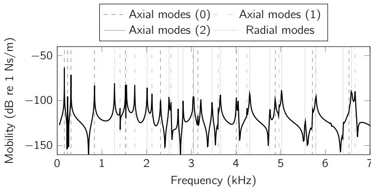
Figure 5.37: Vertical to lateral cross-mobility of the contact position. The eigenfrequencies of radial modes and axial modes with zero, one and two nodal circles are indicated by vertical lines.
