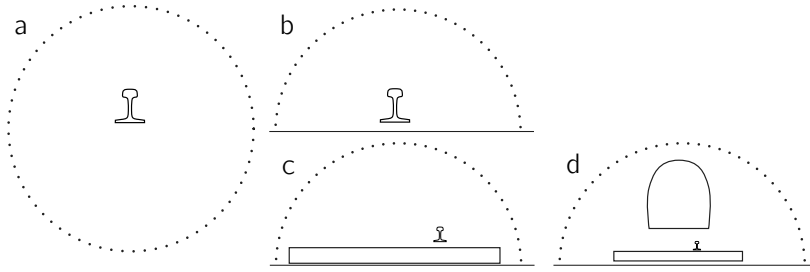
Figure 5.15: BE geometries for which the acoustic transfer-functions have been precalculated.
