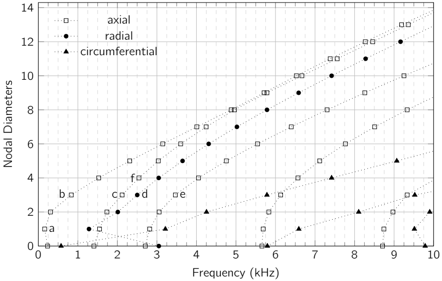
Figure 5.33: Dispersion relation of the eigenfrequencies of the wheel.
