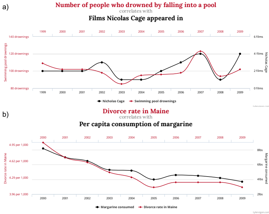
Figure 3.1: Two different examples when correlation does not imply causation . Source: https://matt-rickard.com/correlation-vs-causation
