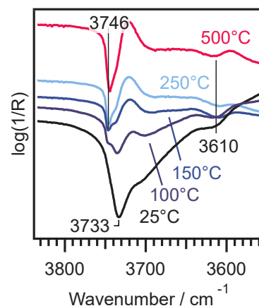
Figure 4.4: Background subtracted DRIFT spectra of pre-adsorbed 2,5-dmf on H-BEA(37) and signal evolution upon temperature increase.[139]
