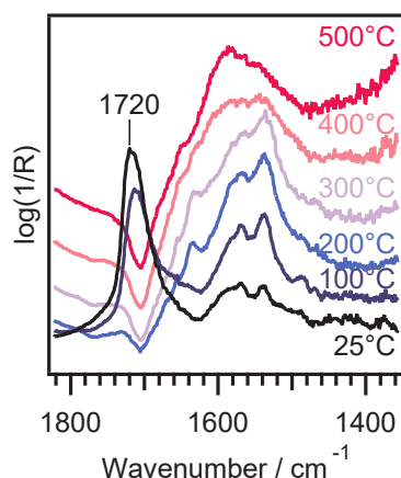
Figure 4.17: Background subtracted DRIFT spectra of pre-adsorbed 2,5-dmf on H-BEA(37) and signal evolution upon temperature increase.[139]
