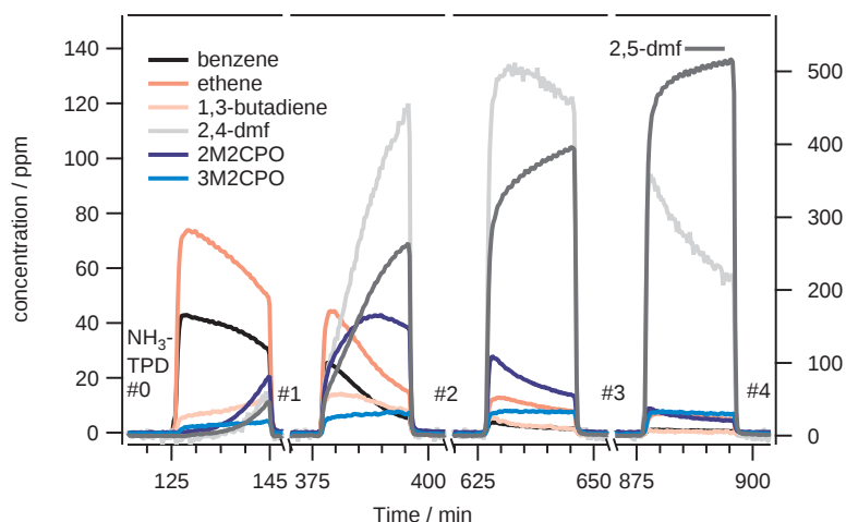
Figure 4.12: Concentration profiles of various species during 20 min 2,5-dmf pulses intermitted by NH 3 -TPD (see Figure 4.11); catalyst: H-ZSM-5(38) 300 \mu m to 355 \mu m.
