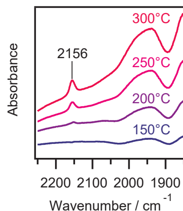
Figure 4.7: Observation of C=O stretch vibration on Cu at 2156\text{ cm}^{-1} in a DRIFTS experiment. Difference spectra, background at 25^\circ\text{C} . [139]
