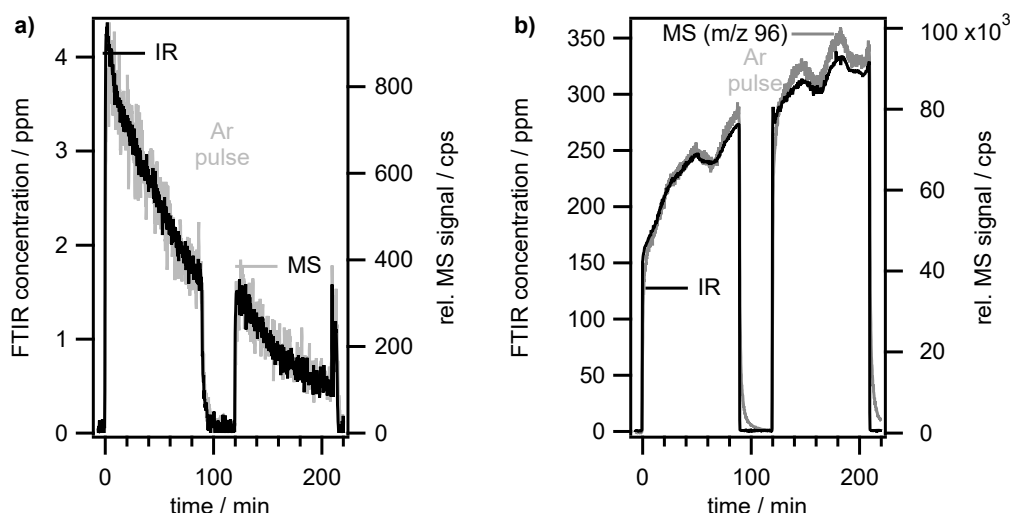
Figure 3.7: Comparison of FTIR and MS: Signal match of IR and MS for a) ethene ( m/z 27) and b) 2,5-dimethylfuran ( m/z 96).[100]
