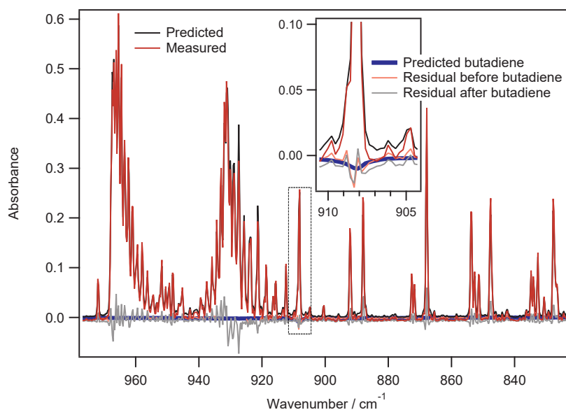
Figure 3.10: Measured, predicted and residual spectra showing false negative predicted spectra during the quantification of the butadiene signal due to interference with the ammonia band around 908\text{ cm}^{-1} .
