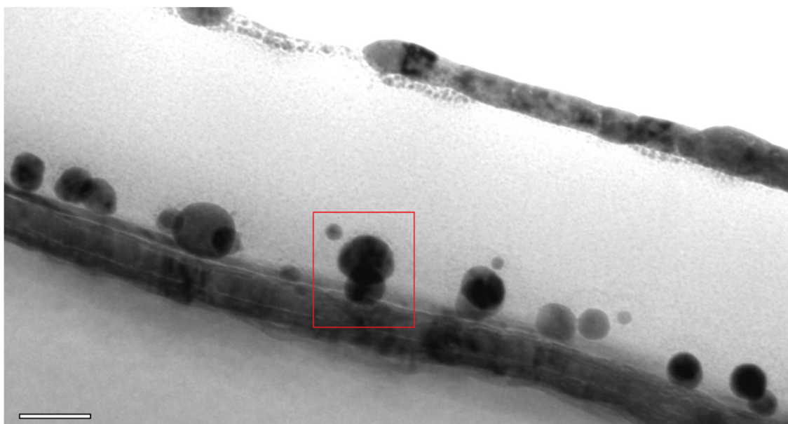
Figure 10: TEM micrograph of sample lifted-out from silica embedded surface with gold nanoparticles modified by thiol-streptavidin and biotinylated 10 nm gold nanoparticles. In the highlighted region, the distance between the larger and the smaller nanoparticle corresponds well to the size of the streptavidin-biotin complex. Scale bar: 50 nm.
