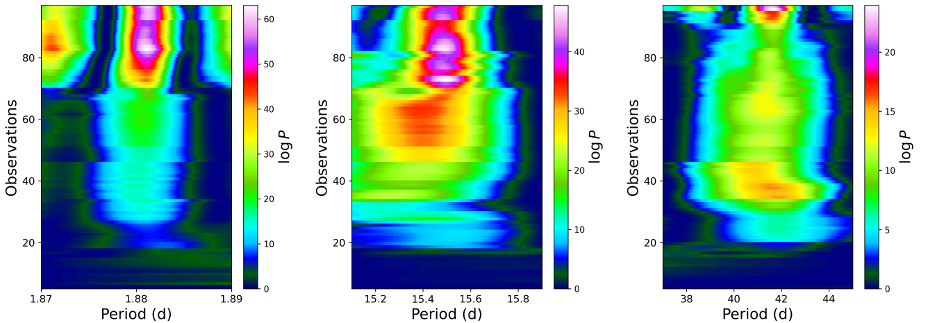
Fig. 9. Evolution of the s-BGLS periodogram for the CARMENES VIS plus MAROON-X RV data of TOI-1468 around the inner planet signal of 1.88 d (left), the outer planet signal of 15.53 d (middle), and the stellar rotation signal of \sim 41 d after removal of both planetary signals (right).
