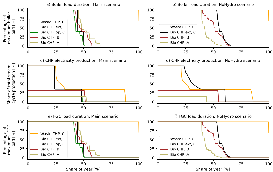
Fig. 9. Duration curves for: a and b) boiler load; c and d) electricity production; and e and f) flue gas condenser load, for the Main and NoHydro scenarios. The letters A, B and C correspond to the small, medium and large district heating subsystems, respectively, while “Bio” denotes wood chips. Note that the durations cover the whole year and not only the operational hours of the plant, i.e., the electricity production level and FGC load should be compared to the boiler load duration. Turbine types: bp, backpressure; ext, extraction.
