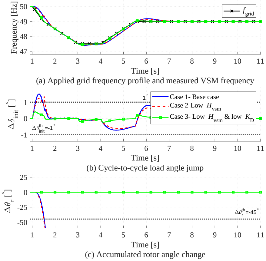
Figure 4.14: Impact of grid frequency variation on the composite VVS-based island detection for a \Delta P_{\text{vsm}} = 25\%S_b . (Case 1- H_{\text{vsm}} = 3 s, K_D = 89.40 p.u., \alpha_f = 1.86 rad/s. Case 2- H_{\text{vsm}} = 0.1 s, K_D = 89.40 p.u., \alpha_f = 1.86 rad/s. Case 3- H_{\text{vsm}} = 0.1 s, K_D = 17.88 p.u., \alpha_f = 1.86 rad/s.)
