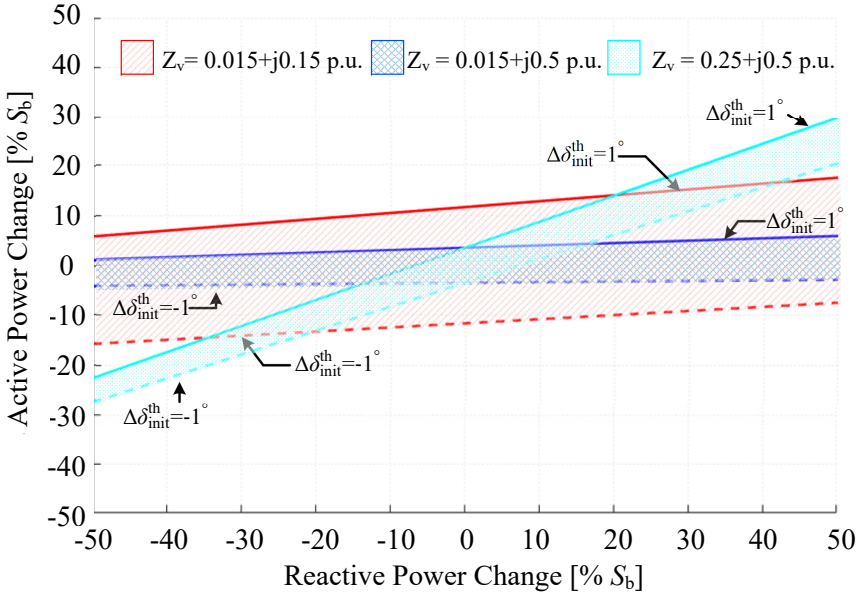
Figure 3.2: Non-detection zone of VVS-based island detection method at different virtual impedance.
