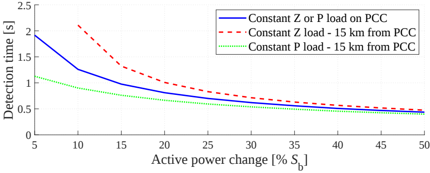
Figure 4.12: Island detection time vs. active power change for constant power and constant impedance load connected at PCC and 15 km away from PCC.
