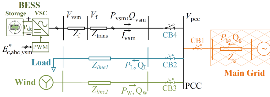
Figure 4.1: Single Line Diagram- Case Study System
