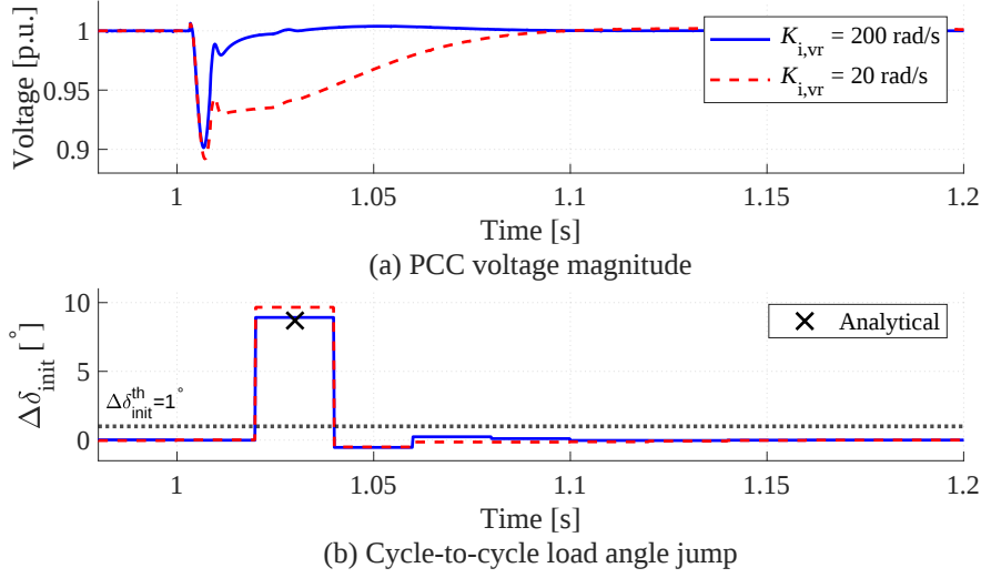
Figure 4.5: Impact of two different voltage controller integral gains on the voltage magnitude and the cycle-to-cycle change in the load angle for \Delta P_{vsm} = 30\%S_b
