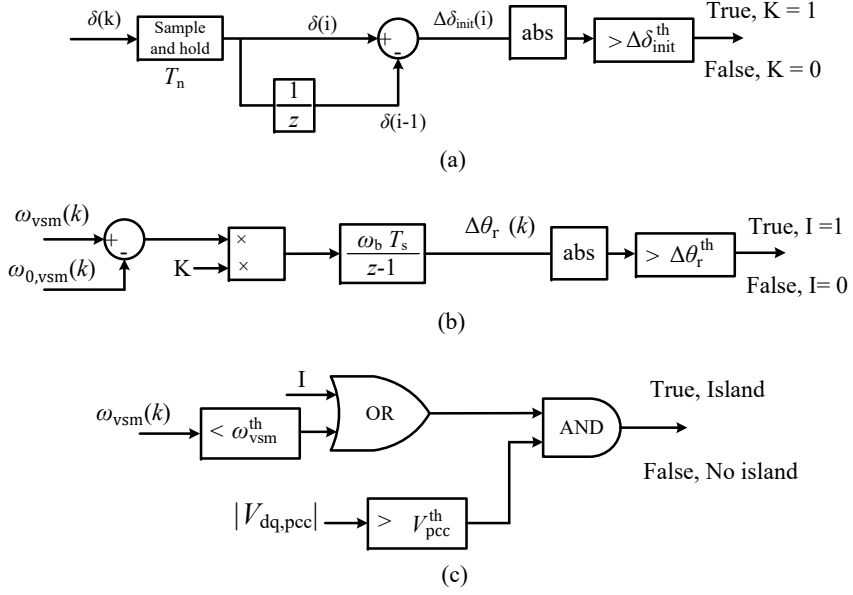
Figure 3.4: Implementation of composite passive island detection method
