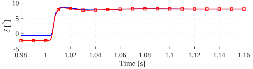
(c) PQ-based estimated load angle
