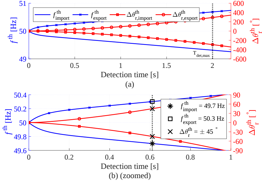
Figure 3.3: Equivalent threshold settings for \Delta f -based and \Delta\theta_r -based island detection for \Delta P_{\text{vsm}} = \pm 30\% S_b , H_{\text{vsm}} = 3 s, K_D = 89.40 p.u., \alpha_f = 1.86 rad/s.
