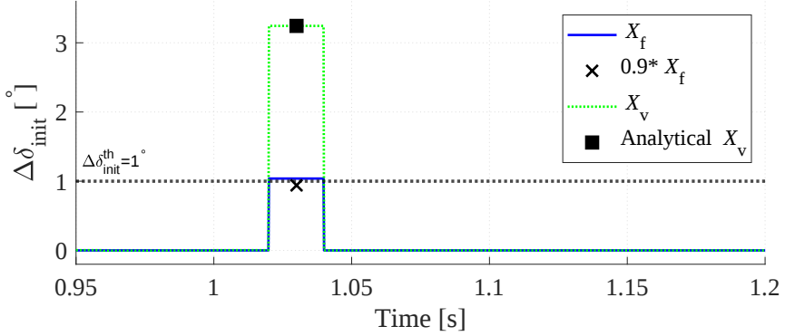
Figure 4.7: Cycle-to-cycle load angle jump for actual filter reactance ( X_f ), filter reactance with 10% error in parameter estimation, and virtual impedance for \Delta P_{vsm} = 12\% S_b
