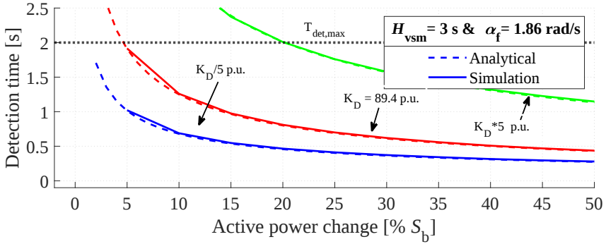
Figure 4.11: Detection time vs active power change for different values of K_D
