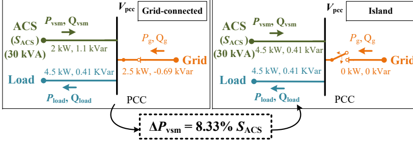
Figure 5.2: Power flow for MG lab setup to analyze the PQ-based vs dq-based load angle estimation before and after an islanding event
