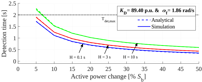
Figure 4.10: Detection time vs active power change for different values of H_{\text{vsm}}
