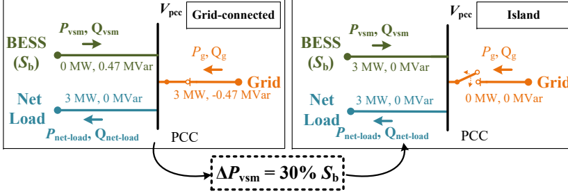
Figure 4.2: Power flow before and after island for the base case scenario. P_{net-load} = P_{load} - P_w = 10 \text{ MW} - 7 \text{ MW} = 3 \text{ MW} .
