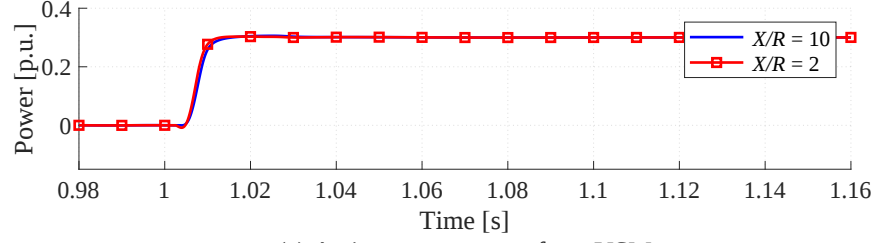
(a) Active power output from VSM
