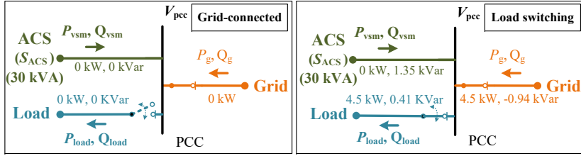
Figure 5.4: Power flow for MG laboratory setup to analyze the PQ-based vs dq-based load angle estimation in case of load switching
