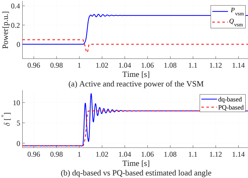
Figure 4.4: Comparison of PQ-based and dq-based estimation of load angle for implementing VVS-based IDM for \Delta P_{vsm} = 30\%S_b
