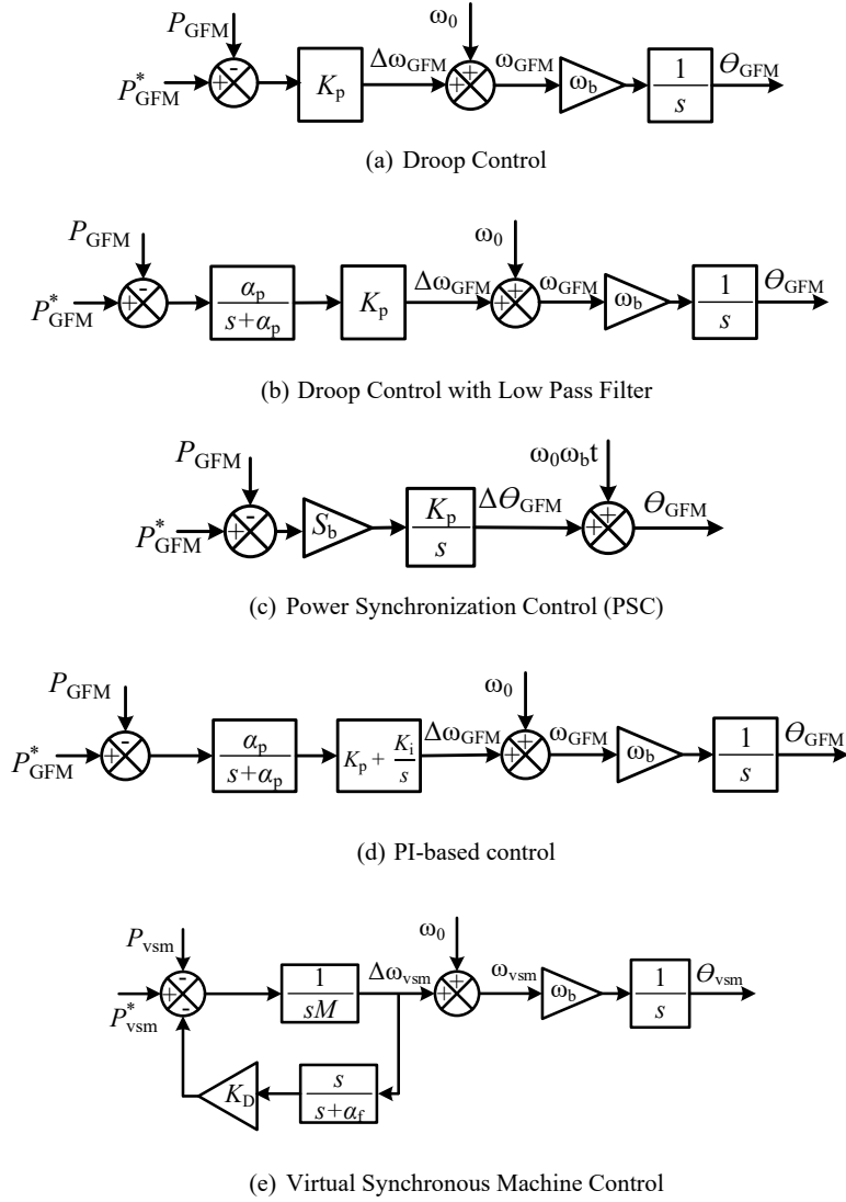
Figure 2.1: GFM control structures using active power based synchronization strategy
