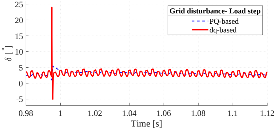
Figure 5.5: PQ-based vs dq-based load angle estimation for VVS-based island detection of an MG laboratory setup for \Delta P_{vsm} = 15\% S_{ACS} : load switching
