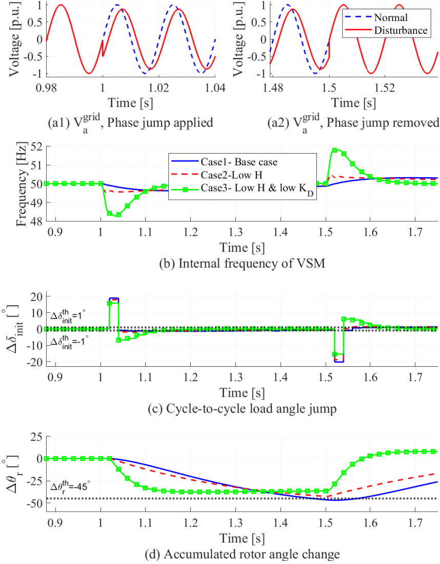
Figure 4.15: Impact of combined voltage dip and phase jump on the composite VVS-based island detection \Delta P_{\text{vsm}} = 25\%S_b . (Case 1- H_{\text{vsm}} = 3 s, K_D = 89.40 p.u., \alpha_f = 1.86 rad/s. Case 2- H_{\text{vsm}} = 0.1 s, K_D = 89.40 p.u., \alpha_f = 1.86 rad/s. Case 3- H_{\text{vsm}} = 0.1 s, K_D = 17.88 p.u., \alpha_f = 1.86 rad/s.)
