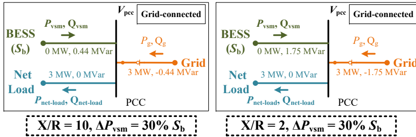
Figure 4.8: Power flows to analyze the impact of grid X/R ratio on VVS-based IDM
