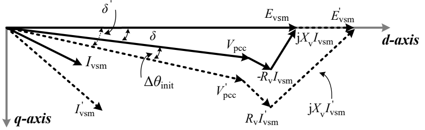
Figure 3.1: Initial angle jump of PCC voltage right after the islanding event
