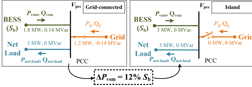
Figure 4.6: Power flows before and after the island to study the impact of parameter estimation error on \Delta\delta_{init} . P_{net-load} = P_{load} - P_w = 10 MW - 7 MW = 3 MW.
