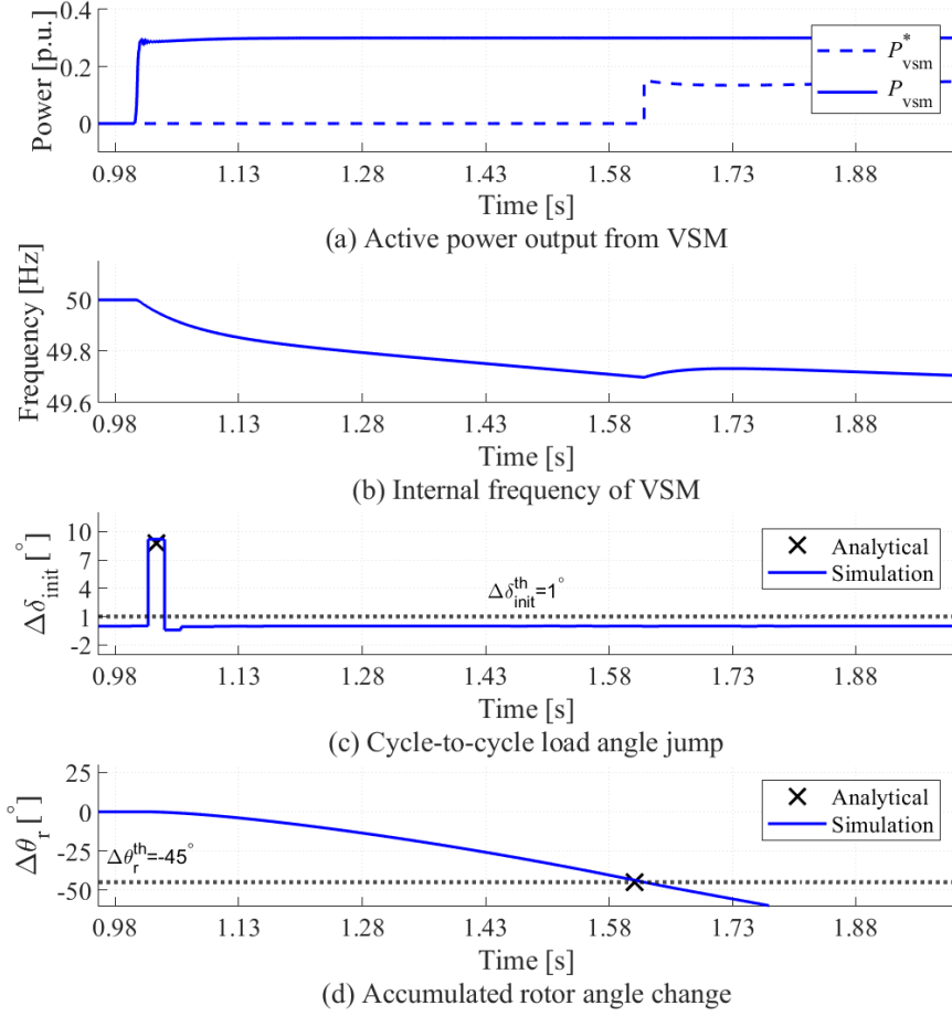
Figure 4.3: Unplanned island on the microgrid for \Delta P_{\text{vsm}} = 30\% S_b
