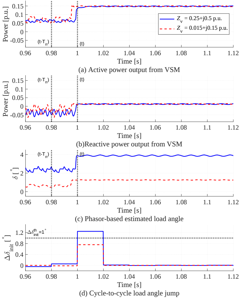
Figure 5.6: Island case: Impact of change of virtual impedance on the non-detection zone of VVS-based island detection for \Delta P_{vsm} = 8.33\% S_{ACS}
