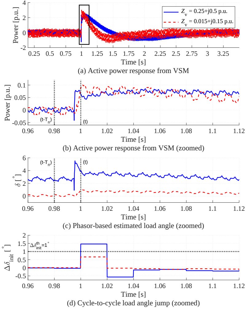
Figure 5.7: Misdetction by VVS-based island detection during a load switching event for \Delta P_{vsm} = 15\% S_{ACS} and two different values of virtual impedance
