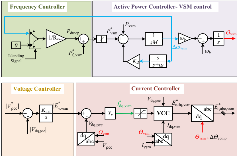
Figure 2.2: Block diagram of controllers for VSM
