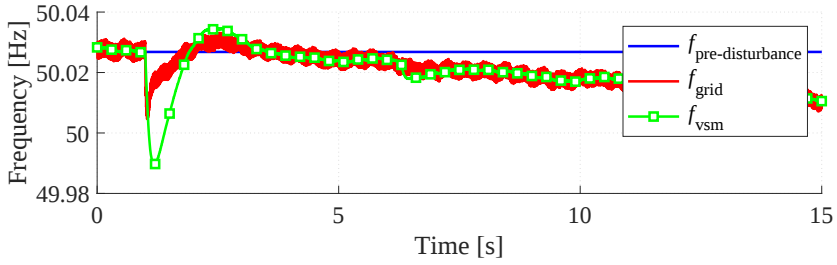
(a) Measured grid frequency and internal VSM frequency
