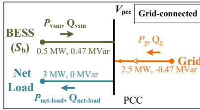
Figure 4.13: Power flows to analyze the risk of misdetection for grid frequency variation and grid voltage phase angle jump
