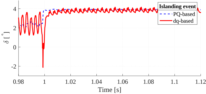
Figure 5.3: PQ-based vs dq-based load angle estimation for VVS-based island detection of MG laboratory setup for \Delta P_{vsm} = 8.33\% S_{ACS} during an islanding event
