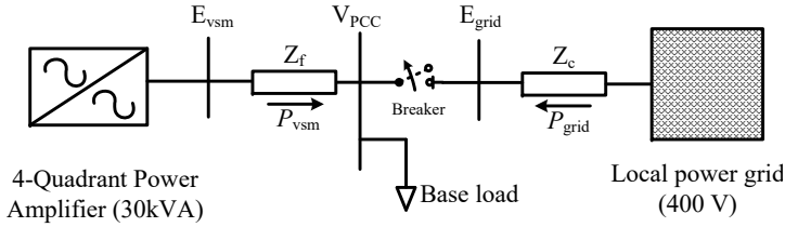
Figure 5.1: Lab setup for evaluating the performance of composite island detection method in an MG powered by a grid-forming inverter
