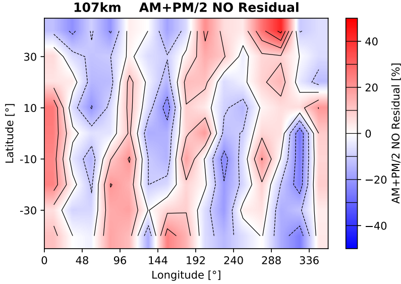
Figure 3.3: December monthly climatology of lower thermospheric SMR average pairs of ascending and descending NO measurements, taken between -40^\circ - +40^\circ latitude at 107 km altitude. The colors represent the deviation in percentage from the zonal mean, also known as residual. The effect of a semidiurnal solar nonmigrating tide on NO mixing ratio is visible in the 4-wave like structure. From Paper 4.
