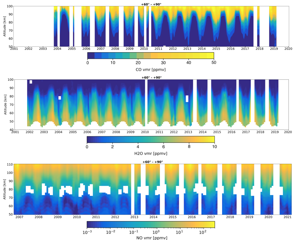
Figure 3.1: Time series of CO (top), H 2 O (middle) and NO (bottom) volume mixing ratios measured by SMR for the +60° – +90° latitude band, taken from Paper 1, 2 and 3 respectively. The white bands indicate months during which the number of scans in the given latitude band is lower than 10. The ticks on the x-axis correspond to the beginning of each year. Note the different colour scales and axes.
