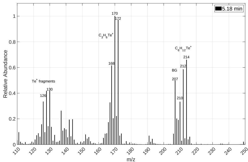
Figure 5.10. Mass spectrum for the irradiated sample containing texanol and \text{TeO}_2 for a peak with retention time 5.18 minutes
