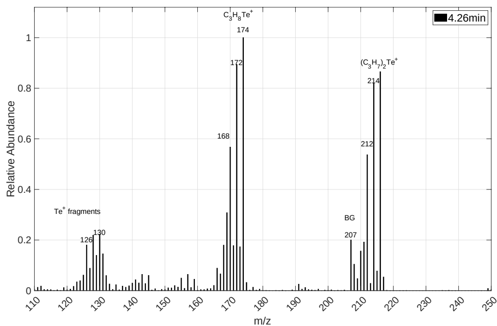
Figure 5.9. Mass spectrum for the irradiated sample containing texanol and \text{TeO}_2 for a peak with retention time 4.26 minutes. Mass at 207 m/z , denoted with BG, is a background signal
