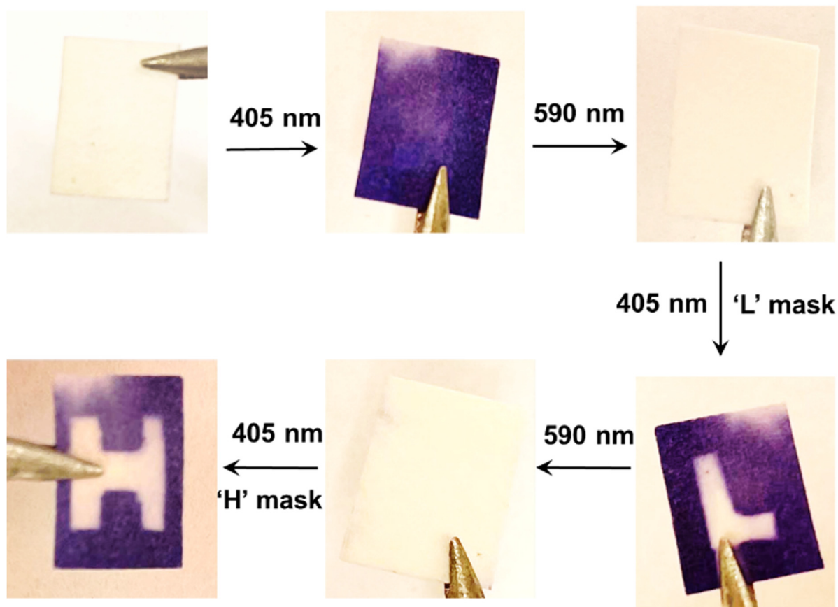
Fig. 6 All-visible-light switching in the solid state. Images of a filter paper prepared from CdS, 3-PCA and DAE2 solution, and its subsequent color (white and purple) and pattern change ('L' shape and 'H' shape), upon visible light irradiation by simply varying the wavelength between 405 nm and 590 nm in a normal atmospheric environment.
